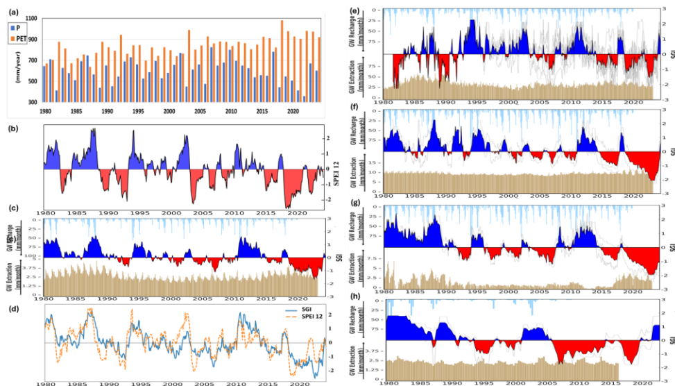
Figure 45. Hydroclimatic and groundwater drought dynamics (1980–2024). (a) Time series of Precipitation (P) and Potential Evapotranspiration (PET). (b) SPEI time series for the entire catchment. (c) SGI time series for the entire catchment. (d) Joint SPEI-12 and SGI comparison illustrating the strong co-variation between annual-scale hydroclimatic anomalies and groundwater-level variations storage response. (e) and (f) SGI time series of highly stressed sub-catchments. (g) and (h) SGI time series of moderately stressed sub-catchments, showing the spatial variability in drought response.
