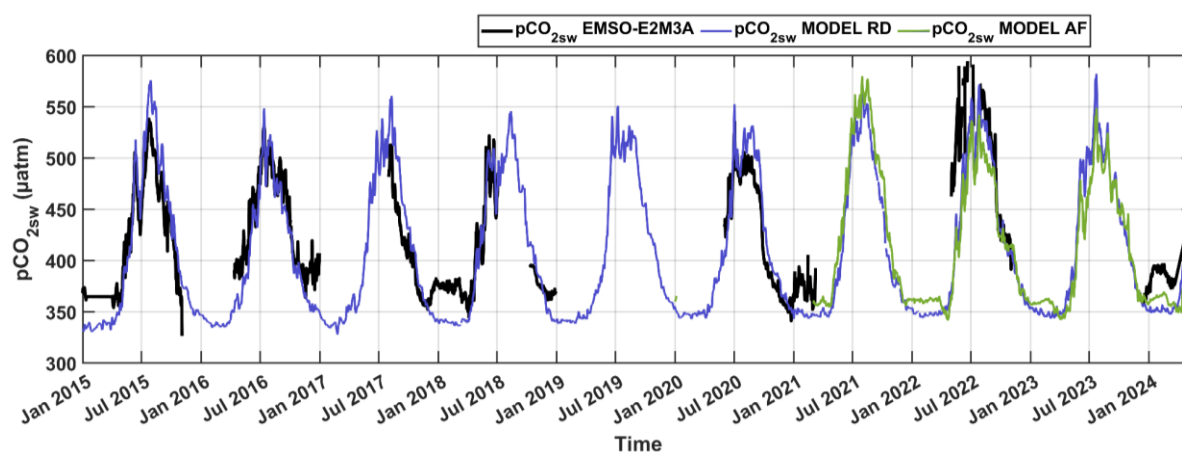
Figure 5. Time series of daily p\text{CO}_{2\text{sw}} ( \mu\text{atm} ) measured at the EMSO-E2M3A regional observatory in black, p\text{CO}_{2\text{sw}} ( \mu\text{atm} ) from the Mediterranean Sea Biogeochemistry Reanalysis (RD) in blue and the Mediterranean Sea Biogeochemistry Analysis and Forecast (AF) in green. RD data after July 2022 were integrated with the interim reanalysis.
