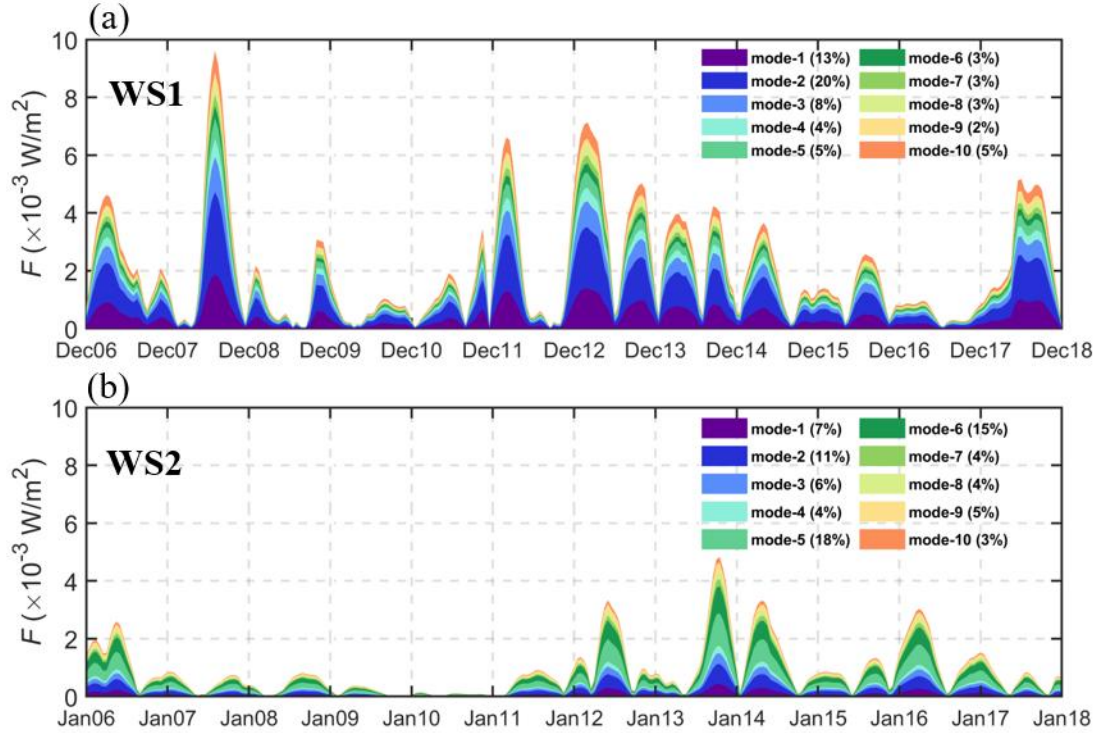
380 Figure 12. Temporal variation of wind-generated near-inertial energy flux, F , projected onto the first 10 modes during WS1 (a) and WS2 (b).
