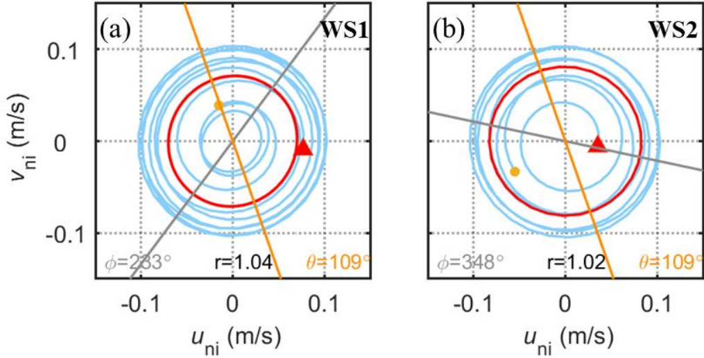
Figure 7. Depth-averaged near-inertial ellipses at the depth range of 70 m to 300 m during WS1 and WS2. The brown dot and red triangle indicate the beginning and end of ellipse, respectively. The red ellipse is obtained from the least squares fitting following Hebert and Moum (1994). The gray and orange lines represent the mean directions of the NIW propagation, \phi , and the background horizontal current, \theta , respectively. The ratio of major axis to minor axis of the near-inertial ellipse, r , is indicated in the corresponding panel.
