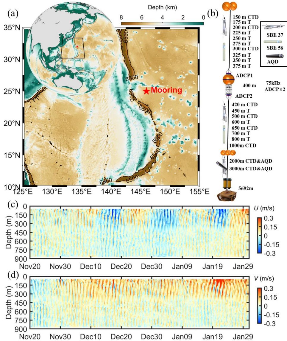
115 Figure 1. (a) Location of subsurface mooring (marked by a red pentagram), with color shading representing the topography. (b) Deployment depths of instruments on the subsurface mooring. (c) and (d) Depth-time plot of zonal and meridional velocities from 20 November 2017 to 31 January 2018.
