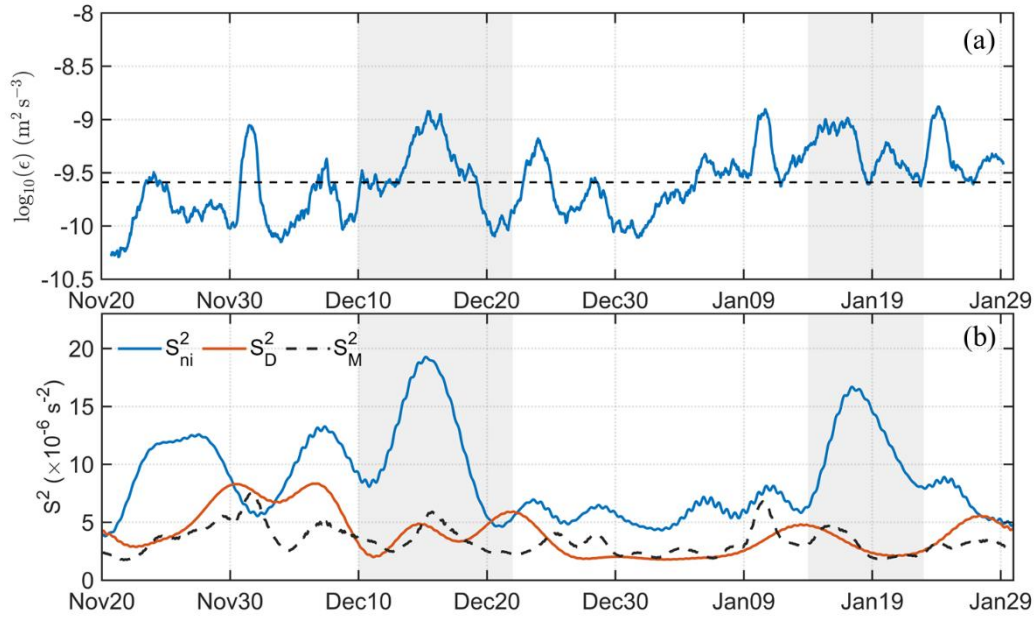
345 Figure 10. (a) Time series of the turbulent dissipation rate from GHP parameterization, during the observational period (50-300 m). The gray shading indicates the two NIW events. The horizontal dashed line denotes the time-averaged value. (b) Time series of vertical shear variance of near-inertial, diurnal, and semidiurnal components.
