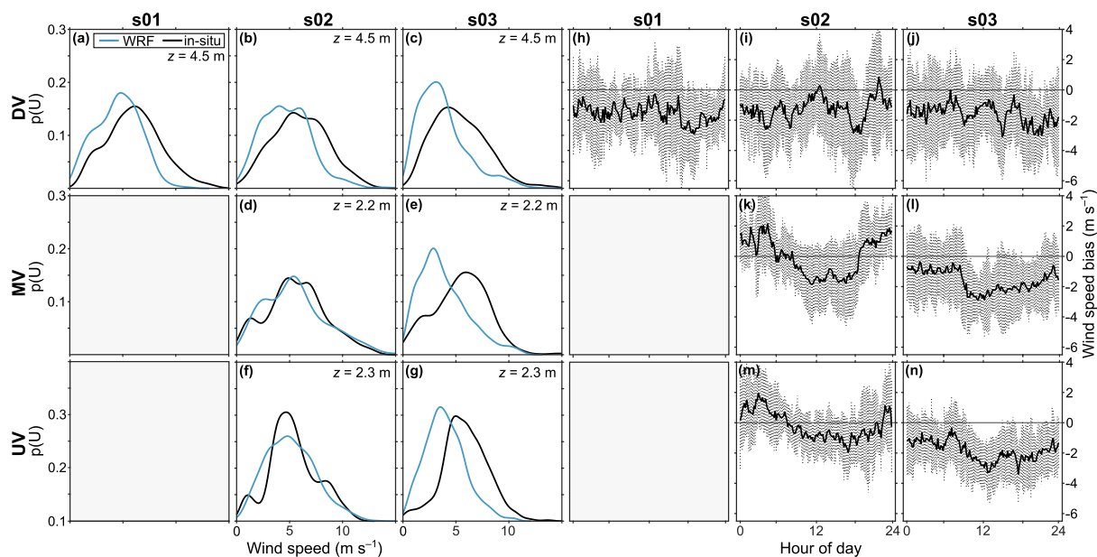
Figure 6. (a–g) Observed and simulated wind speed distributions at respective sensor height ( z ) for each simulation periods (s01: 2019 – 12 days; s02: 2021 – 11 days; s03: 2022 – 19 days). The s02 comparison only compares records from 24 June 2021– 3 July 2021 due to station data availability. (h–n) WRF wind speed bias vs. surface observations, shaded interval indicates 1\sigma .
