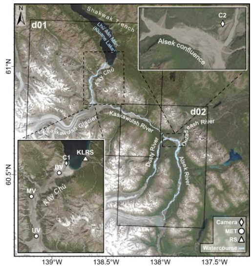
Figure 3. An overview of camera, MET (meteorological station) and RS (remote sensing) installations in the region. The two model domains (d01; d02) are indicated. Landsat 9 imagery (7 July 2023) courtesy of the U.S. Geological Survey.
