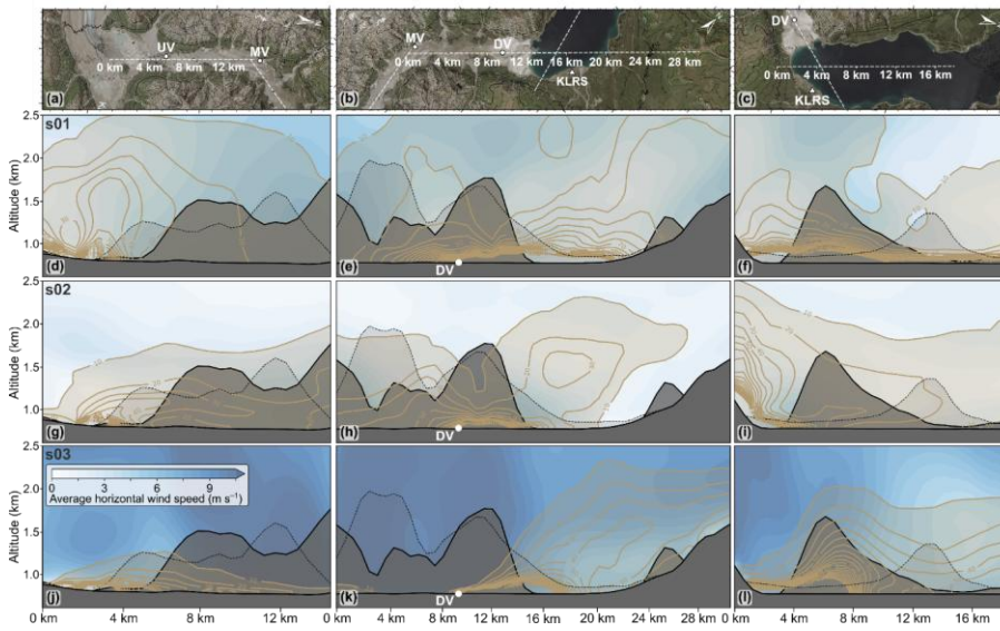
Figure 12. Cross sections of average horizontal wind speed and dust concentrations for (d–f) s01, (g–i) s02 and (j–l) s03. Contours range from 10–200 \mu\text{g m}^{-3} . Grey contouring indicates a parallel track of background valley sidewalls; (–) partial transparency indicates foreground topography (axis not to scale). Landsat 9 imagery (7 July 2023) courtesy of the U.S. Geological Survey.
