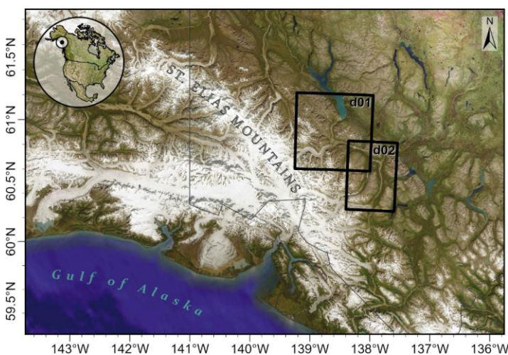
Figure 1. Overview of the study region and location of the two model domains (d01; d02). Basemap imagery courtesy of ESRI (2019).
