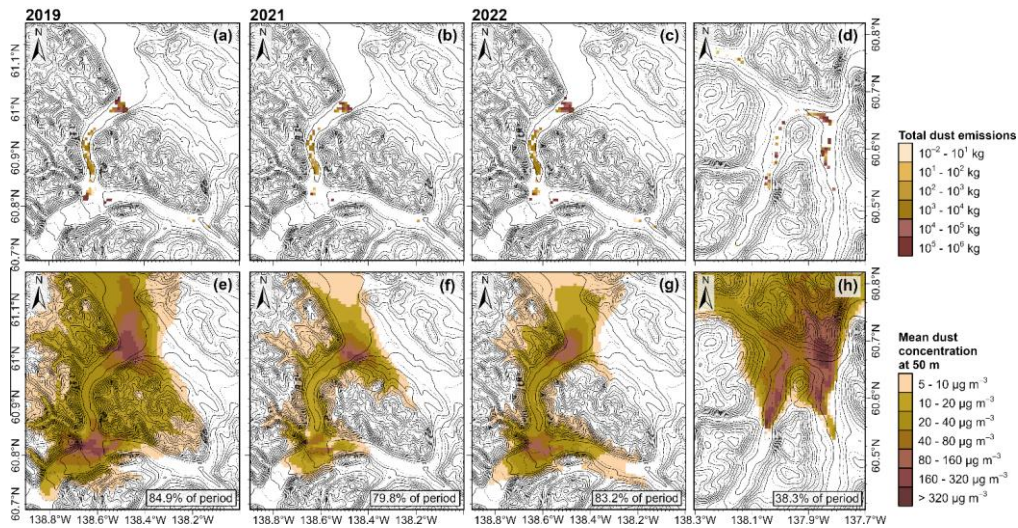
Figure 11. (top row) Summed dust (0.2 – 20.0 µm) emissions (kg) from 0.6 km 2 grid cells across simulation periods in d01 (a–c) and d02 (d). (bottom row) mean dust concentration at 50 m during active emission periods (non-zero emissions anywhere within domain) in d01 (e–g) and d02 (h). Percentage of period with active emissions indicated in each figure. Contours kriged from model topography.
