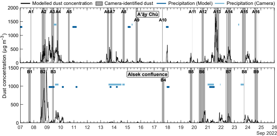
Figure 8. Dust observations and precipitation record derived from 10 min photography from C1 (A'ăy Chù) and C2 (Alsek confluence) during s03. Simulated dust concentration at 50 m was averaged for the area of the Alsek confluence covered by the viewshed of C2 (60.561–60.670°N, 137.772–137.855°W), and for the A'ăy Chù delta covered by C1 viewshed (60.988–61.022°N, 138.446–138.553°W). Simulated precipitation index indicates precipitation \geq 0.1 \text{ mm h}^{-1} averaged over viewsheds.
