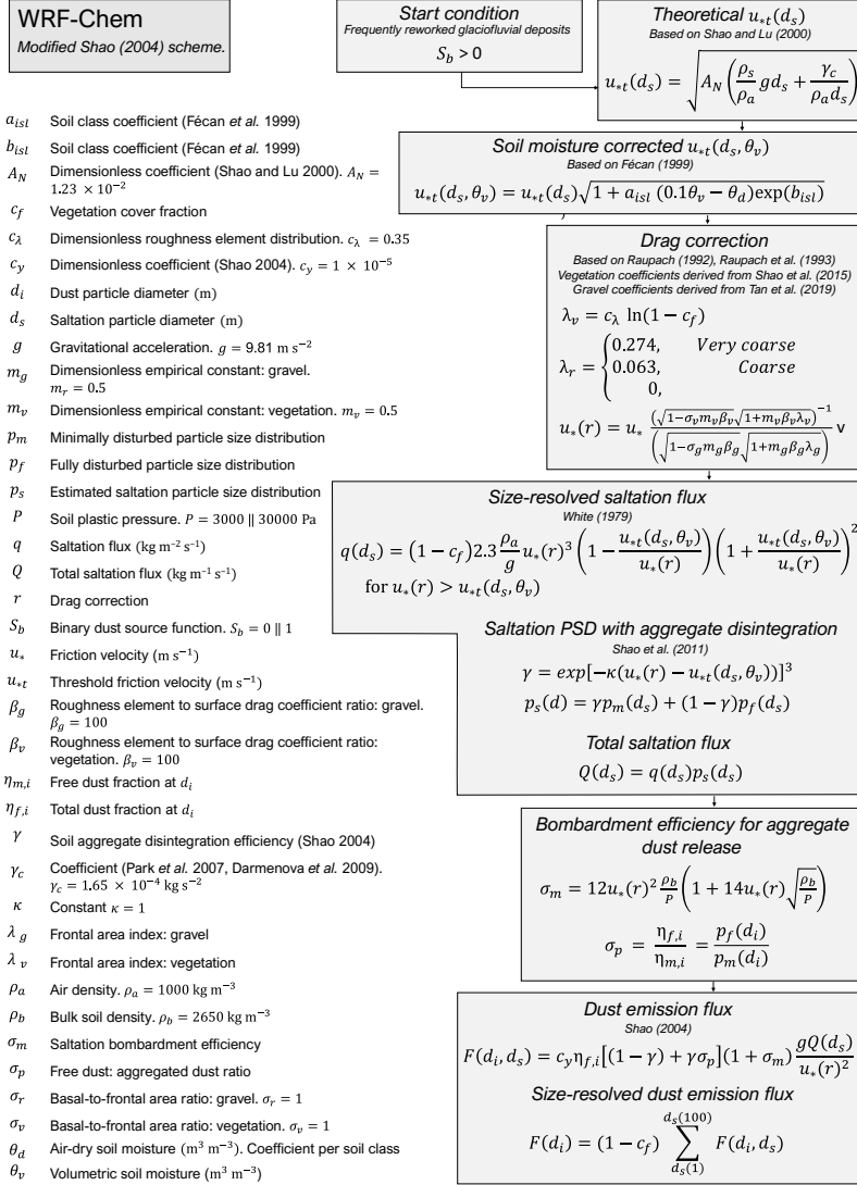
Figure 2. Overview of the modified Shao (2004) scheme in WRF-Chem developed in this work. Modifications were applied to the drag partition parameterisation ( \lambda_r, u_*(r) ), further are detailed in section 2.2.3.
