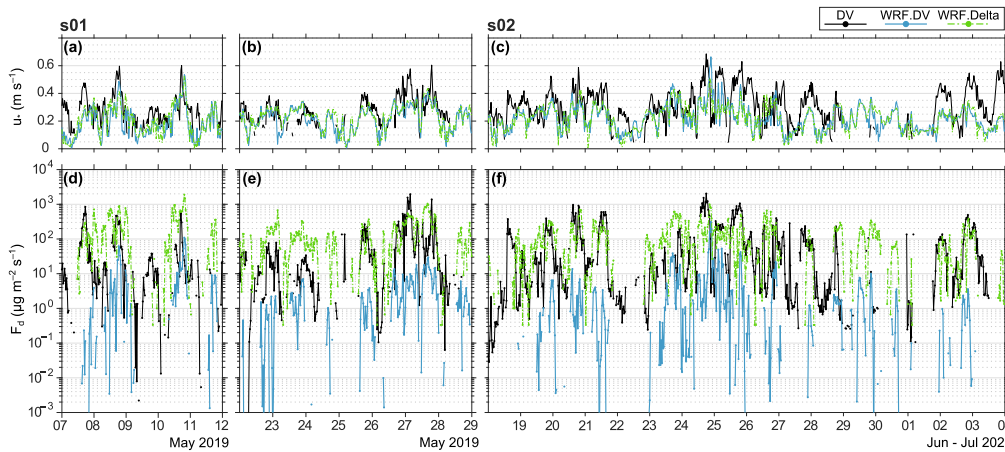
Figure 7. Comparison of measured (DV) and WRF-simulated variables: at the DV grid point (WRF.DV) and averaged over emissive grid cells of the A'ay Chù delta (WRF.Delta). (a-c) Friction velocity ( u_* ), (d-f) Vertical dust flux ( F_d ) (0.25 – 9.81 \mu\text{m} ).
