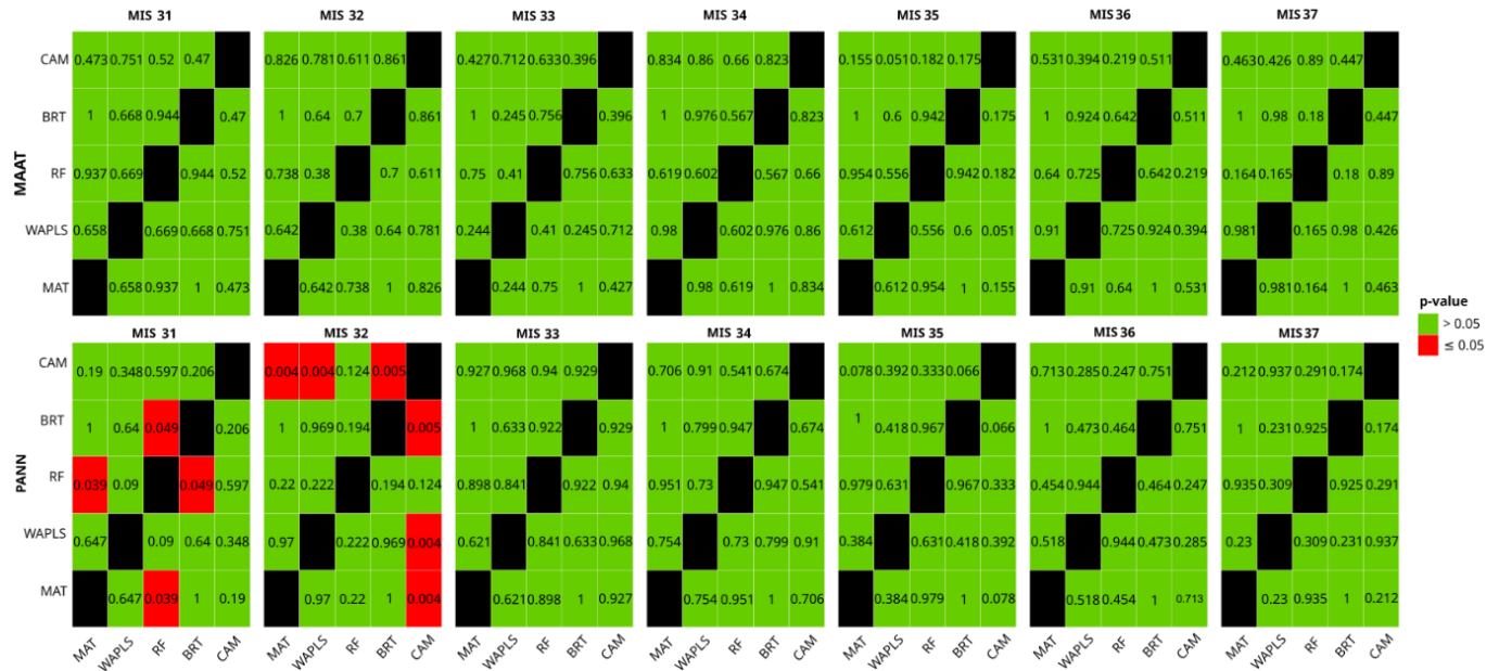
385 Figure 5. PERMANOVA p-values between climate reconstruction methods for each isotopic stage and for Mean Annual 386 Air Temperature (MAAT) and Mean of Annual Precipitation (PANN). A p-value less than or equal to 0.05 is significant 387 and indicates that the two methods are different from each other.
