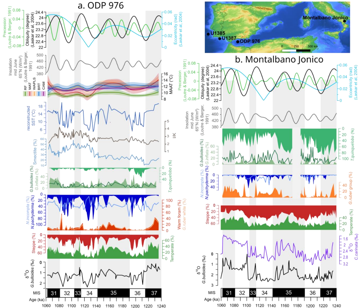
Figure 8. Land-sea variability comparison at ODP site 976 (left), compared to the site of Montalbano Jonico (right) in southern Italy. Isotope data for the ODP site 976 are from Catrain et al. (2025). For the Montalbano Jonico site, pollen and oxygen isotope data come from Joannin et al. (2008), and planktonic foraminifera data from Girone et al. (2013).
