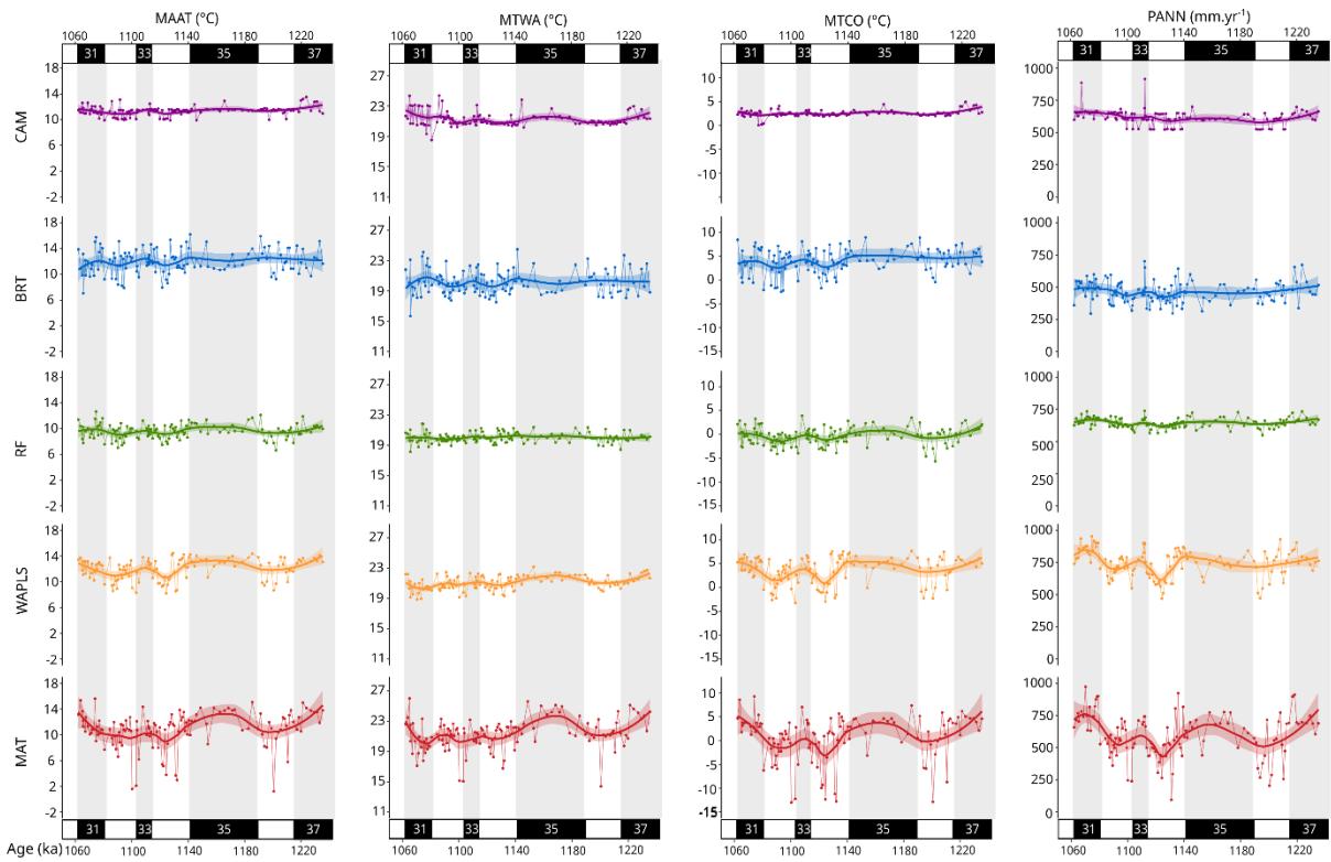
Figure 4. ODP site 976 pollen climate reconstruction. In green, RF (Random Forest), in blue BRT (Boosted Regression Trees), in yellow WAPLS (Weighted Averaging Partial Least Squares regression), in red MAT (Modern Analogue Technique) and in purple CAM (Climatic Amplitude Method). Four climatic parameters: MAAT (Mean Annual air Temperature), MTWA (Mean Temperature of the Warmest month), MTCO (Mean Temperature of the Coldest month) and PANN (mean annual precipitation). Grey bands correspond to interglacial periods and the thick coloured lines correspond to loess-smoothed curves and shaded areas to the 95 % confidence interval.
