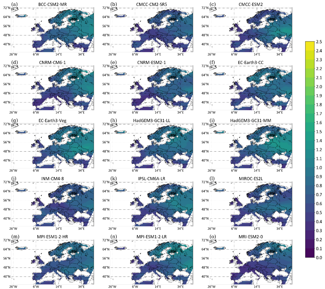
Figure S3: Yearly ICV estimates based on HS2009 method from each model of CMIP6 simulation during the historical simulation (1971-2000).
