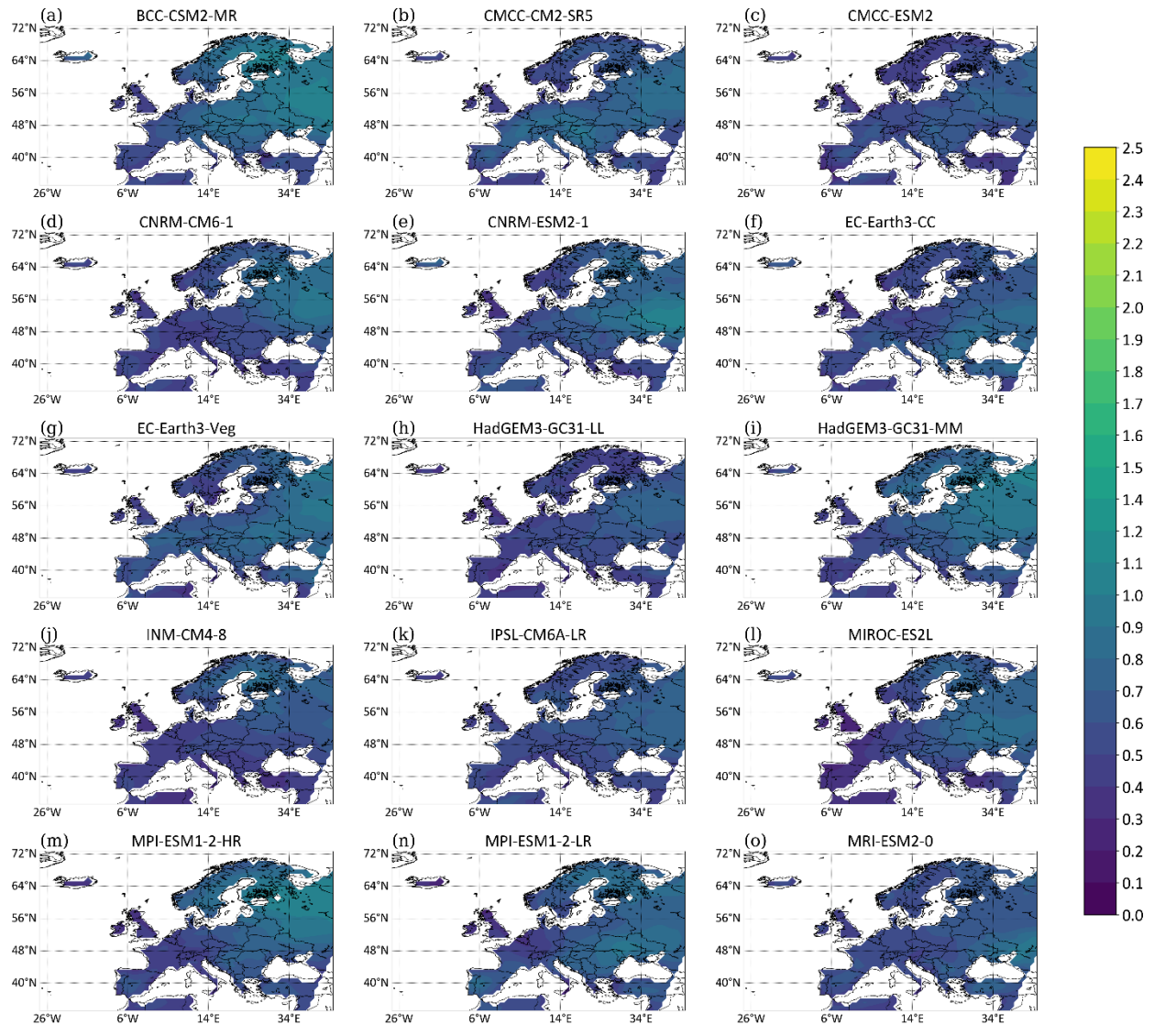
Figure S4: Same as Fig.S3 but for the period 2070-2099
