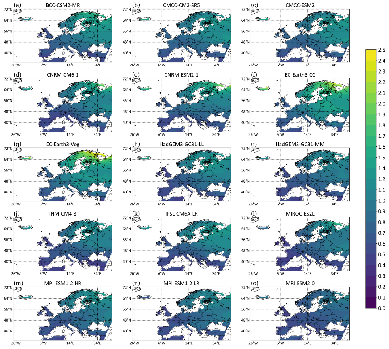
Figure S2: Yearly ICV estimates from each of the model of Pidata
