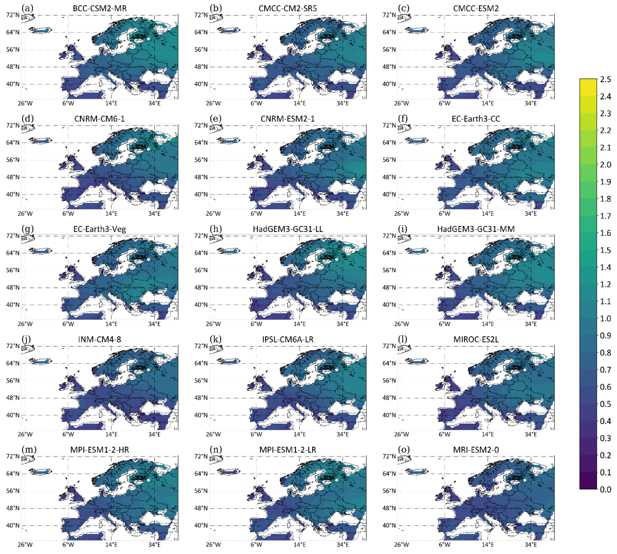
Figure S5: Same as Fig.S3 but for the period 1971-2100.
