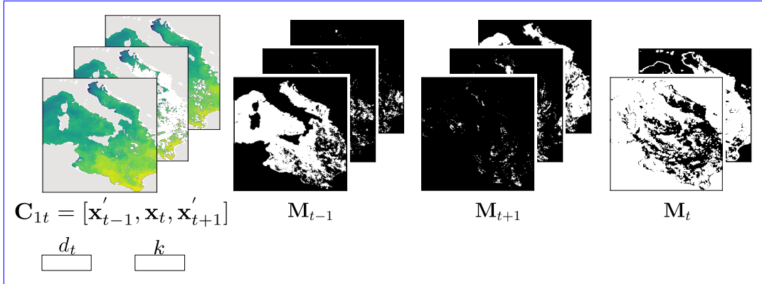
Figure 2. Context information fields provided to DIRECT at input. DIRECT uses a three-day SST window \mathbf{C}_{1t} = [\mathbf{x}'_{t-1}, \mathbf{x}_t, \mathbf{x}'_{t+1}] , with corresponding one-hot encoded masks \mathbf{M}_{t-1} and \mathbf{M}_{t+1} indicating the temporal origin of filled pixels, and \mathbf{M}_t marking observed versus missing values in the central frame. Additional conditioning is provided by the day-of-year ( d_t ) and the flow timestep k .
