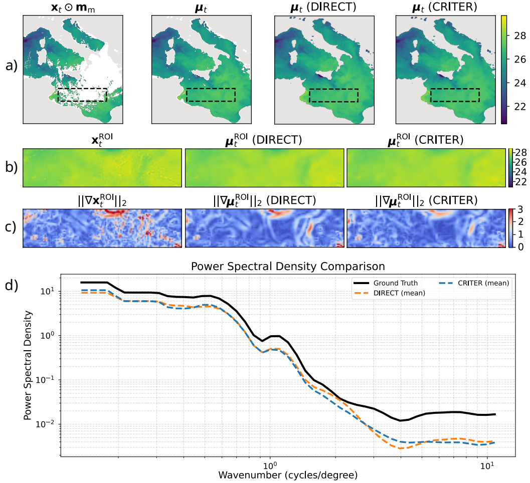
Figure 11. Power spectral density (PSD) analysis for a selected region of interest (ROI). Row-1:-a) masked SST input, ground truth field, and reconstructions from DIRECT and CRITER. Row-2:-b) zoomed views of the ROI. Row-3:-c) Gradient magnitudes \|\nabla \mu_t^{\text{ROI}}\|_2 highlighting structural differences. Row-4:-d) Isotropic PSD computed from the plane-detrended ROI fields using an FFT with Blackman-Harris-a Blackman-Harris window. The displayed curves represent the average spectral density across 10 independent mask realizations.
