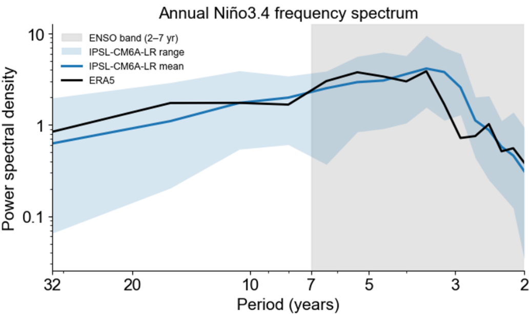
Figure A1: Power spectrum of the annual Niño3.4 index in ERA5 (black curve) and in the IPSL-CM6A-LR past2k simulations, computed over their common 1940–2014 period. The IPSL-CM6A-LR ensemble mean is shown by the blue curve, and the light-blue shading indicates the full range across ensemble members. The grey shading indicates the 2–7-year ENSO band.
