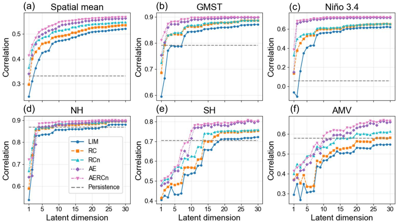
Figure 2: One-year lead forecast skill as a function of latent-space dimension. Correlation between emulator predictions and target surface temperature anomalies (500–1800 CE) is shown for (a) spatially averaged local scores, (b) GMST, (c) Niño3.4, (d) NH, (e) SH, and (f) AMV indices. The persistence benchmark is indicated by the dashed line.
