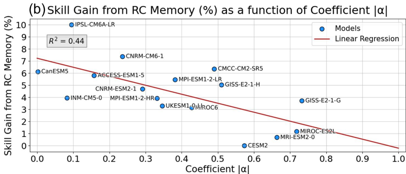
580 Figure 5: Skill gains attributed to reservoir computing (RC) memory and nonlinearities. Panel (a) shows the percentage improvement in spatially averaged tropical Pacific correlation relative to LIM across 16 CMIP6 models. Panel (b) presents the linear regression between memory-related skill gain and the nonlinearity indicator |\alpha| .
