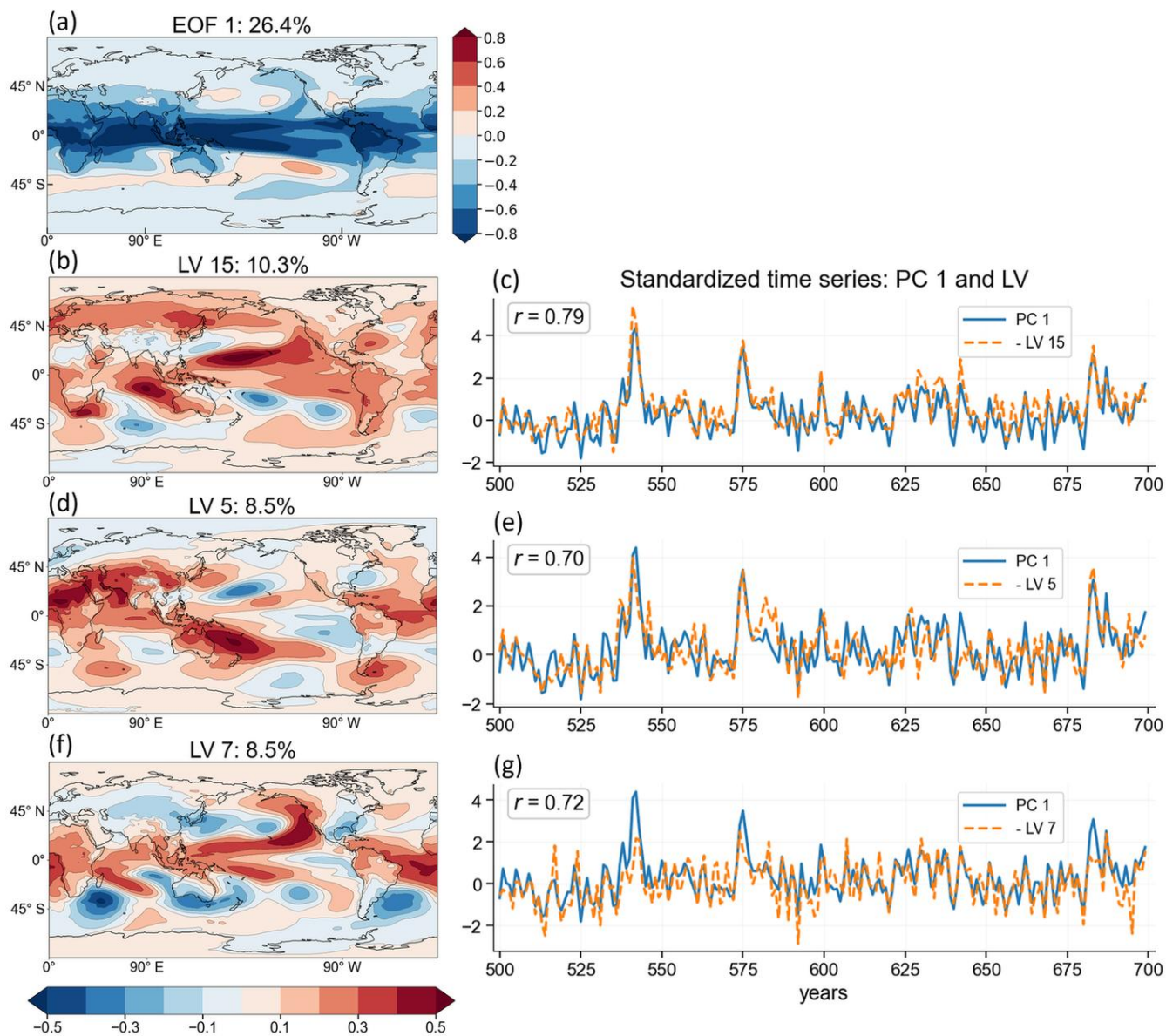
Figure A8: Variance structures associated with EOF1 within the 16-dimensional latent space. Panel (a) shows local variance explained by EOF1. Panels (b, d, f) display variance explained by selected AE latent vectors based on correlation \geq 0.7 with EOF1. Panels (c, e, g) show standardized time series over the first 200 years. Correlation coefficients are indicated.
