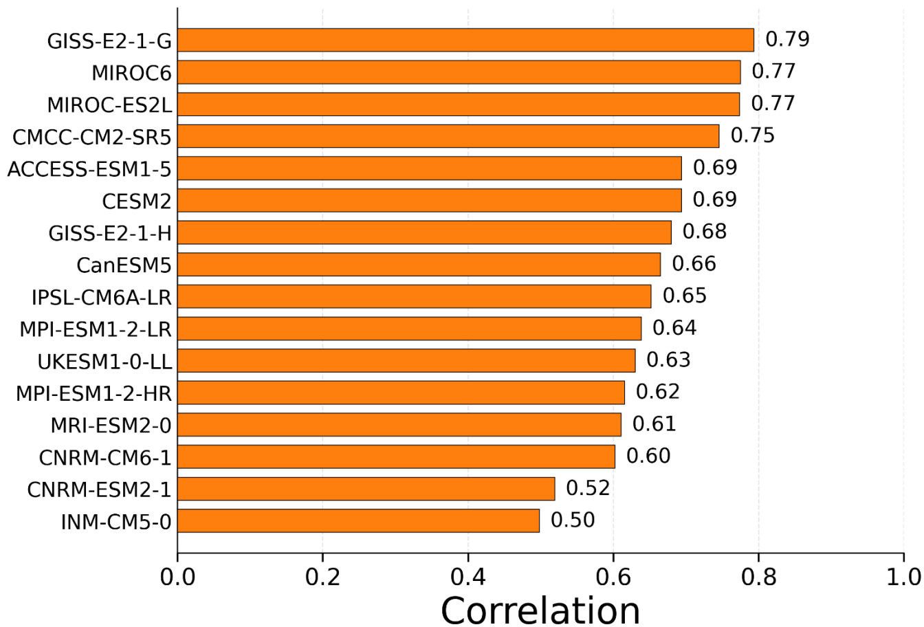
885 Figure A11: Spatially averaged tropical Pacific correlation at one-year lead time obtained using the RC emulator across 16 CMIP6 models. Models are ordered by decreasing skill.
