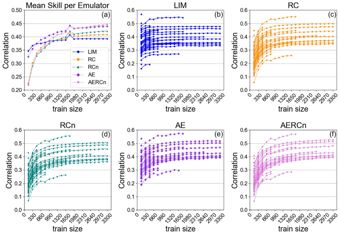
Figure 6: Sensitivity of forecast skill to training data length. Panel (a) shows the spatially averaged correlation as a function of training size (years), with one curve per emulator averaged across CMIP6 models. Panels (b–f) display model-specific results for LIM, RC, RCn, AE, and AERCn, with one curve per CMIP6 model.
