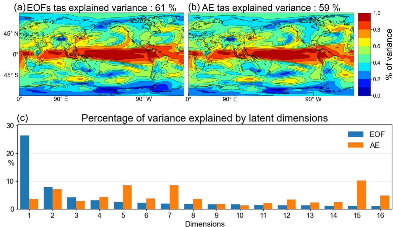
Figure A6: Spatial distribution of variance explained by latent representations of annual surface air temperature (tas) anomaly fields from the IPSL-CM6A-LR past2k ensemble. Panels (a) and (b) show the variance explained by a 16-dimensional latent space constructed using EOFs and AE latent vectors, respectively. Panel (c) presents the fractional variance contribution associated with each latent dimension.
