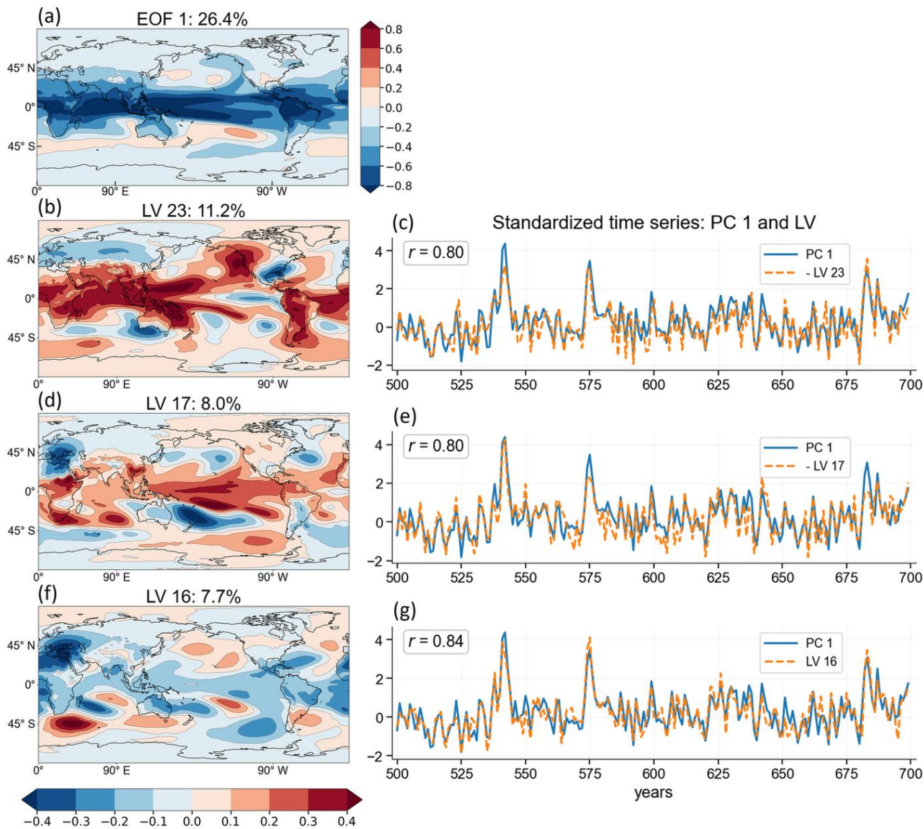
Figure A4: Variance structures associated with EOF1 and AE latent vectors using a 30-dimensional latent space. Panel (a) shows the local variance explained by EOF1. The spatial patterns are dimensionless, as the EOF analysis is performed on the normalized covariance matrix. Panels (b, d, f) display variance explained by AE latent vectors selected based on correlation \geq 0.7 with EOF1. Panels (c, e, g) show the corresponding standardized time series over the first 200 years. Correlation coefficients are indicated.
