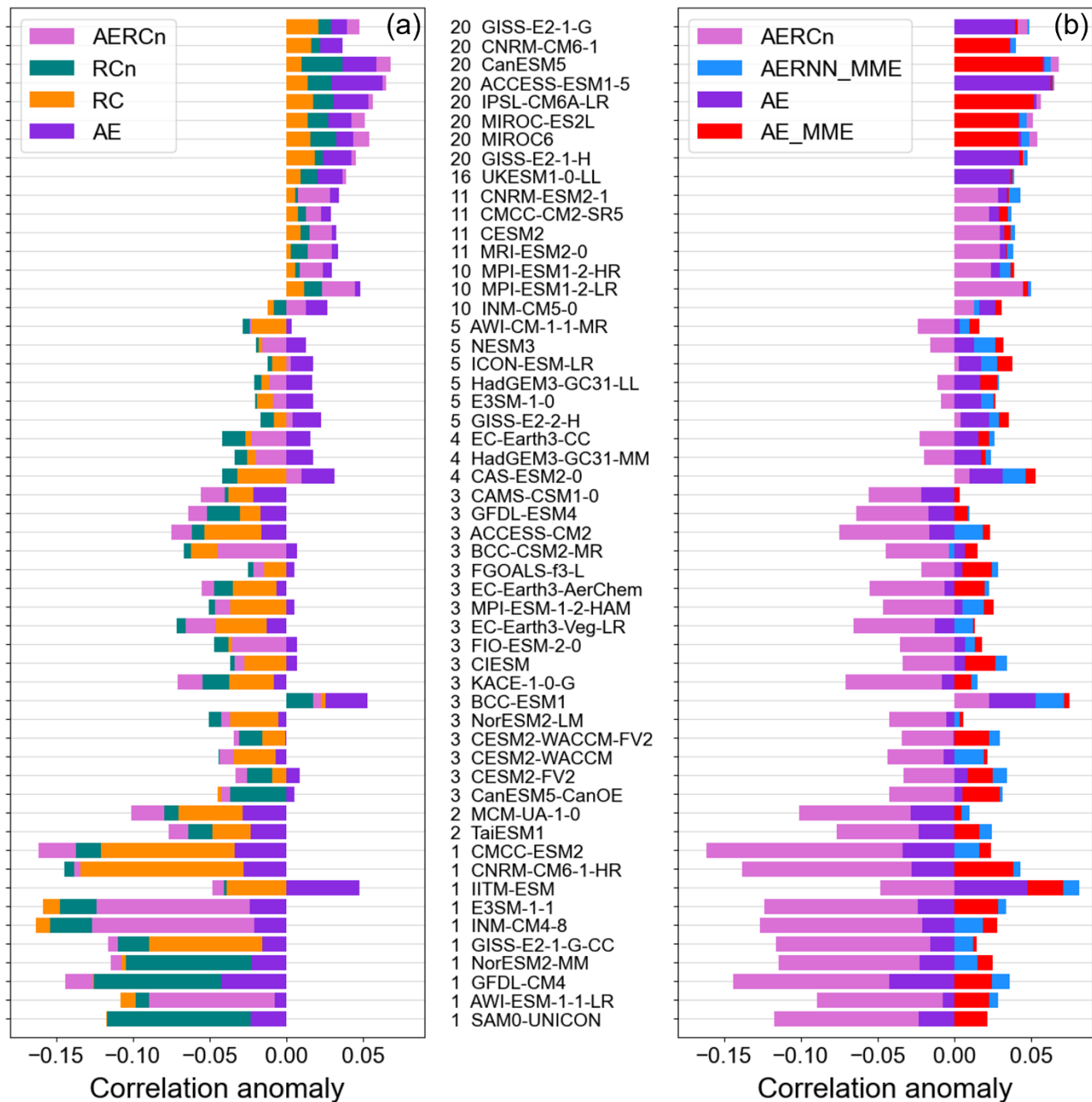
Figure A12: Emulator skill gain relative to LIM across 52 CMIP6 models. Panel (a) shows anomalies in spatially averaged correlation for AERCn, RCn, RC, and AE relative to LIM. Panel (b) shows skill differences for AE, AERCn, and their multimodel pretrained variants. Models are ordered according to training-set size, defined as the number of available historical ensemble members, which is indicated in the central panel.
