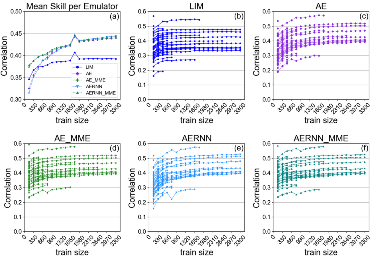
620 Figure 7: Impact of transfer learning on forecast skill. (a) Spatially averaged correlation is shown for LIM, AE, AE_MME, AERNN, and AERNN_MME configurations across CMIP6 models as a function of training size (years), with one curve per emulator. Panels (b–f) show model-specific results, with one curve per CMIP6 model.
