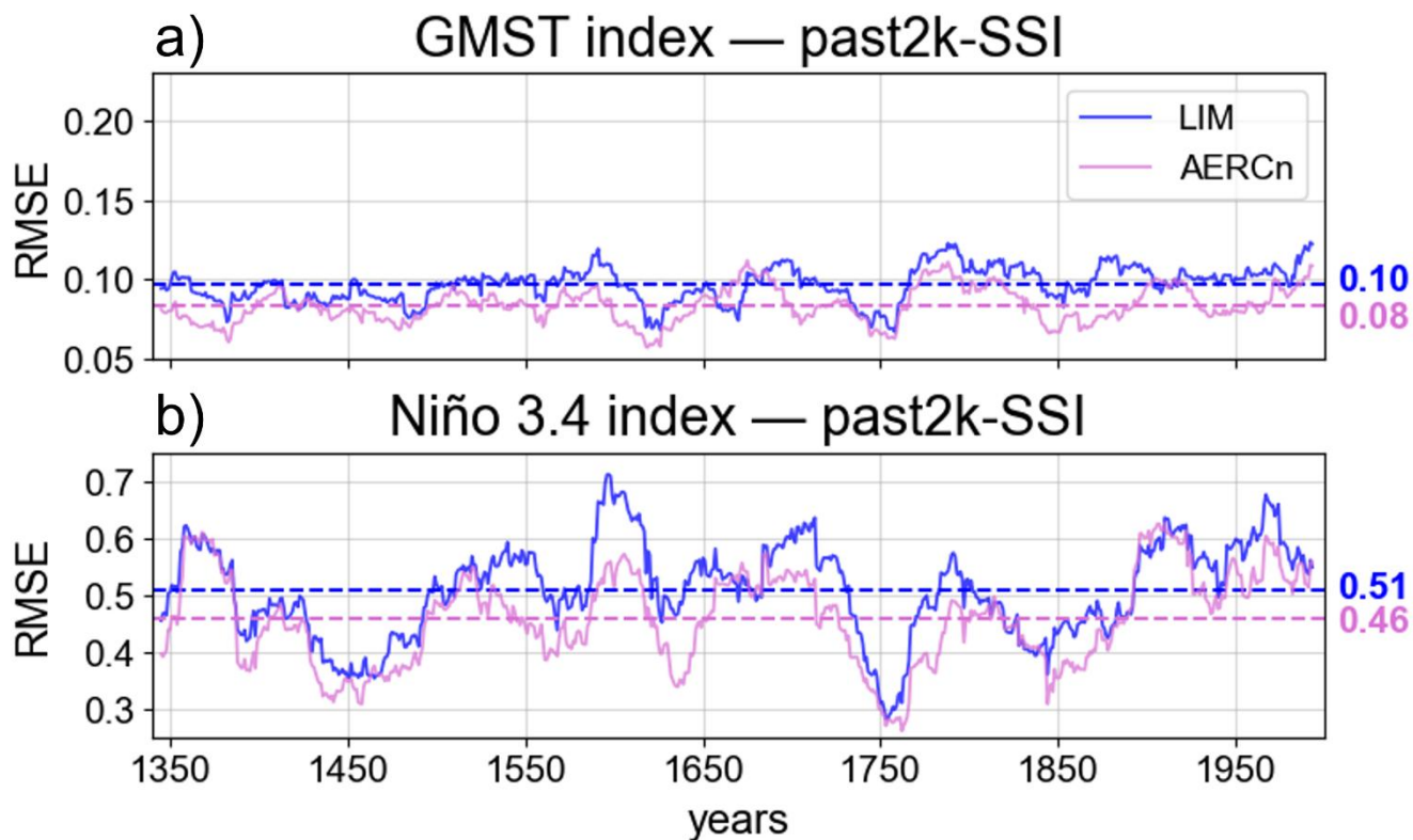
Figure A10: Temporal evolution of prediction error. Thirty-year rolling RMSE of one-year lead forecasts for LIM (blue) and AERCn (pink) is shown for (a) GMST and (b) Niño3.4 in the past2k-SSI experiment.
