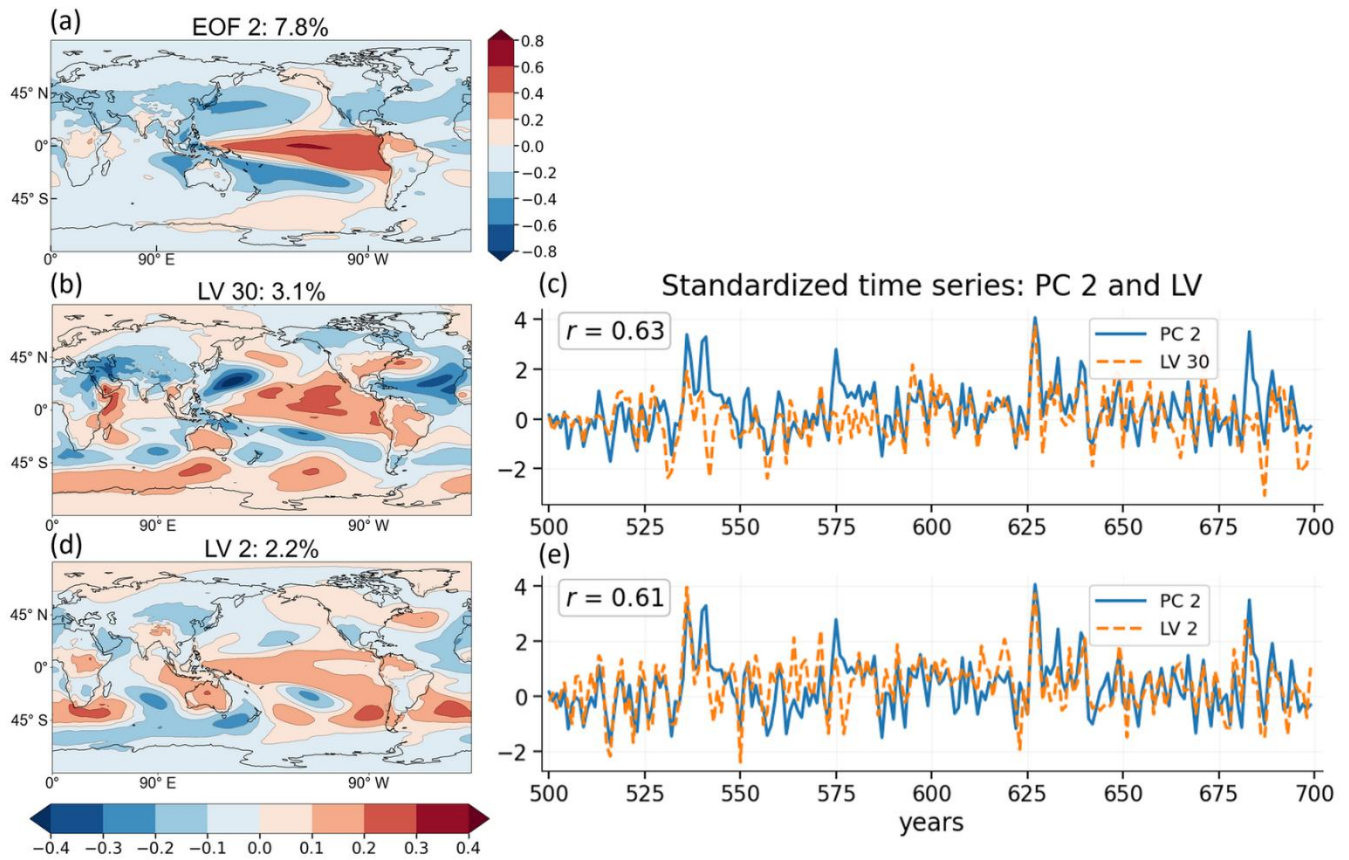
Figure A5: Variance structures associated with EOF2 and AE latent vectors using a 30-dimensional latent space. Panel (a) shows the local variance explained by EOF2. The spatial patterns are dimensionless, as the EOF analysis is performed on the normalized covariance matrix. Panels (b, d) display variance explained by AE latent vectors selected based on correlation \geq 0.6 with EOF2. Panels (c, e) show the corresponding standardized time series over the first 200 years. Correlation coefficients are indicated.
