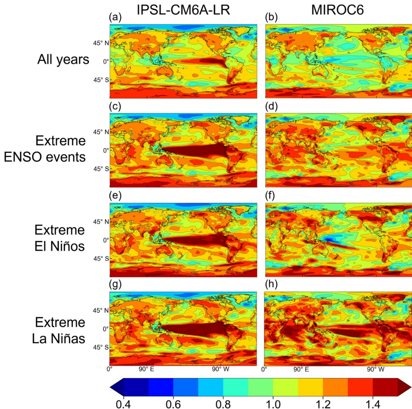
Figure A14: RMSE of one-year lead persistence forecasts with target piControl simulations during all years (a, b) extreme ENSO events (c,d), extreme El Niños (e,f) and extreme La Niñas (g,h). Results are shown for IPSL-CM6A-LR (left column) and MIROC6 (right column).
