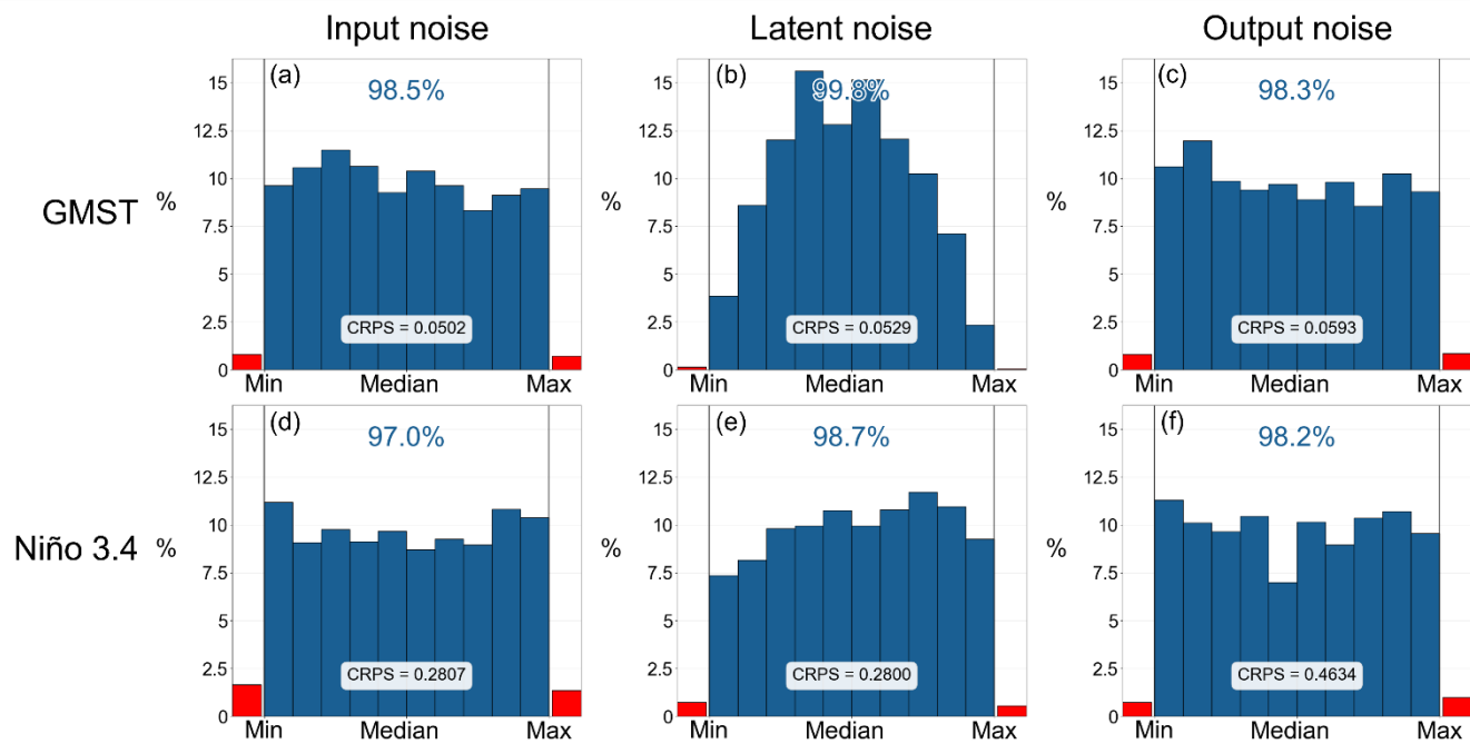
910 Figure A15: Reliability of AERCn ensemble forecasts generated with different perturbation strategies for IPSL-CM6A-LR. Rank histograms are shown for GMST (a–c) and Niño3.4 (d–f) using 100-member one-year lead ensembles. Columns correspond to input-space white-noise perturbations (left), latent-space white-noise perturbations (middle), and output-space noise based on the covariance of prediction errors (right). Blue bars indicate target frequency within ensemble deciles; red bars denote occurrences outside the ensemble spread. Percentages within the spread and mean CRPS values are indicated in each panel.
