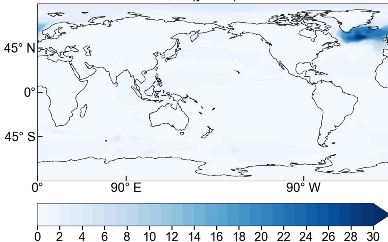
Figure A9: Decorrelation time of surface air temperature anomalies for IPSL-CM6A-LR, computed as the pointwise e-folding time of the autocorrelation function. Values are shown in years.
