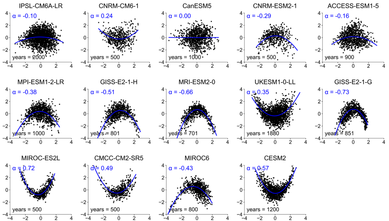
895 Figure A13: Phase-space representation of ENSO variability. Scatter plots of PC1 versus PC2 of DJF SST anomalies from CMIP6 piControl simulations are shown. The fitted quadratic curve provides the nonlinearity coefficient \alpha .
