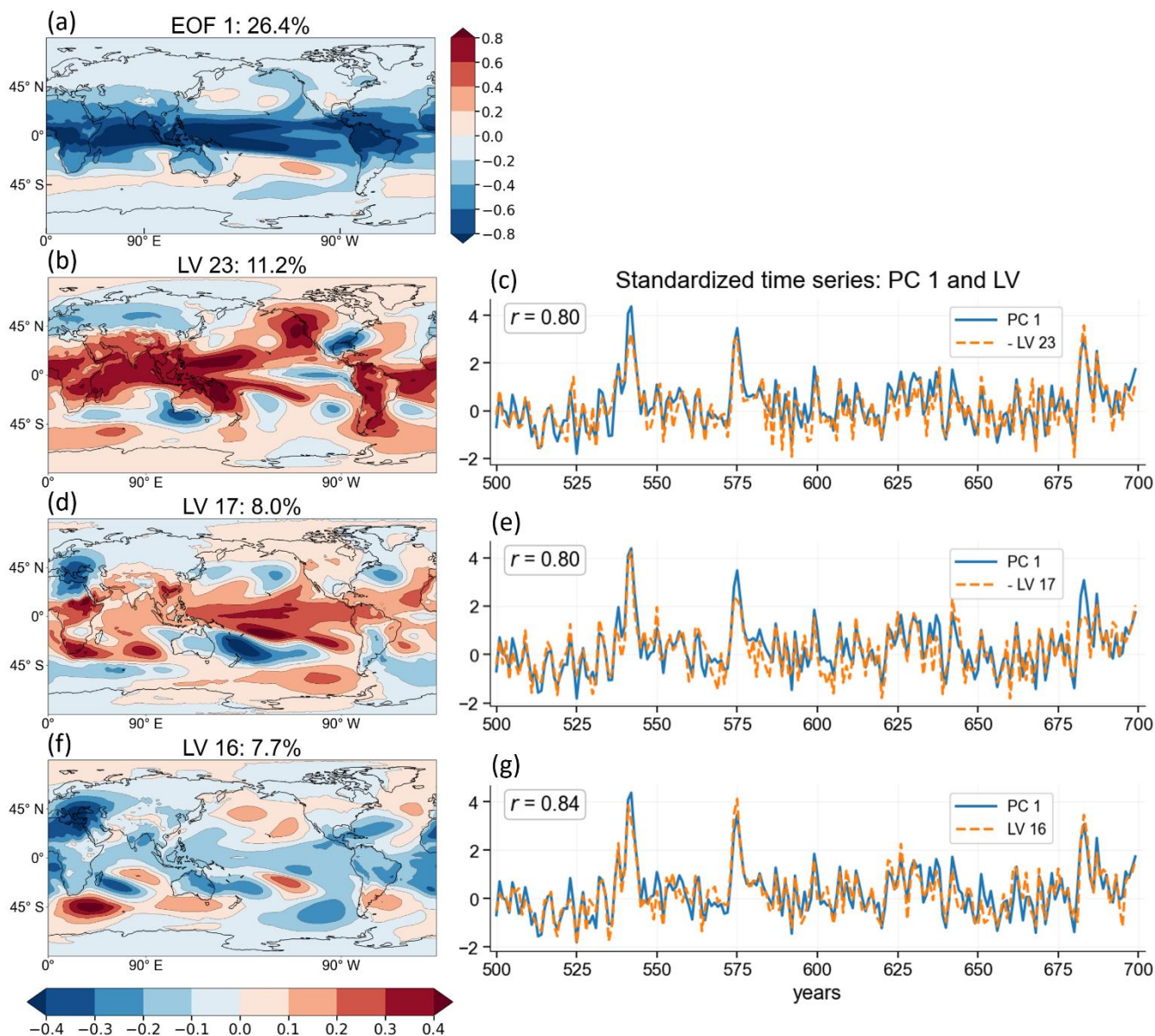
835 Figure A4: Variance structures associated with EOF1 and AE latent vectors using a 30-dimensional latent space. Panel (a) shows the local variance explained by EOF1. Panels (b, d, f) display variance explained by AE latent vectors selected based on correlation \geq 0.7 with EOF1. Panels (c, e, g) show the corresponding standardized time series over the first 200 years. Correlation coefficients are indicated.
