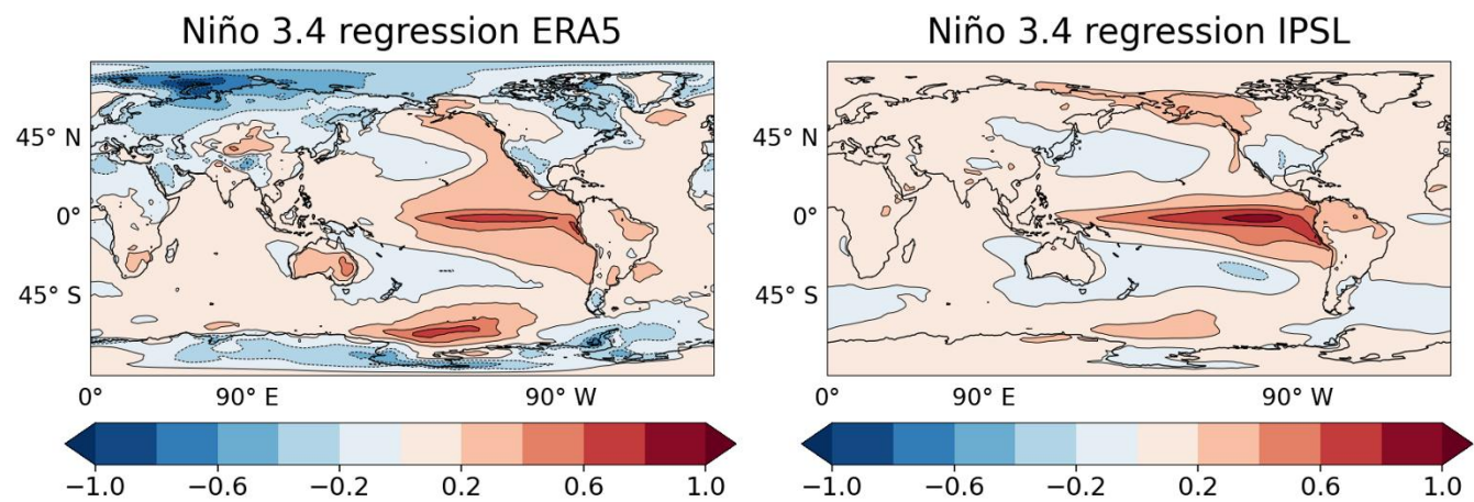
Figure A2: Regression maps of annual surface temperature anomalies onto the Niño3.4 index in ERA5 (left) and in the IPSL-CM6A-LR past2k simulations (right).
