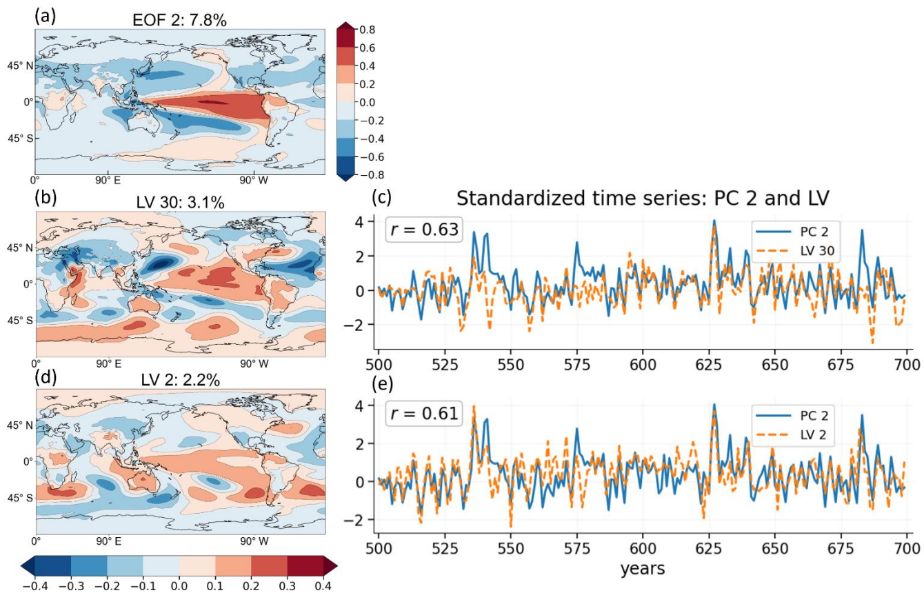
Figure A5: Variance structures associated with EOF2 and AE latent vectors using a 30-dimensional latent space. Panel (a) shows the local variance explained by EOF2. Panels (b, d) display variance explained by AE latent vectors selected based on correlation \geq 0.6 with EOF2. Panels (c, e) show the corresponding standardized time series over the first 200 years. Correlation coefficients are indicated.
