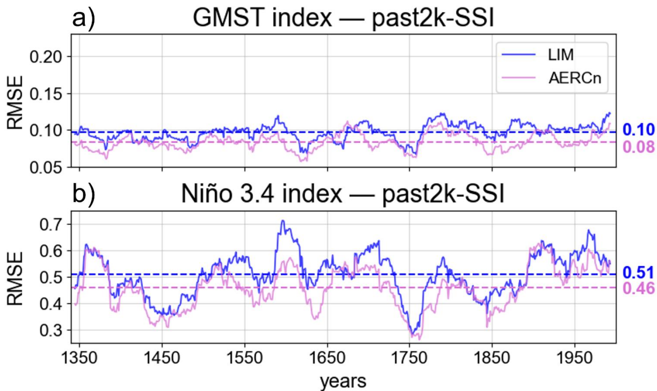
880 Figure A10: Temporal evolution of prediction error. Thirty-year rolling RMSE of one-year lead forecasts for LIM (blue) and AERCn (pink) is shown for (a) GMST and (b) Niño3.4 in the past2k-SSI experiment.
