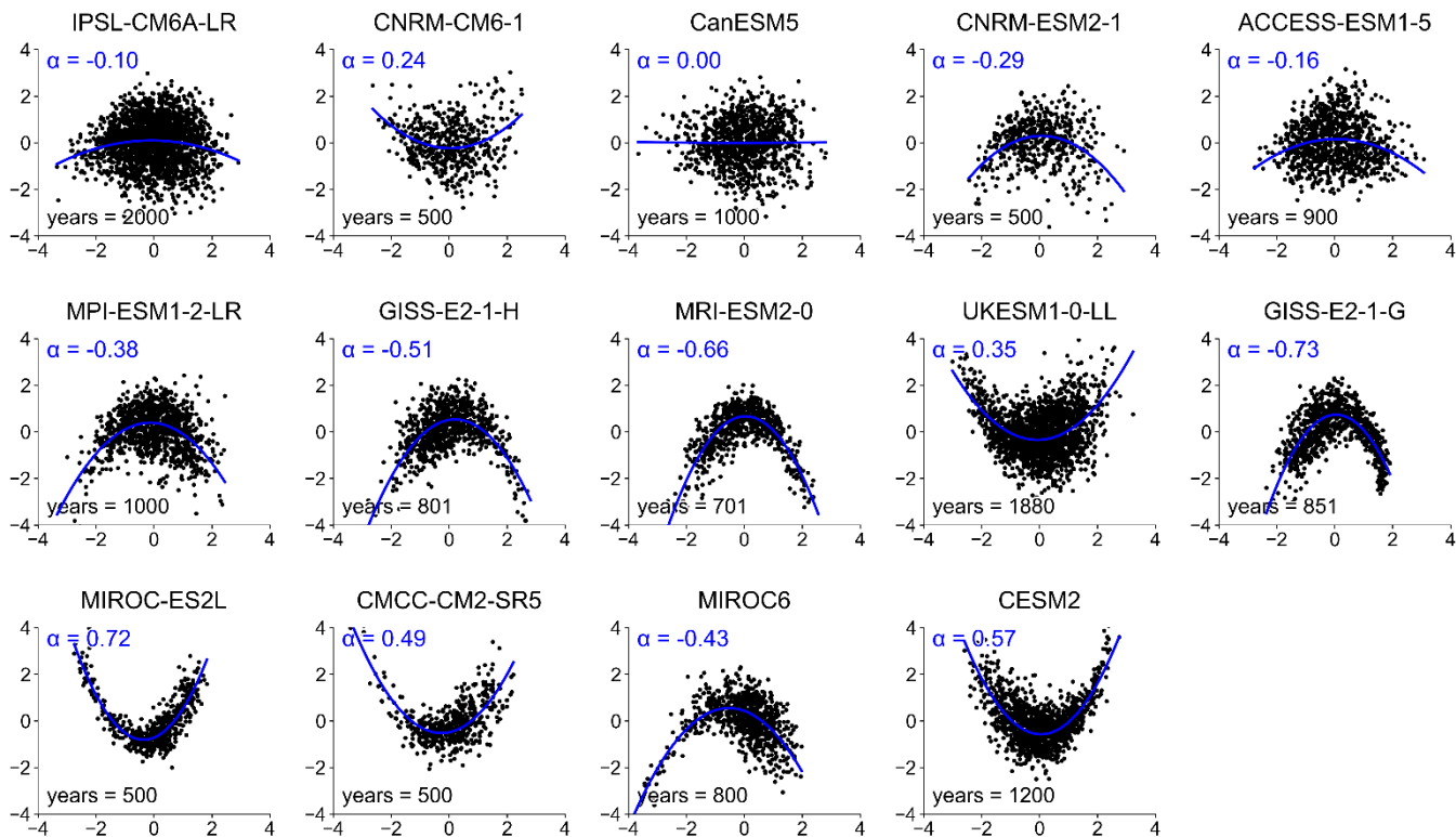
Figure A13: Phase-space representation of ENSO variability. Scatter plots of PC1 versus PC2 of DJF SST anomalies from CMIP6 piControl simulations are shown. The fitted quadratic curve provides the nonlinearity coefficient \alpha .
