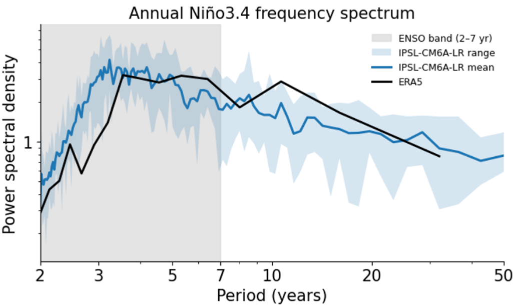
Figure A1: Power spectrum of the annual Niño3.4 index in ERA5 (black curve) and in the IPSL-CM6A-LR past2k simulations. The IPSL-CM6A-LR ensemble mean is shown by the blue curve, and the light-blue shading indicates the full range across ensemble members. The grey shading indicates the 2–7-year ENSO band.
