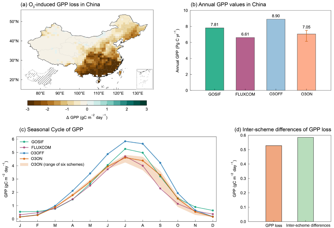
Figure 3. Simulated O_3 -induced vegetation damage and the inter-scheme differences in China. (a) Spatial distribution of O_3 -induced GPP loss averaged from all six parameterizations during the growing season (April-September). (b) National annual GPP from GOSIF and FLUXCOM benchmarks compared with simulations under O3OFF and O3ON conditions. The O3ON shows the average from six O_3 damage experiments, with the error bar indicating inter-scheme discrepancies. (c) Seasonal cycle of GPP in China, with shading indicating the range across the six O_3 damage schemes. (d) Comparison between averaged GPP loss and inter-scheme differences of the simulations. The inter-scheme difference is defined as the range across the six parameterizations, calculated as the difference between the maximum and minimum values.
