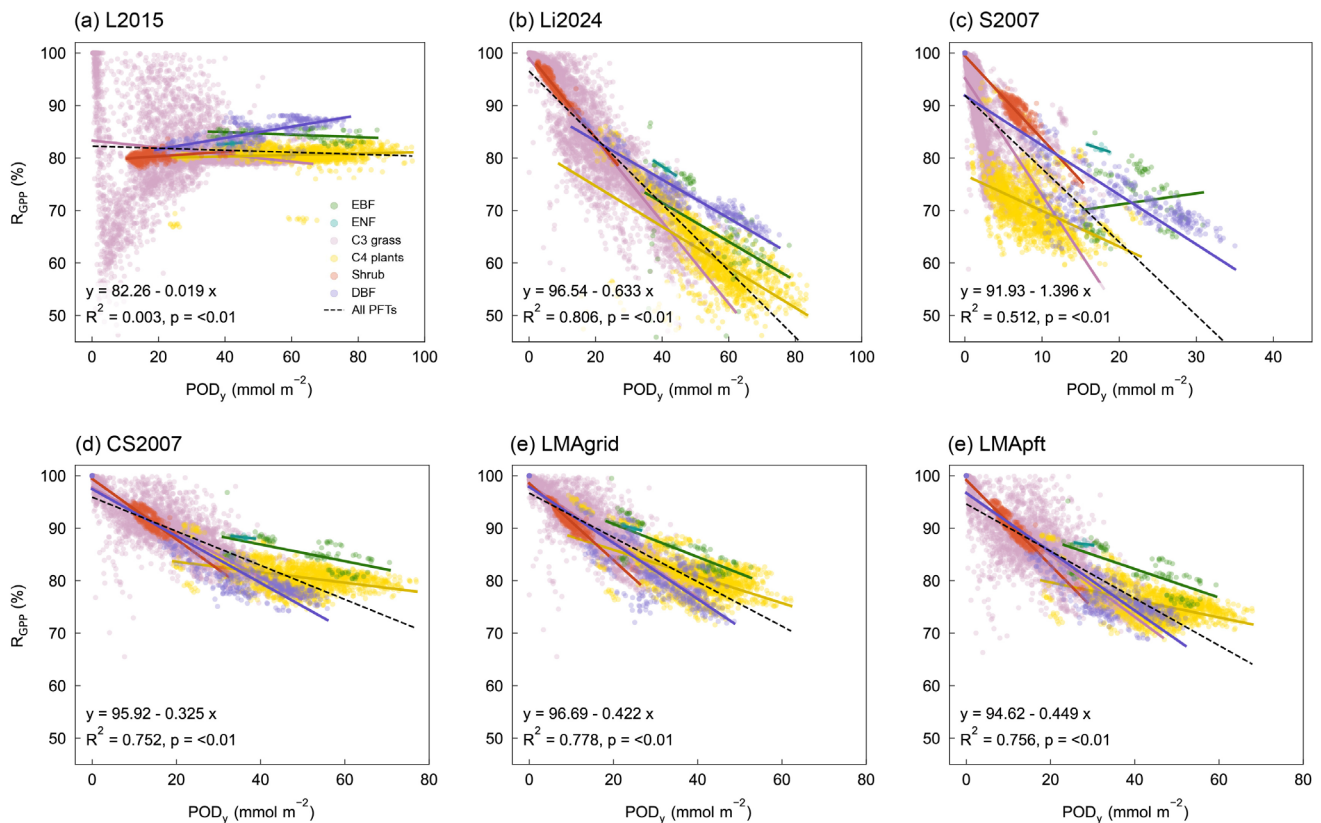
625 Figure 5. Dose–response relationships between relative gross primary productivity (RGPP) and POD y for six O 3 damage 630 parameterizations: (a) L2015, (b) Li2024, (c) S2007, (d) CS2007, (e) LMAgrid, and (f) LMApft. Each point represents simulated annual values for one grid cell over China. Colors denote the dominant PFT of each grid cell. Solid lines show PFT-specific linear fits for each scheme, and the dashed lines indicate the overall dose–response relationship for each parameterization across all PFTs. Regression equations and coefficients of determination for each scheme are reported in the corresponding panel.
