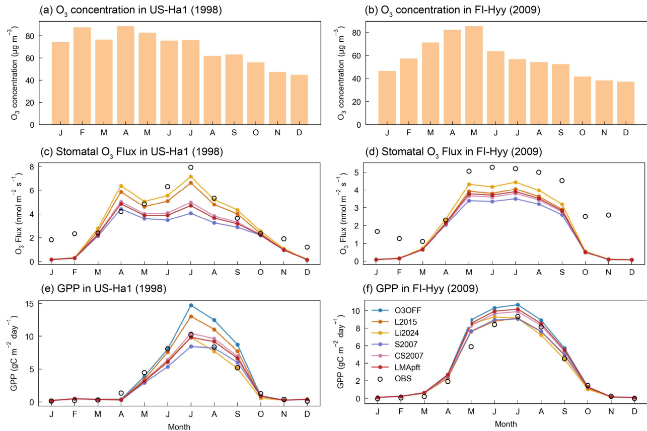
600 Figure 1. Site-level observations and simulations of monthly O 3 concentration (a, b), stomatal O 3 flux (c, d), and GPP (e, f) for US-Ha1 (1998) and FI-Hyy (2009), respectively. Colored lines denote different O 3 damage parameterizations, bars and symbols indicate field observations.
