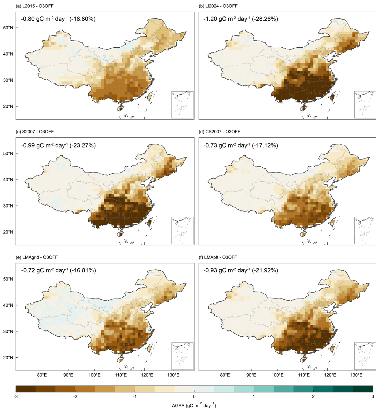
620 Figure 4. Comparison of O 3 -induced GPP loss in China simulated by six damage parameterizations. The panels show the simulated O 3 damage during the growing season (from April to September) for (a) L2015, (b) Li2024, (c) S2007, (d) CS2007, (e) LMAgrid, and (f) LMApft, respectively. The values in the upper-left corner indicate the area-weighted mean GPP loss over China and the corresponding relative change compared with O 3 OFF.
