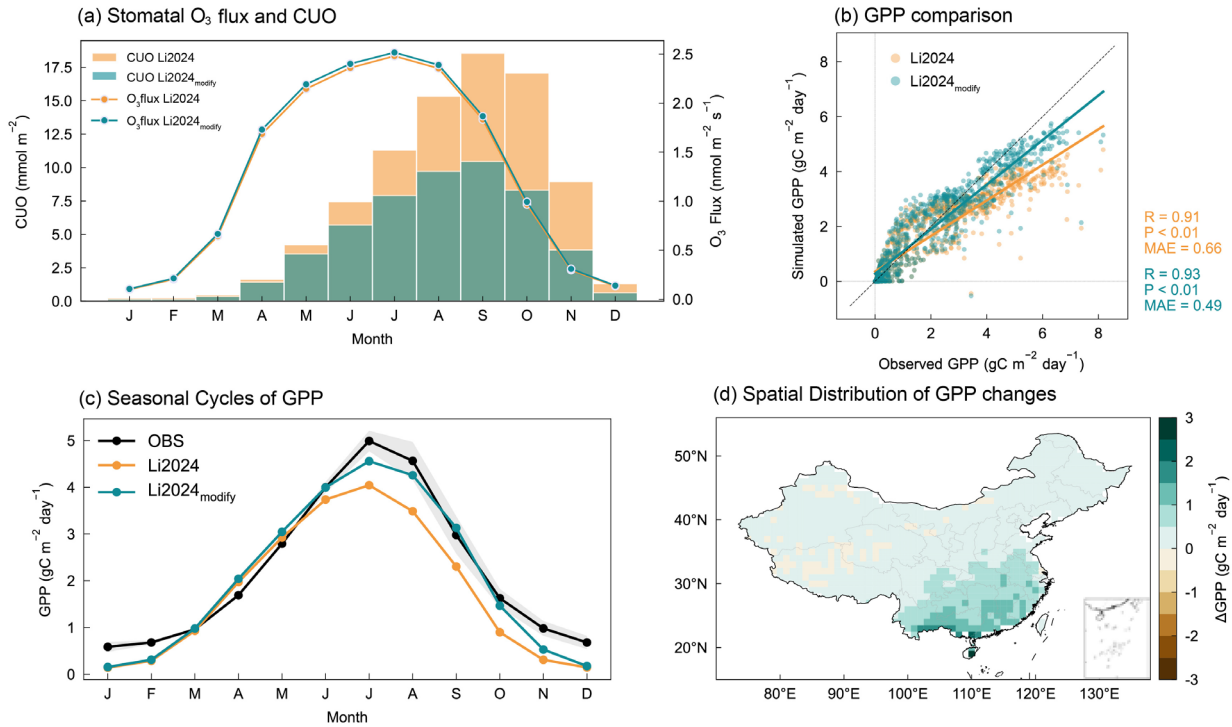
Figure 8. Comparison between the original and refined Li2024 parameterizations. (a) Instantaneous stomatal O 3 flux and cumulative uptake of O 3 (CUO) simulated by the original Li2024 and the refined Li2024 formulation (Li2024 modify ). (b) Grid-level comparison of simulated and observed annual mean GPP. The observed GPP is calculated as the mean of GOSIF and FLUXCOM products at each grid cell. (c) Seasonal cycles of GPP from observations, the original Li2024, and the refined Li2024 modify scheme. (d) Spatial patterns of annual GPP changes between the original and refined Li2024 formulations. The black line in (c) denotes the mean of GOSIF and FLUXCOM observations, and the grey shading indicates the range between these two products.
