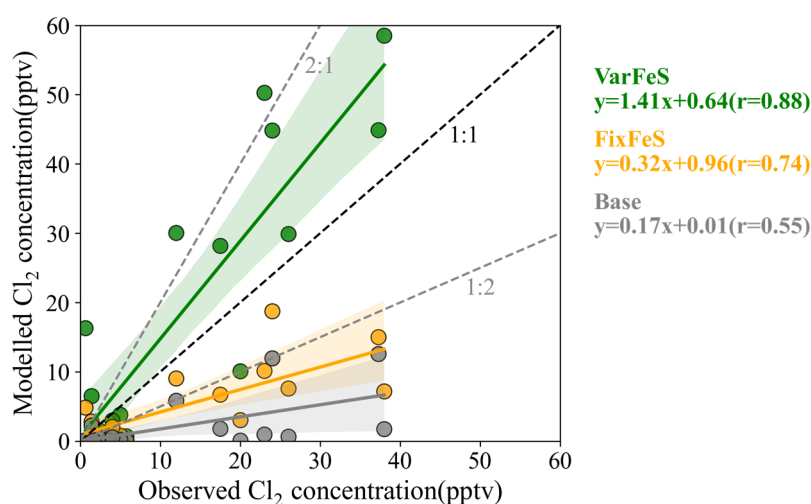
325 Figure 2. Comparison of modelled and normalized observed \text{Cl}_2 concentrations under different scenarios.
