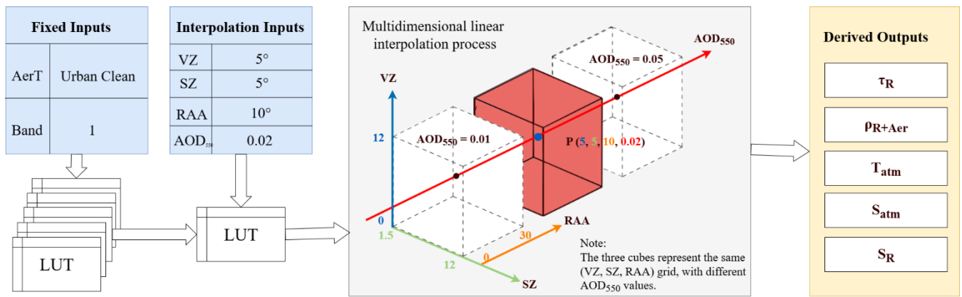
Figure 3: Input-Output Framework for Atmospheric Radiative Transfer Calculations Using Multidimensional LUT.
