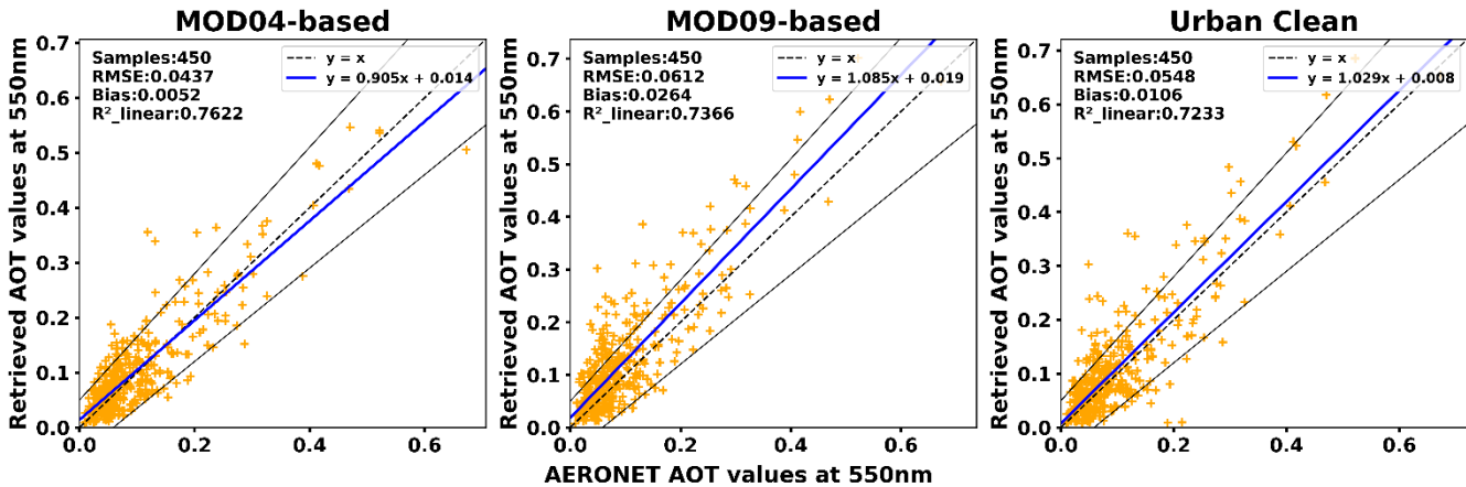
Figure 5: Scatter plot of 550 nm aerosol optical thickness (expected error: \Delta AOD = \pm(0.05 + 0.15 \times AOD_{AERONET}) ).
