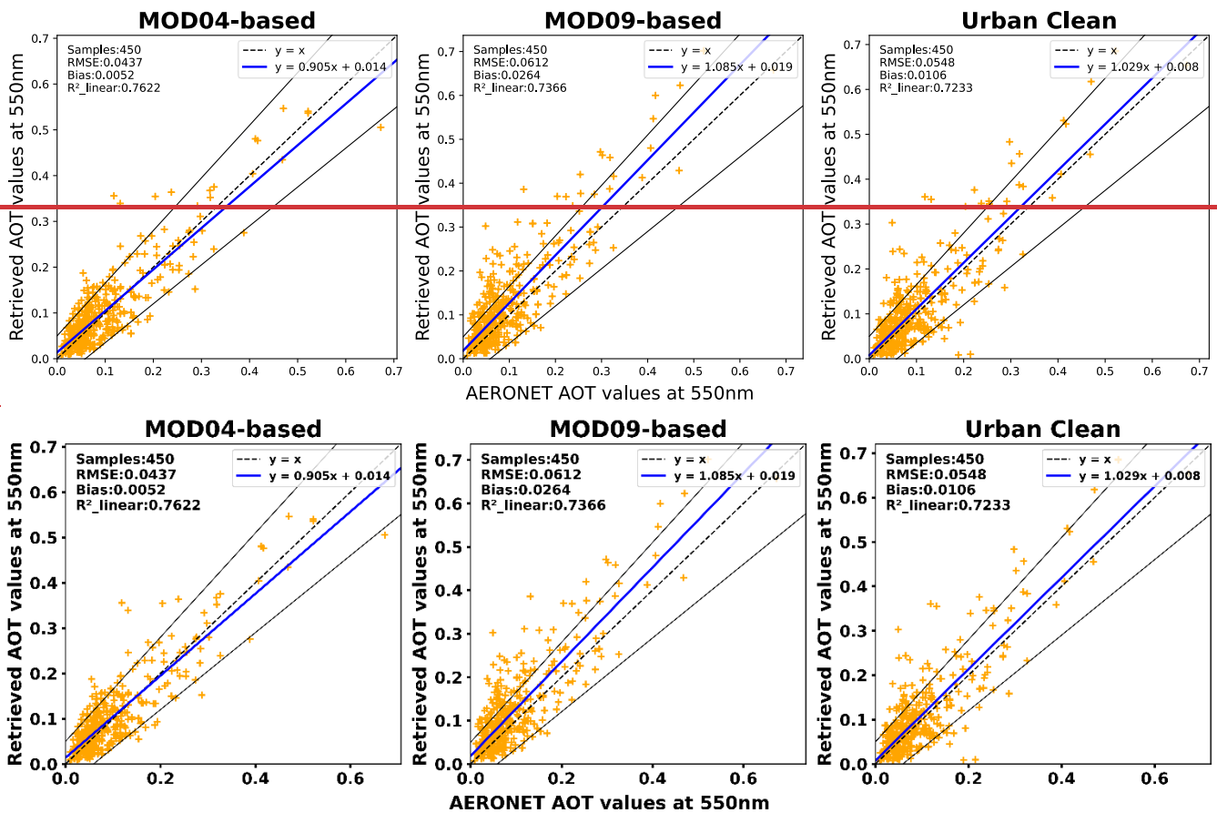
Figure 5: Dispersion plot of 550 nm aerosol optical thickness(specs= 0.15 \times \text{AOD}_{550} + 0.05 ).
