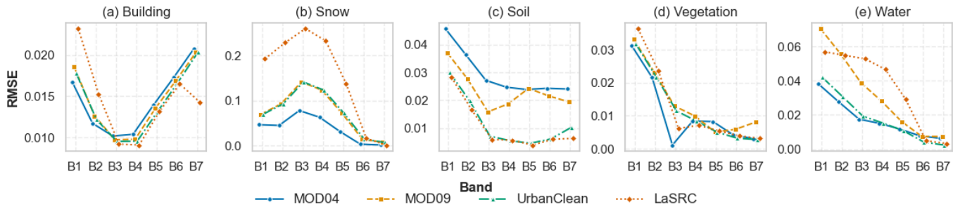
Figure 8: RMSE of the four surface reflectanceSR products across seven spectral bands.
