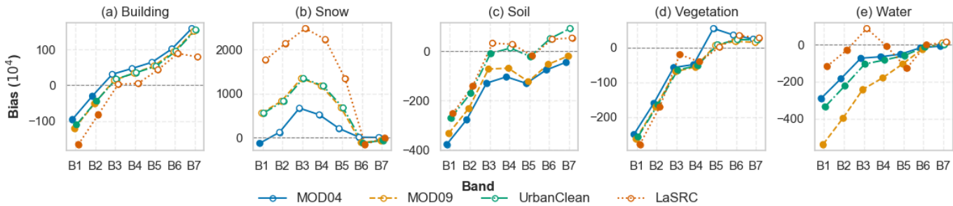
Figure 9: Bias of the four surface reflectanceSR products across seven spectral bands.
