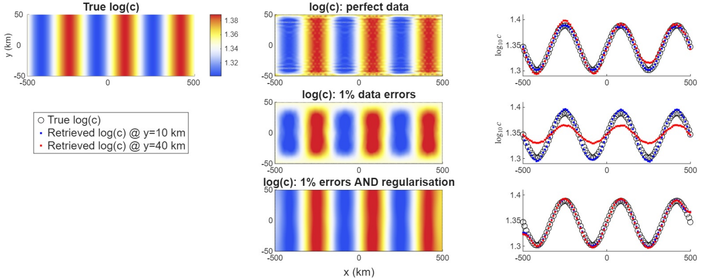
Figure 5. Examples of the basal slipperiness retrieval in \hat{U}a for the same experiment as in Fig. 4. for the laterally-confined channel, for a range of data errors and regularisation parameters of either zero or ( \gamma_a = 1 , \gamma_s = 10^3 \bar{h} ). We show contour plots of the retrieved field in the two-dimensional domain, and also cut-throughs at y = 0.2W and y = 0.8W .
