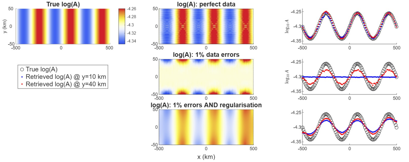
Figure 4. Examples of the viscosity retrieval in \hat{U}a for the laterally-confined channel, for a range of data errors and regularisation parameters of either zero or ( \gamma_a = 1 , \gamma_s = 10^3 \bar{h} ). We show contour plots of the retrieved field in the two-dimensional domain, and also cut-throughs at y = 0.2W and y = 0.8W . The parameter values for the domain are equivalent to the example in Fig. 2, but we now use dimensions \bar{h} = 1000\text{m} , \tau_d = 450\text{kPa} and \eta = 10^4\text{kPa.yr} .
