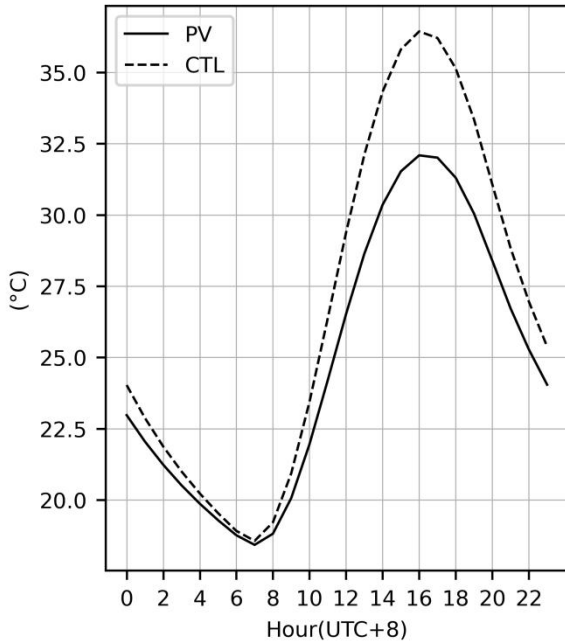
Figure 7: Mean diurnal cycle of the 0–7 cm soil temperature in WRF_PV and WRF_CTL, averaged over all PV grid cells.
