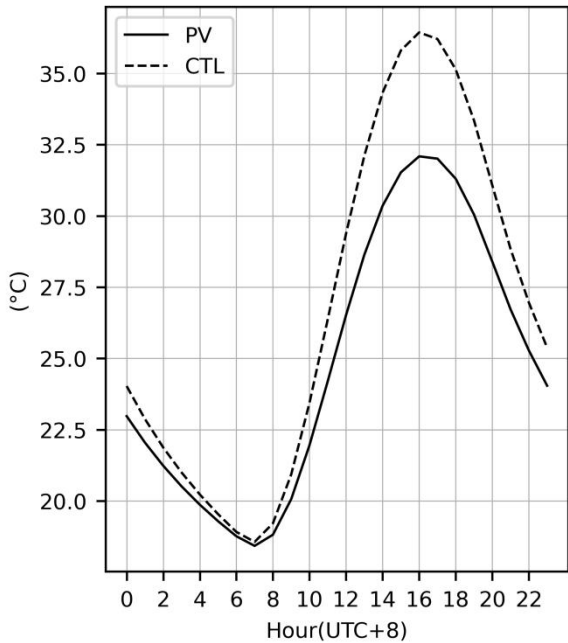
370 Figure 7: Mean diurnal cycle of the 0–7 cm soil temperature in WRF_PV and WRF_CTL, averaged over all PV grid cells.
