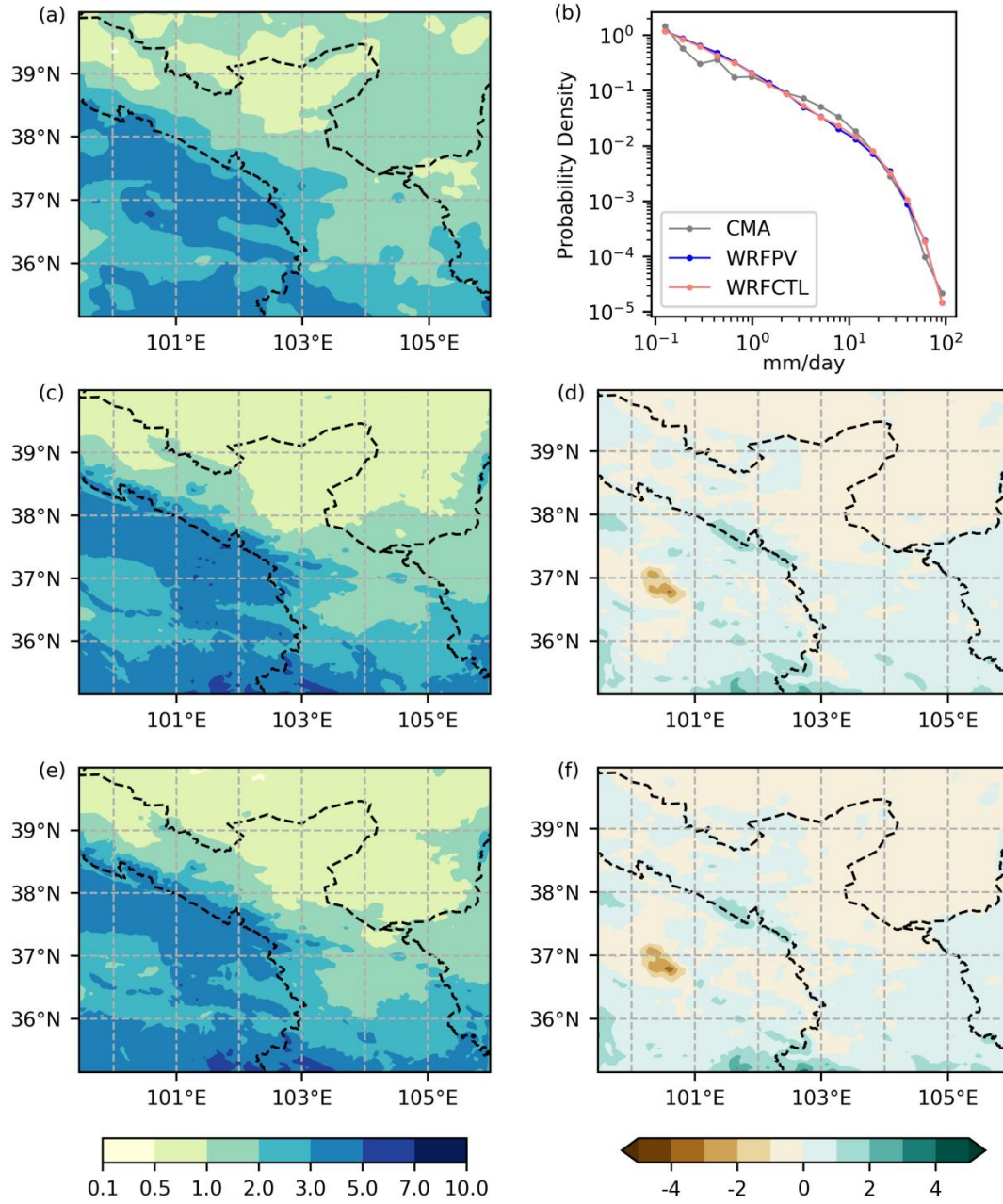
280 Figure 3: Spatial distribution of mean precipitation (mm day -1 ) during summer in D03: (a) CLDAS, (c) WRF_PV, and (e) WRF_CTL; differences of (d) WRF_PV-CLDAS and (f) WRF_CTL-CLDAS. (b) Probability distribution of daily precipitation intensity derived from CMA station observations (grey line) and from WRF_PV (blue line) and WRF_CTL (red line). Simulation results were interpolated to station points.
