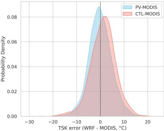
305 Figure 4: Probability density distributions of skin temperature (TSK, °C) errors for the WRF_PV (blue shade) and WRF_CTL (red shade) simulations with respect to MODIS observations. The vertical dashed line denotes zero error.
