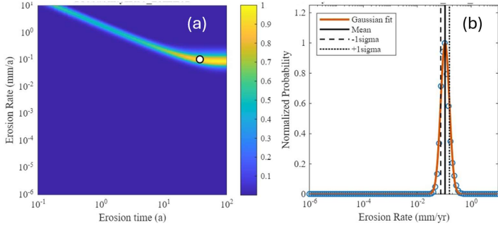
Figure 4: (a) The probability likelihood surface plot of \dot{\epsilon} - t_s 10^4 pairs in log-space for the sample IR50_BALL02. The light greenish-blue shaded sloped portion points towards a mildly fitting possible transient-state solution. The yellow-shaded patch represents the possible steady-state solutions. The white-filled circle defines the minimum t_{ss} . (b) The Gaussian distribution of \dot{\epsilon}_{ss} for t_{ss} = 38 a. The blue circles define the normalised values of probability likelihood of the erosion rate column of t_{ss} and fitted with a Gaussian distribution function. The solid, dotted and dashed black line represents represent the mean, +\delta and -\delta , respectively.
