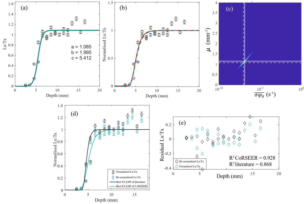
Figure 2: Re-evaluation of the IR50 calibration parameters for sample ROAD02 (IR50_ROAD02) (Smedley et al., 2021). (a) The natural IR50 Lx/Tx depth profiles (hollow circles) and associated sigmoidal fit (teal solid line). Although the normalisation was already performed by the Smedley et al. (2021), the fitted amplitude showed a = 1.085 , indicating \sim 8.5\% under-normalisation. Parameters b and c indicate the steepness and x_{0.5} , respectively. (b) The simulated LDPs for best-fit (dashed blue) and median (solid orange) calibration parameters associated with the SCF-normalised LDP (hollow circles). The precise overlap between both simulated LDPs shows a great agreement between the best-fit and median values, indicating plausible fitting strategies. (c) Probability likelihood distribution in \sigma\phi_0 and \mu space from Bayesian inversion. The dashed lines represent the best-fitting values, and the solid line represents the median of the filtered values using the criteria described in Section 3.2.2. (d) Direct comparison of the literature-normalised profile (black circles) and CoRSEER-ISCFSF-normalised profile (cyan square) using CoRSEER-I alongside their corresponding best-fit simulated luminescence depth profile (black and cyan lines). Both datasets show comparative x_{0.5} , but there is a slight change in the slope after renormalisation. (e) Residuals (data – model) as a function of depth for both fits, highlighting the improved agreement for CoRSEER-I. The coefficient of determination increases from R^2 = 0.868 (literature handling) to R^2 = 0.928 (CoRSEER-I), indicating a tighter, more precise fit to the same underlying measurements.
