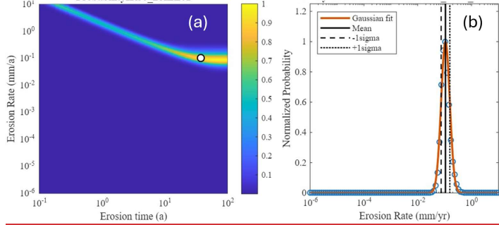
Figure 4: (a) The probability likelihood surface plot of \bar{\epsilon} - t_s pairs in log-space for the sample IR50_BALL02. The light greenish-blue shaded sloped portion points towards a mildly fitting possible transient-state solution. The yellow-shaded patch represents the possible steady-state solutions. The white-filled circle defines the minimum t_{ss} . (b) The Gaussian distribution of \bar{\epsilon}_{ss} for t_{ss} = 38 a. The blue circles define the normalised values of probability likelihood of the erosion rate column of t_{ss} and fitted with a Gaussian distribution function. The solid, dotted and dashed black line represents mean, +\delta and -\delta , respectively.
