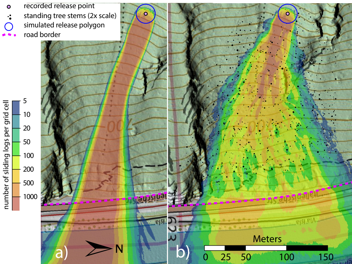
Figure A1. Additional simulations based on the 2022 event in Plattawald, Rothenbrunnen (CH). All simulations were performed with 20000 randomly distributed upright logs within the release polygon and a friction coefficient of \mu = 0.25 . The colours indicate the number of logs intersecting each 0.5 m \times 0.5 m grid cell, highlighting preferential sliding paths of the deadwood. a) Simulation without forest. b) Simulation with a randomly generated forest. Map and hillshade from swisstopo (2020–2024).
