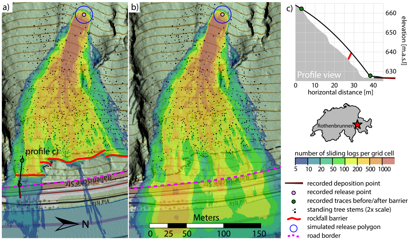
Figure 4. Reconstruction of the 2022 event in Plattawald, Rothenbrunnen (CH). All simulations were done with 20000 randomly distributed upright logs within the release polygon and a friction coefficient of \mu = 0.25 . The colours indicate how many of the 20000 released logs intersect their motion with each 0.5 \times 0.5 m grid cell, revealing preferential sliding paths of the deadwood. a) Simulation with ALS-based tree locations and rockfall barriers. b) Simulation with ALS-based tree locations without barriers. c) Profile view in the vicinity of the presumably overjumped rockfall barrier with fitted flight parabola. Map and hillshade from swisstopo (2020–2024).
