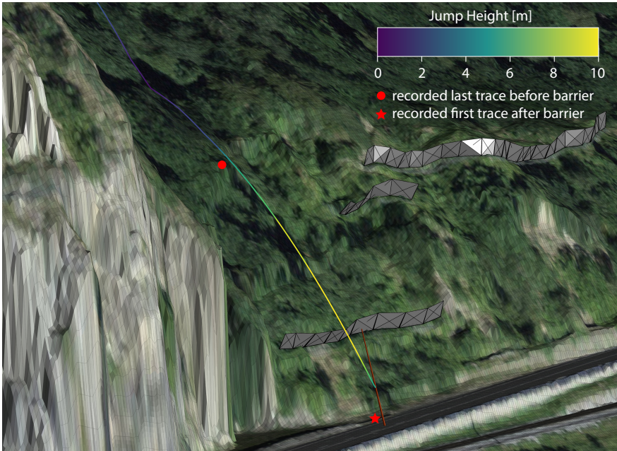
Figure B1. Three-dimensional simulation of a representative sliding deadwood trajectory at the Rothenbrunnen site. The figure shows the simulated log position at the time step when the log first touches the terrain after the jump over the barrier. The jump is initiated by a local plateau upslope of the barrier, leading to a maximum jump height of 9.9 m (measured as the vertical distance between the log centre of mass and the terrain) and a velocity of 27.8 \text{ m s}^{-1} at take-off. Background orthophoto from swisstopo (2020–2024).
