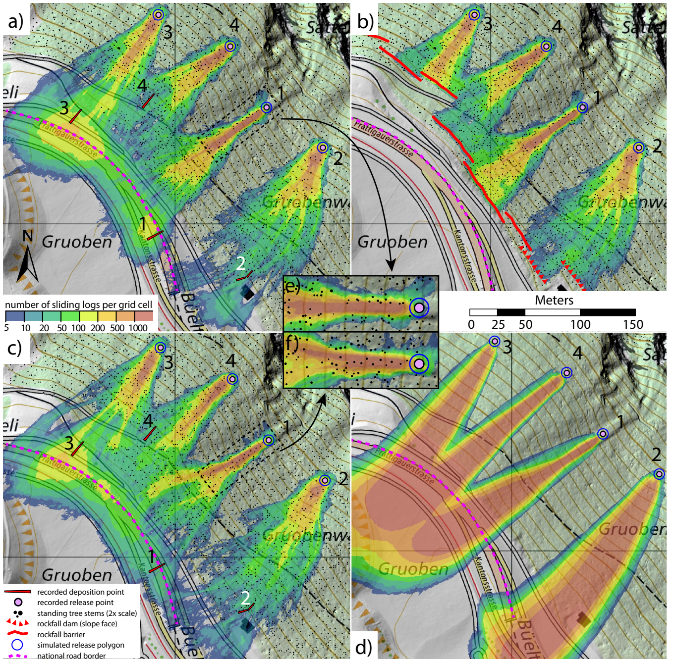
Figure 3. Reconstruction of the four events in Gruobenwald, Klosters (CH) with a friction coefficient of \mu = 0.25 . The colours indicate how many of the 20000 released logs intersect their motion with each 0.5 \times 0.5 m grid cell, revealing preferential sliding paths of the deadwood. a) Simulation without protection measures and ALS-based tree locations. b) Simulation with protection measures finished in 2024 and ALS-based tree locations. c) Simulation without protection measures and randomly generated forest. d) Simulation without protection measures and no forest. Two magnified sections below release 1 reveal the differences of the forest structure between ALS-based forest (e) and randomly generated forest (f). Map and hillshade from swiss topo (2020–2024).
