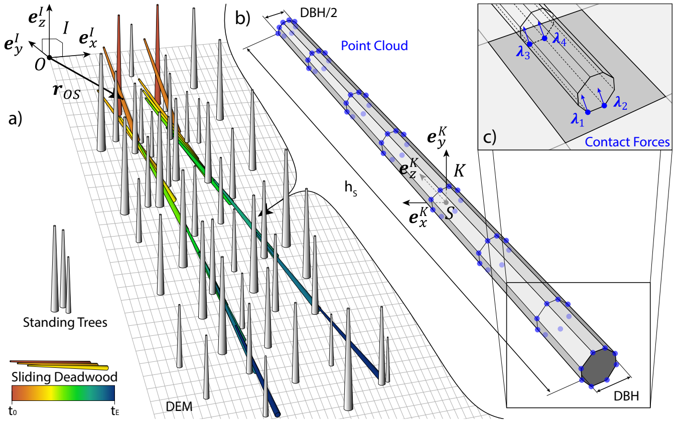
Figure 2. Simulation model of the sliding deadwood. a) DEM and standing trees are described in the inertial frame I . Two sliding deadwood logs are exemplary shown as a time series starting at the mobilisation time t_0 up to the deposition time t_E . b) Rigid, sliding deadwood with its geometry described as a point cloud in body-fixed frame K fixed at the centre of mass S . c) Contact between deadwood geometry and terrain with contact forces \lambda_i acting at vertex points of the point cloud.
