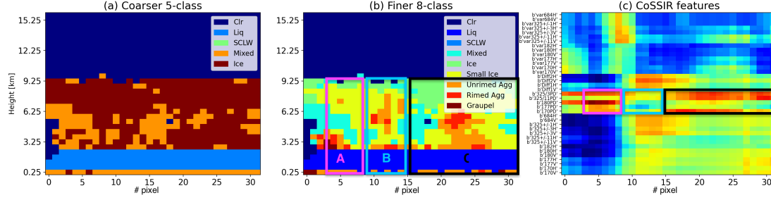
Figure 10. Combined (a) 5-class and (b) 8-class hydrometeor classifications for a cross-section of the storm, and (c) the collocated and coincident CoSSIR measurements (normalized for each variable). From bottom to top in (c): radiance ( TB ) following the order listed in Table 1 with V-pol first followed by H-pol for each frequency, polarization difference ( PD ) for 170, 177, 180, 325 \pm 11 , 325 \pm 3.4 GHz, TB difference between different channels ( 325 \pm 11V - 170V , 325 \pm 11H - 170H , 325 \pm 3V - 180V , 325 \pm 3H - 180H ) and variance of 14 channel TBs . All values have been normalized using min-max method with values ranging from 0 (deep blue) to 1 (bright red). The three colored rectangles encircle three different vertical cloud structures and their corresponding PD signals in CoSSIR. The PD signals are measured at 170, 177, 180, 325 \pm 11 and 325 \pm 3 GHz from lower to upper rows. Note that the horizontal resolution of (a) and (b) are coarsened both horizontally to \sim 500 m to match CoSSIR footprint size, and vertically to \sim 250 m. See text for the discussion about Regime A, B, and C circled in (b) and (c).
