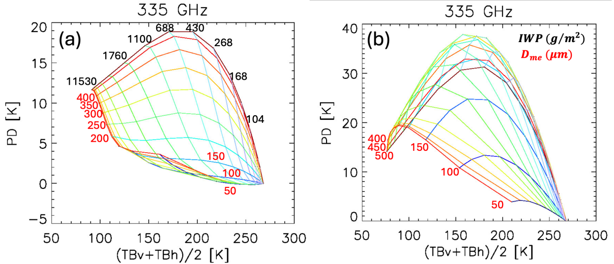
Figure 14. Look-up-table (LUT) for 325.15 + 10 GHz for (a) 6-bullet rosette and (b) column ice.
