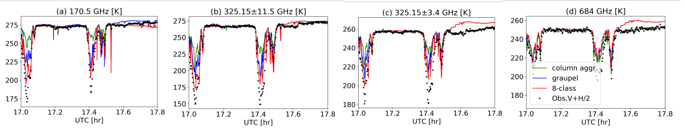
Figure 7. Timeseries of observed TB (black astericks) versus simulated TB . Red, blue and green lines are using detailed frozen hydrometeors, uniform graupel and uniform LCA assumptions, respectively. (a) 170.5 GHz; (b) 325.15 \pm 11.5 GHz; (c) 325.15 \pm 3.4 GHz; (d) 684 GHz. The observed TB is an average between V-pol and H-pol measurements.
