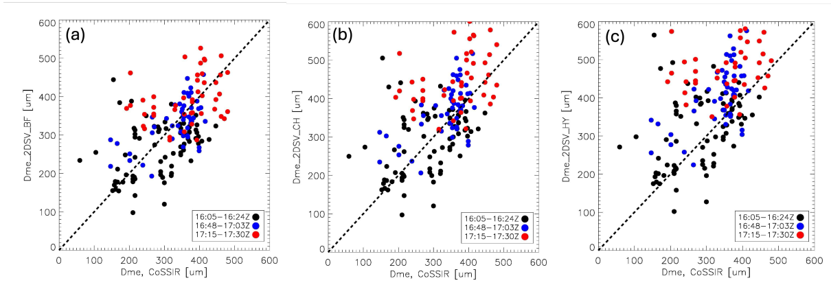
Figure 15. Scatter plots of retrieved D_{me} from CoSSIR 325.15 \pm 11 GHz (horizontal axis) in comparison with collocated 2D-S retrievals using the m - D relationship from (a)Brown and Francis (1995), (b)Chase et al. (2021) and (c)Heymsfield et al. (2010). Black, blue and red dots are taken from 16.08 – 16.4, 16.8 – 17.05 and 17.25 – 17.5 UTC periods, respectively.
