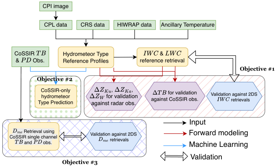
Figure 4. Architecture flow for this work. Green rectangles are observations (or ancillary atmospheric field) as retrieval or machine learning inputs. Yellow rectangles are retrieval products from this work, purple hexagons are consistency check as part of the closure study, and blue hexagons are independent validation from in-situ 2D-S cloud probe observations as the other part of the closure study. Red arrows represent forward modeling operator to convert physical parameters to remote sensing variables. Blue arrows represent the machine learning task. This paper includes three objectives, which are enclosed by the pink hatched area, green dotted area, and blue cross-hatched area, respectively.
