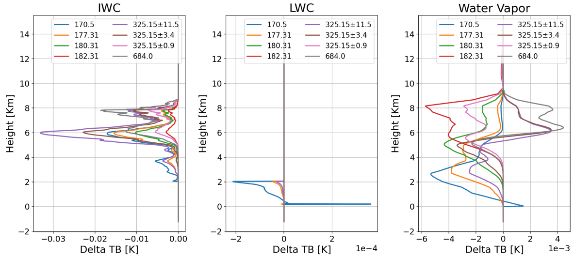
Figure A2. Jacobians for each channel for (a) IWC , (b) LWC and (c) water vapor that are provided in Fig. A1. The Jacobians are computed by perturbing each layer by 1% each time. Please note the value range in the horizontal axis.
