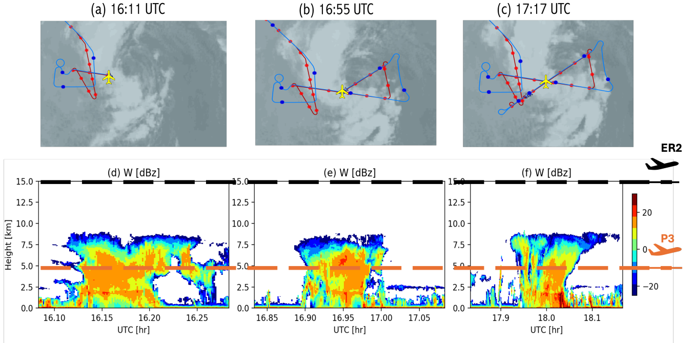
Figure 1. Illustration of the weather system and flight patterns of the Jan. 15, 2023 IMPACTS campaign case. Top rows are ER-2 (blue) and P-3 (red) flight routes overlaid on GOES-16 satellite false-color Advanced Baseline Imager (ABI) albedo measurements at three different UTC times. Dots mark the time at :05, :10, :15, and so on. Cyclone center was roughly at 37^{\circ}N , 70^{\circ}W . Bottom row presents the CRS radar reflectivity curtains during the corresponding time segments. Two aircraft icons roughly represent ER-2 and P-3 flight altitudes. Top panels are cropped from https://catalog.eol.ucar.edu/maps/impacts_2023 , last accessed: June 26, 2026, and bottom panels are calibrated L1B CRS W-band radar reflectivities at corresponding periods. GOES-16 ABI data courtesy of NOAA. NCAR/EOL map products courtesy of NCAR/UCAR. CRS radar data courtesy of NASA.
