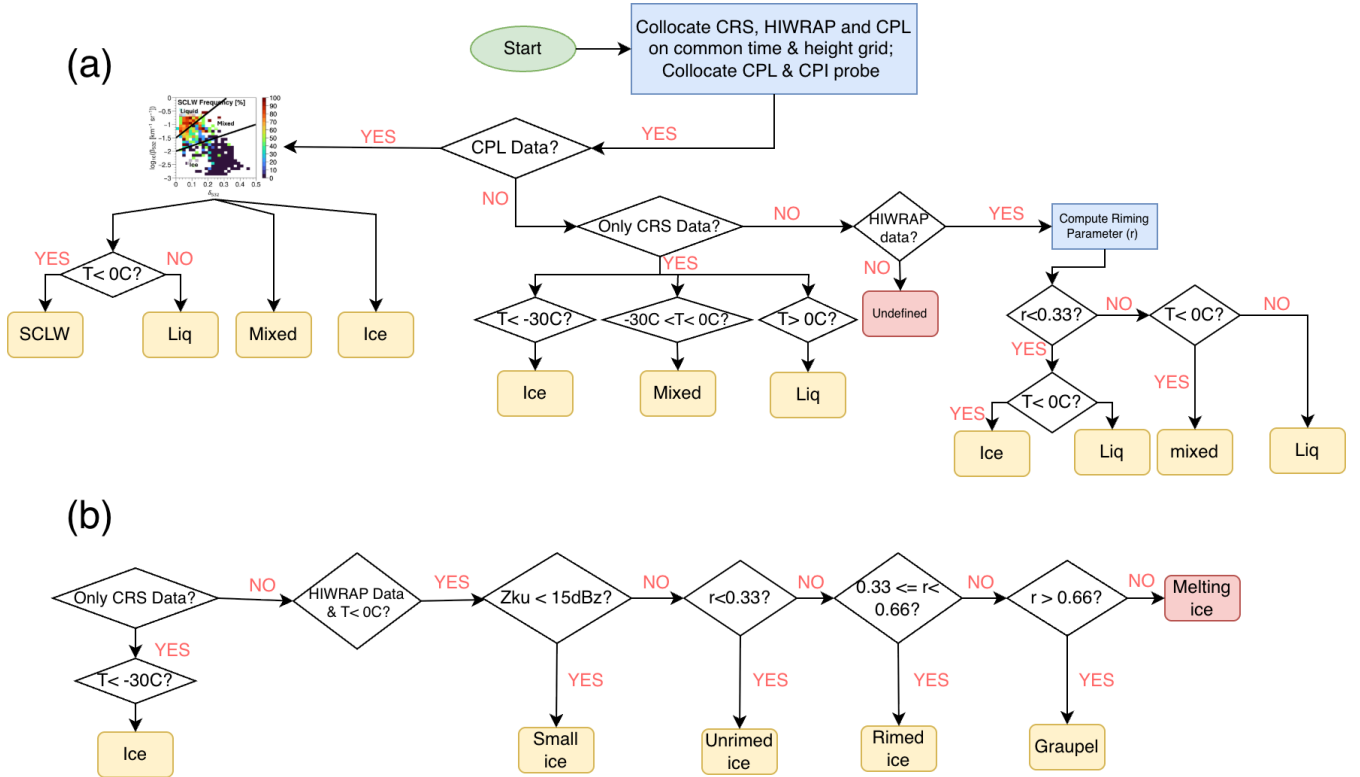
Figure 2. (a) Decision tree for the coarser 5-class hydrometeor classification using CRS, HIWRAP and CPL; (b) further decision tree for finer classification among the ice category. Blue rectangles enclose computing procedures; yellow rectangles enclose the final output categories while pink rectangles are either undefined or not considered in further analysis.
