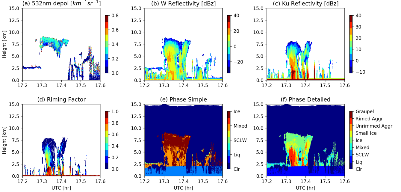
Figure 3. An example to show how the final hydrometeor type is decided based on (a) lidar 532 nm depolarization ratio ( \delta ) and backscatter ( \beta ; not shown); (b) W-band reflectivity; (c) Ku-band reflectivity; and (d) calculated riming parameter ( r ). The final coarse and detailed type classification products are shown in (e) and (f), respectively.
