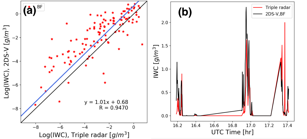
Figure 9. Comparison between joint CRS+HIWRAP IWC retrievals and 2D-S cloud probe retrievals at the collocated radar range bin where P-3 was cruising. (a) Scatter plots from the collocated samples and (b) displaying the same data samples using a timeseries. The Brown and Francis (1995) m - D relationship is used for 2D-S. Linear regression results for (a) are added as the blue line and equation/R-value written in the bottom right corner of panel (a).
