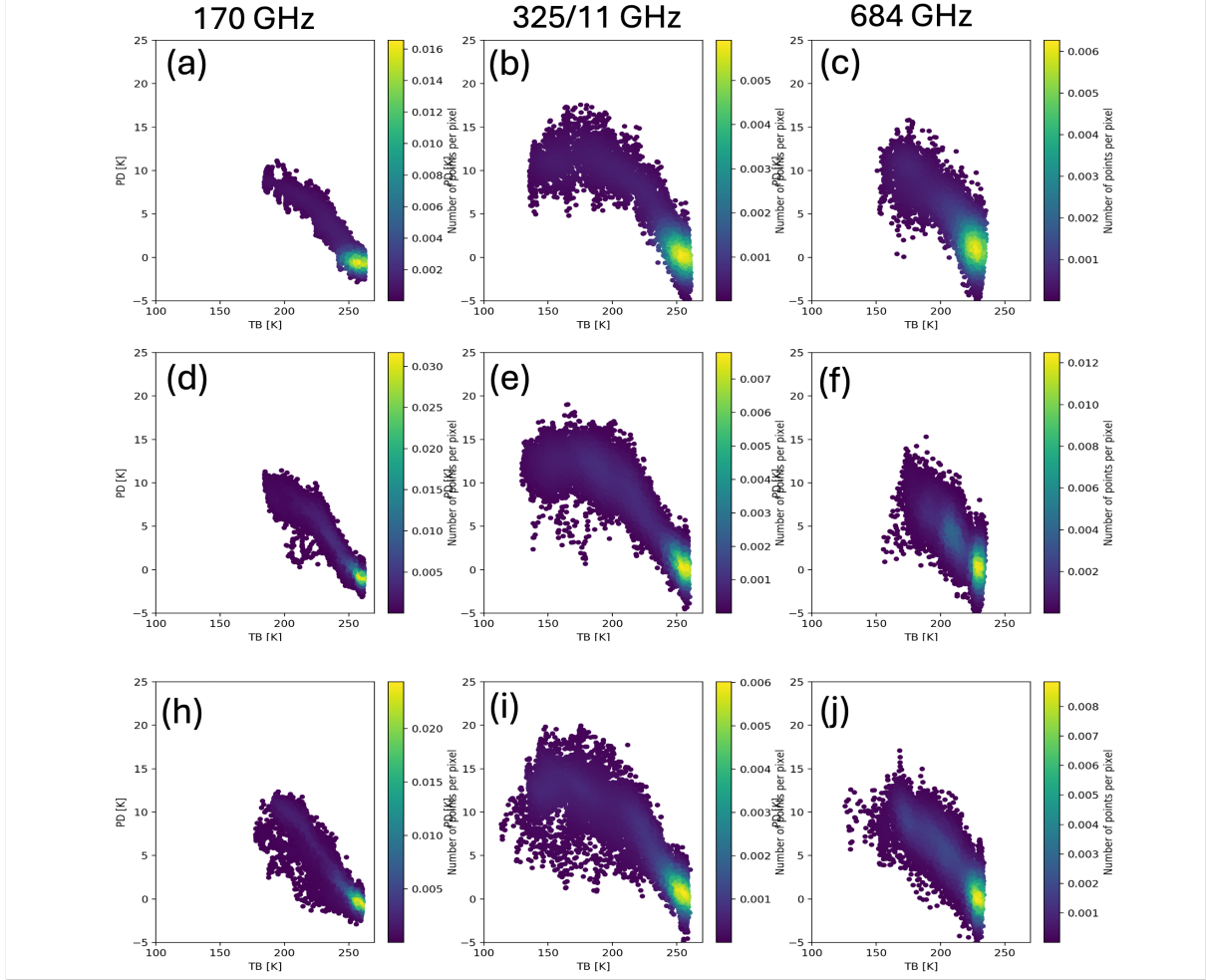
Figure B1. Same with Fig. 13, except the second row is made up from samples collected during 16.8 – 17.05 UTC, and last row from 17.25 – 17.5 UTC.
