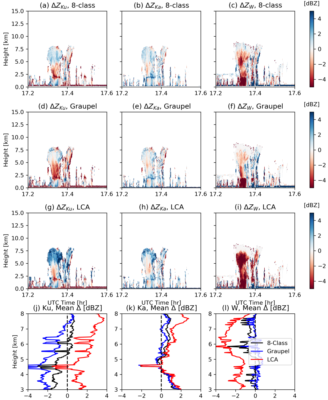
Figure 6. Reflectivity difference \Delta Z between simulated and observed ones for HIWRAP-Ku (left), HIWRAP-Ka (middle) and CRS (right) using three different ice habit assumptions. The top row employs the three detailed ice class (LCA/ECA/Graupel), the middle row assumes graupel-only for all frozen hydrometeors and the 3rd row assumes LCA everywhere for all frozen hydrometeors. The bottom row shows the comparison of mean difference as a function of height for Ku, Ka and W band, respectively.
