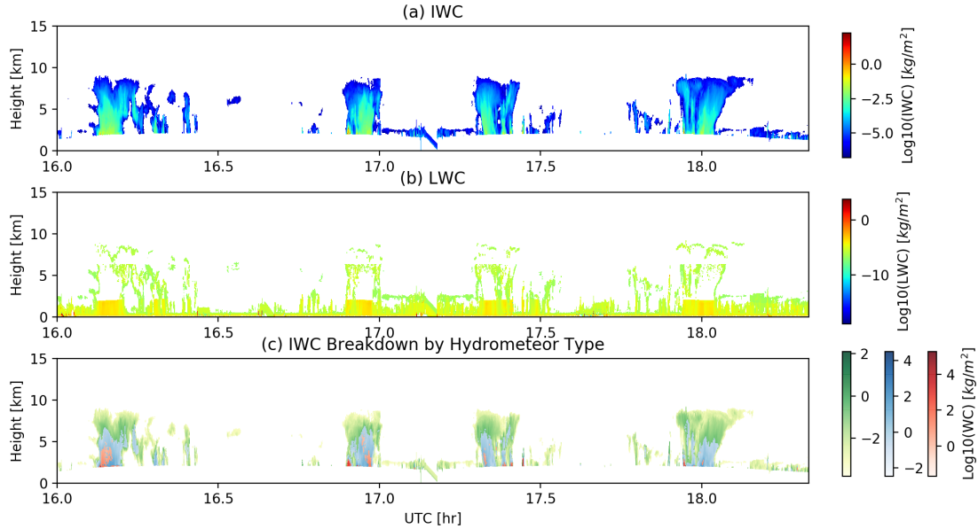
Figure 5. Vertical water content ( WC ) profile retrieved from CRS plus HIRWAP. (a) IWC ; (b) LWC ; (c) IWC from cloud ice (green), snow aggregates (blue), graupel (red) and liquid. Colorbars are in \text{Log}_{10} -scale. Note that positive LWC pixels overlap with many of the positive IWC pixels (e.g., cloud top, cloud boundary, SCLW layer, etc.), so they are shown separately in (a) and (b) to ease visual comparison.
