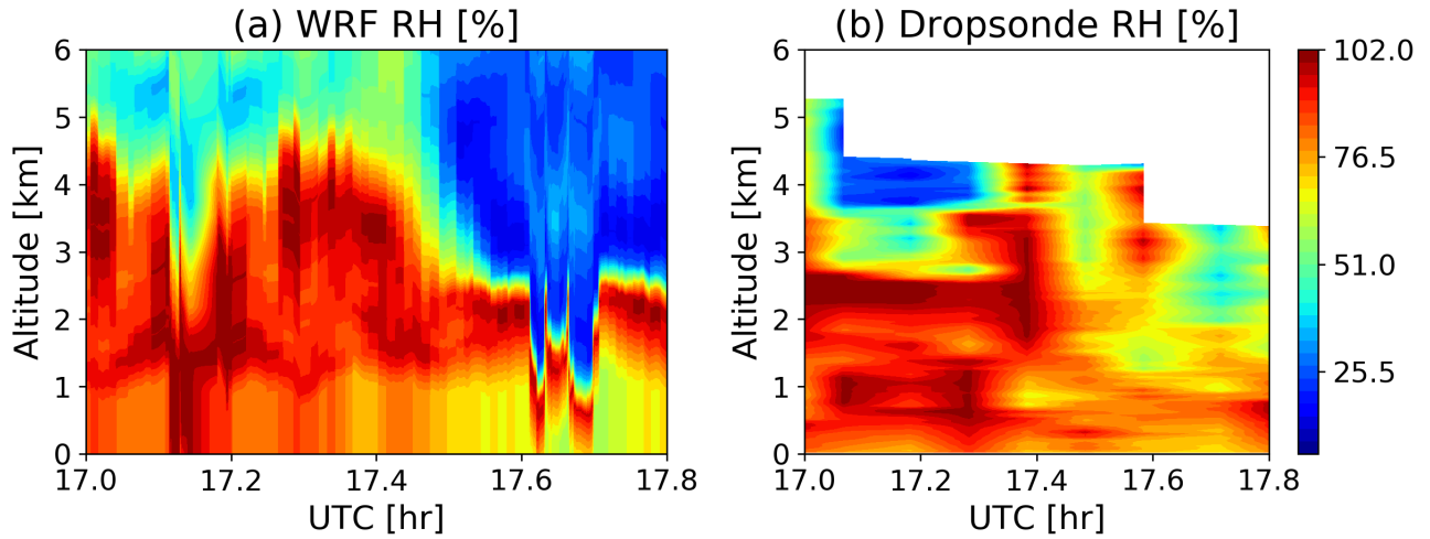
Figure 8. Timeseries of (a) WRF model simulated relative humidity (RH, unit in %) and (b) Dropsonde observed ones during the same period of Fig. 7 (17 - 17.8 UTC).
