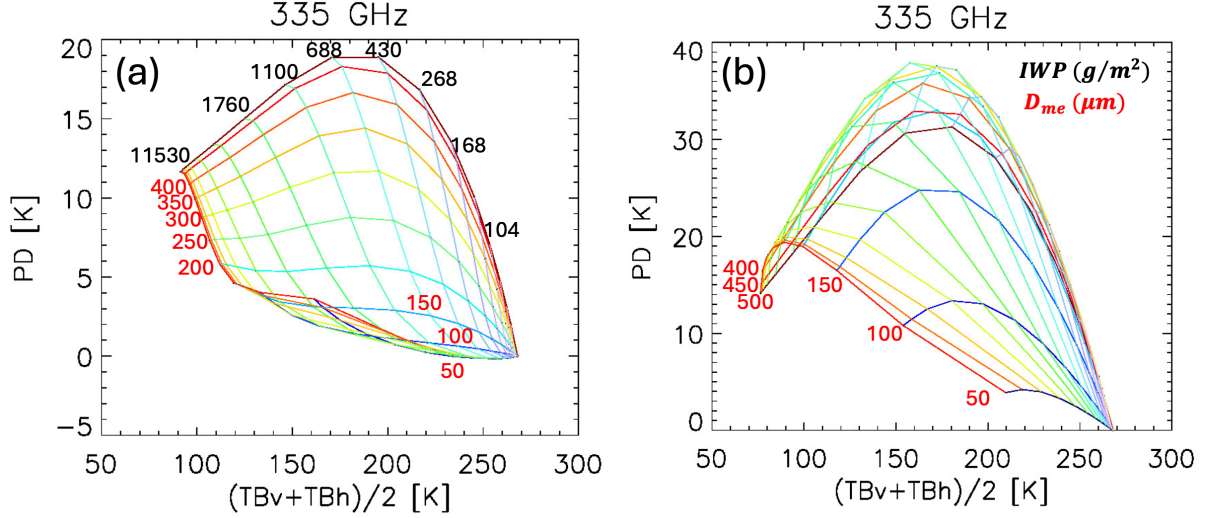
Figure 14. Look-up-table (LUT) for 325.15 \pm 10 GHz for (a) 6-bullet rosette and (b) column ice.
