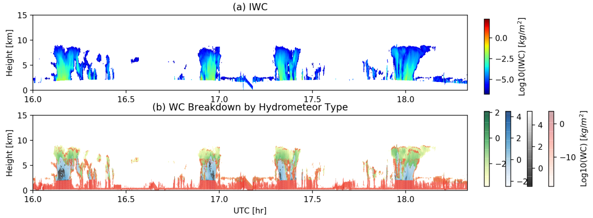
Figure 5. Vertical water content (WC) profile retrieved from CRS plus HIRWAP. (a) IWC; (b) WC from cloud ice (green), snow aggregates (blue), graupel (grey) and liquid (red). Colorbars are in Log10-scale. Note that positive LWC pixels overlap with many of the positive IWC pixels (e.g., cloud top, cloud boundary, SCLW layer, etc.), which cannot be separated clearly in Panel b.
