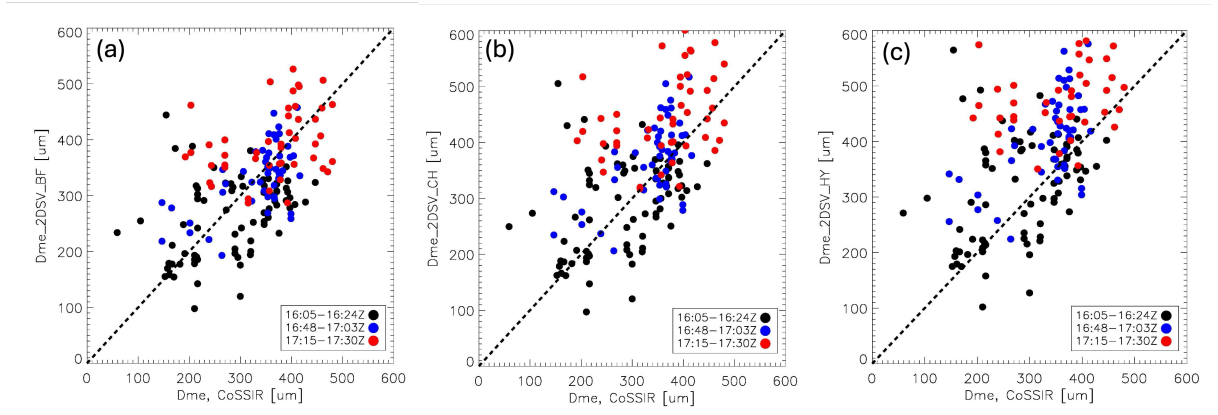
Figure 15. Scatter plots of retrieved D_{me} from CoSSIR 325.15 \pm 11 GHz (horizontal axis) in comparison with collocated 2D-S retrievals using the m - D relationship from (a) Brown and Francis (1995), (b) Chase et al. (2021) and (c) Heymsfield et al. (2010). Black, blue and red dots are taken from 16.08 – 16.4, 16.8 – 17.05 and 17.25 – 17.5 UTC periods, respectively.
