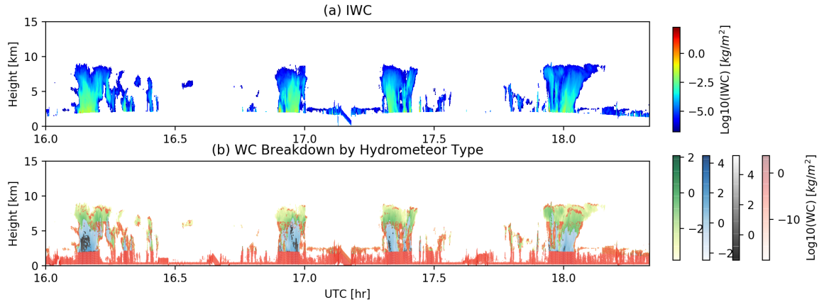
Figure 5. Vertical water content (WC) profile retrieved from CRS plus HIRWAP. (a) IWC; (b) WC from cloud ice (green), snow aggregates (blue), graupel (grey) and liquid (red). Colorbars are in \log_{10} -scale. Note that positive LWC pixels overlap with many of the positive IWC pixels (e.g., cloud top, cloud boundary, SCLW layer, etc.), which cannot be separated clearly in Panel b.
