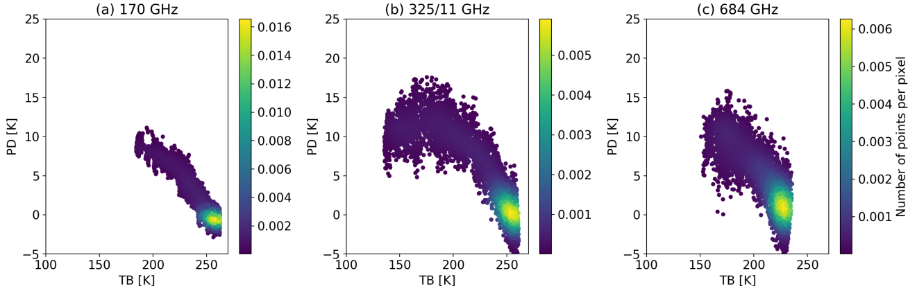
Figure 13. Density plots of the observed PD-TB relationship during 16.08–16.4 16:05-16:24 UTC for (a) 170 GHz, (b) 325.15 \pm 11 GHz and (c) 684 GHz.
