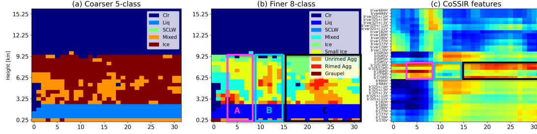
Figure 10. Combined (a) 5-class and (b) 8-class hydrometeor classifications for a cross-section of the storm, and (c) the collocated and coincident CoSSIR measurements (normalized for each variable). From bottom to top in (c): radiance (TB) following the order listed in Table 1 with V-pol first followed by H-pol for each frequency, polarization difference (PD) for 170, 177, 180, 325 \pm 11 , 325 \pm 3.4 GHz, TB difference between different channels ( 325 \pm 11V - 170V , 325 \pm 11H - 170H , 325 \pm 3V - 180V , 325 \pm 3H - 180H ) and variance of 14 channel TBs. All values have been normalized using min-max method with values ranging from 0 (deep blue) to 1 (bright red). The three colored rectangles encircle three different vertical cloud structures and their corresponding PD signals in CoSSIR. The PD signals are measured at 170, 177, 180, 325 \pm 11 and 325 \pm 3 GHz from lower to upper rows. Note that the horizontal resolution of (a) and (b) are coarsened both horizontally to \sim 500 m to match CoSSIR footprint size, and vertically to \sim 250 m. see text for the discussion about Regime A, B, and C circled in (b) and (c).
