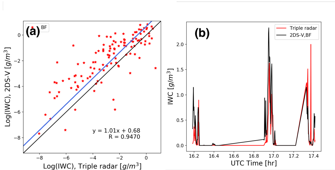
Figure 9. Comparison between joint CRS+HIWRAP IWC retrievals and 2D-S cloud probe retrievals at the collocated radar range bin where P-3 was cruising. (a) Scatter plots from the collocated samples and (b) displaying the same data samples using a timeseries. The Brown and Francis (1995) m - D relationship is used for 2D-S.
