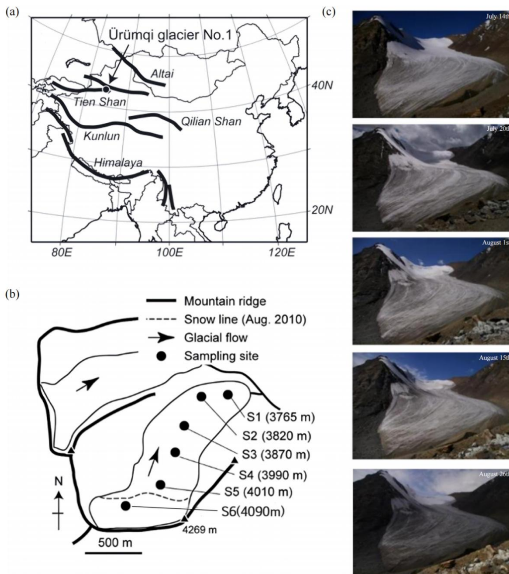
120 121 Figure 1: Location maps and photographs of Urumqi Glacier No.1. (a) Location of Urumqi Glacier No.1 in 122 the Tien Shan Mountains. (b) Map of sampling sites (S1–S6) in this study. (c) Photographs of Urumqi 123 Glacier No.1 across five sampling periods in 2013.
