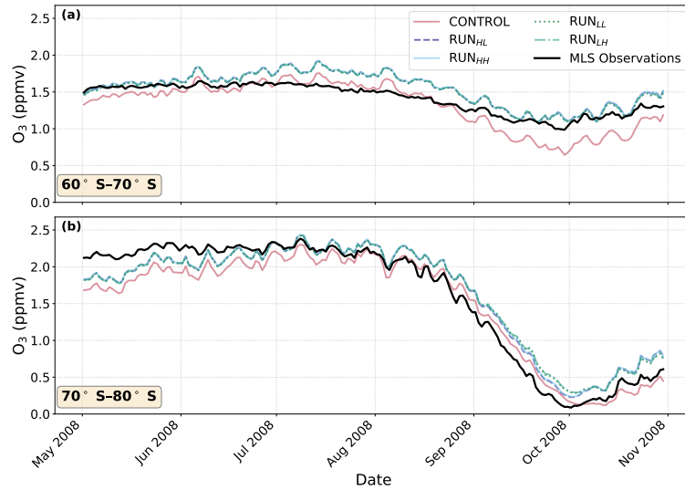
Figure 9. As Fig. 6, but for zonal mean \text{O}_3 (ppmv) at 68 hPa . Note that there is almost complete overlap of \text{RUN}_{\text{HH}} and \text{RUN}_{\text{HL}} , and \text{RUN}_{\text{LL}} and \text{RUN}_{\text{LH}} , resulting in only \text{RUN}_{\text{HH}} and \text{RUN}_{\text{LL}} being visible in the plot.
