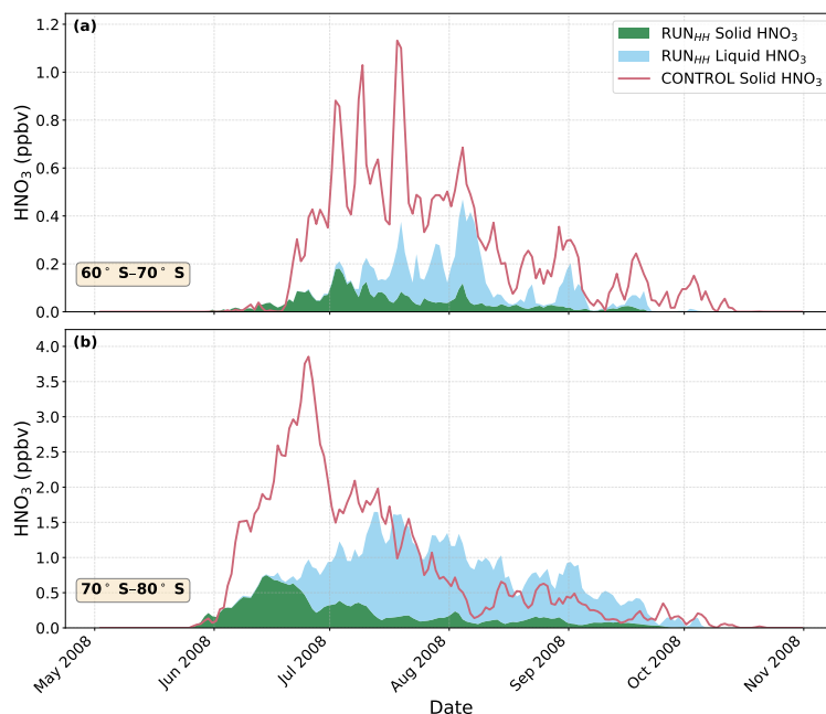
Figure 7. As Fig. 6, but for the zonal mean volume mixing ratio of solid-phase and liquid-phase \text{HNO}_3 (ppbv) at 68 hPa for CONTROL (pink line) and \text{RUN}_{\text{HH}} over the Antarctic for the extended 2008 winter season (green area May to October), as well as averaged across latitude bands 60^\circ\text{S} – 70^\circ\text{S} (a), and 70^\circ\text{S} – 80^\circ\text{S} (b). Solid-phase \text{HNO}_3 for CONTROL is shown with a pink line. The solid- and liquid-phase \text{HNO}_3 (blue area) for \text{RUN}_{\text{HH}} are shown as a stacked area, with solid-phase in green and liquid-phase in blue. Note that liquid-phase \text{HNO}_3 is not shown for CONTROL, as this is not simulated by the original PSC parameterisation. Also, the panels have different scales.
