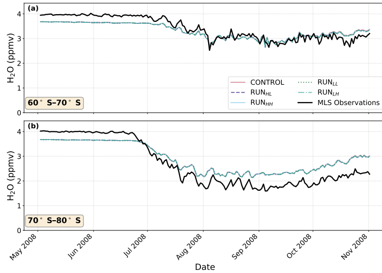
Figure 8. As Fig. 6, but for zonal mean gas-phase \text{H}_2\text{O} (ppmv). Note that there is complete overlap of all model runs (CONTROL and sensitivity simulations).
