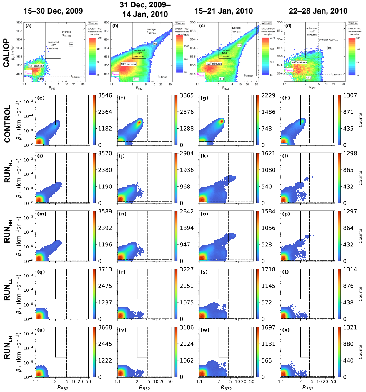
Figure 2. 2D histogram of optical properties from CALIOP (a–d), CONTROL (e–h), RUN HL (i–l), RUN HH (m–p), RUN LL (q–t), and RUN LH (u–x) over the Arctic for the 2009/2010 winter season, covering a latitude range of 65°N–75°N, and height range of 15–30 km. The results are separated into four distinct periods, comprising 15–30 Dec 2009 (first column), 31 Dec 2009–14 Jan 2010 (second column), 15–21 Jan 2010 (third column), and 22–28 Jan 2010 (fourth column). The results are plotted with the same classification algorithm, shading, boundaries, and regions as Fig. 1.
