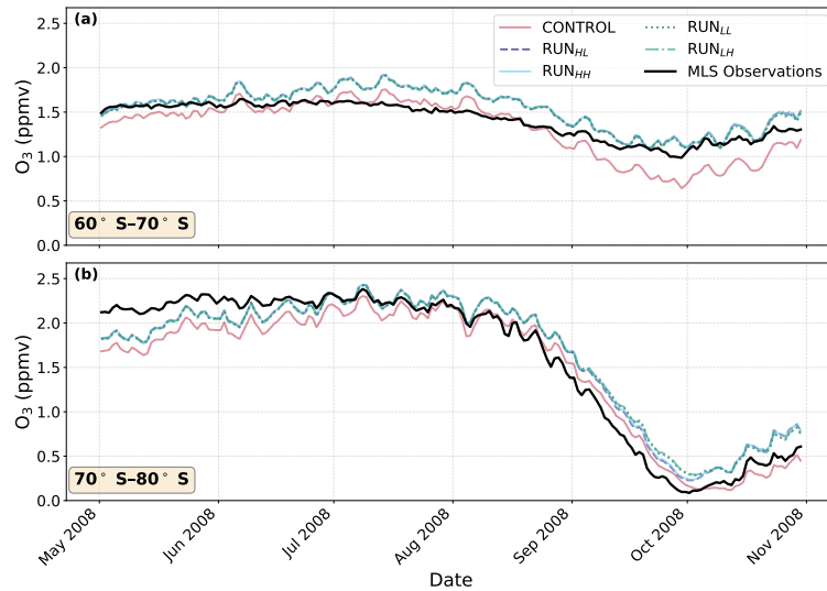
Figure 9. As Fig. 6, but for zonal mean \text{O}_3 (ppmv). Note that there is almost complete overlap of \text{RUN}_{\text{HH}} and \text{RUN}_{\text{HL}} , and \text{RUN}_{\text{LL}} and \text{RUN}_{\text{LH}} , resulting in only \text{RUN}_{\text{HH}} and \text{RUN}_{\text{LL}} being visible in the plot.
