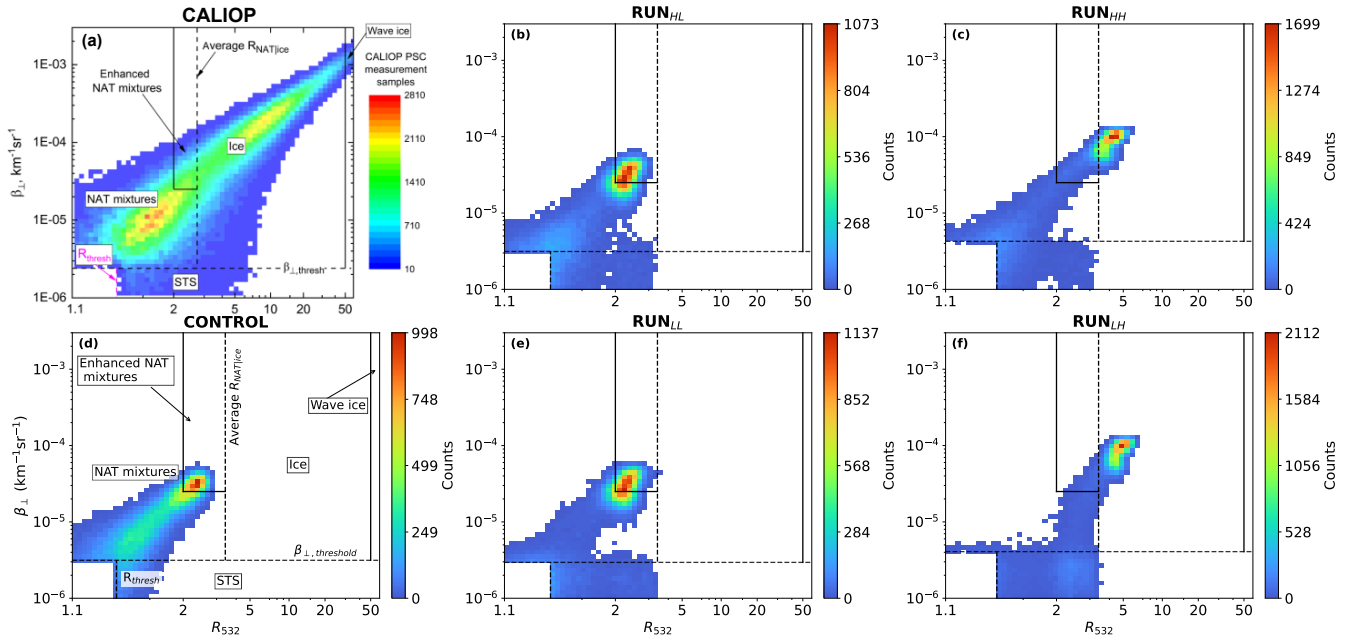
Figure 1. 2D histogram of optical properties from CALIOP (a), CONTROL , and RUN HL (b), RUN HH (c), CONTROL (d), RUN LL (e), and RUN LH (f) over the Antarctic for the period July 10–18 2008, covering a latitude range of 65°S–75°S, and potential temperature range of 475–525 K. The optical properties are plotted in the CALIOP v2 classification coordinate system of R_{532} vs \beta_{\perp} , with regions of enhanced NAT mixtures (enhNAT), liquid-NAT mixtures (NATmix), STS, ice, and wave ice indicated. The shading indicates the number of CALIOP observations (a), or the number of model grid points (b–f). Dashed lines indicate the mean \beta_{\perp} and R_{532} thresholds (including measurement uncertainty), as well as the mean R_{\text{NATice}} boundary, calculated for CALIOP and each simulation separately. Solid lines indicate the boundary boundaries separating wave ice, and enhanced-NAT (ice and enhNAT) and NATmix. The regions labelled for CONTROL (d) are the same for all the sensitivity simulations (b, c, e, f).
