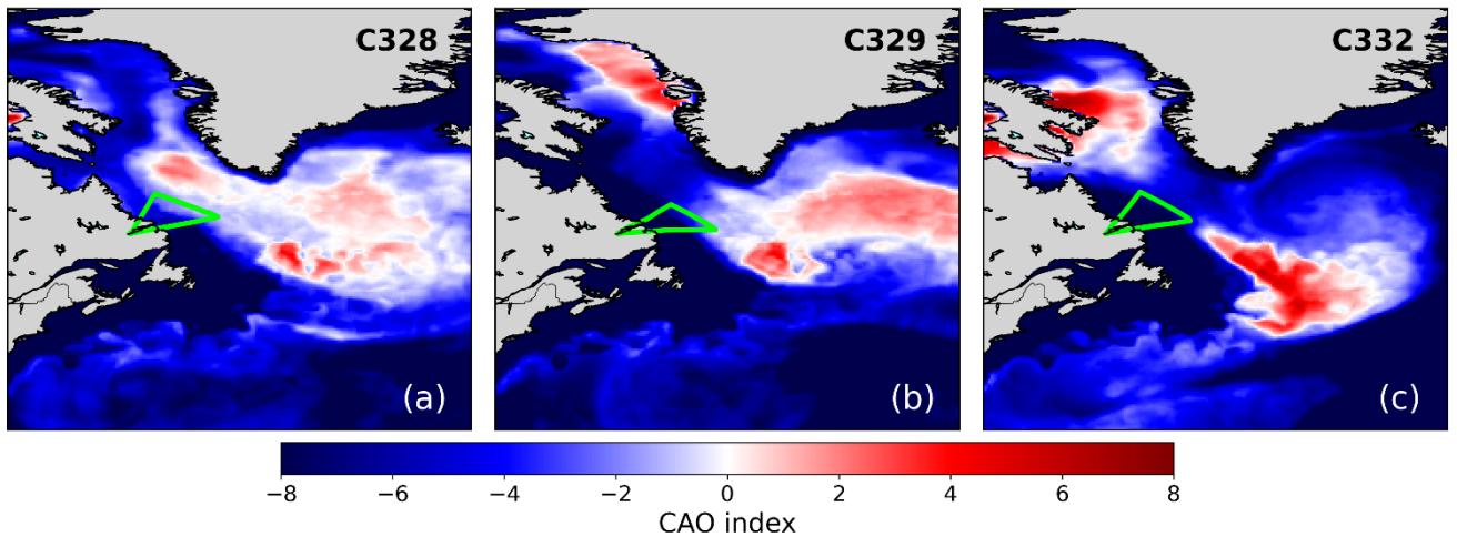
Figure B1: Mean CAO index values during M-Phase flights (a), C328, (b), C329, and (c) C332. Red and blue regions represent positive and negative index values, respectively. Flight tracks are overlaid (green lines).
