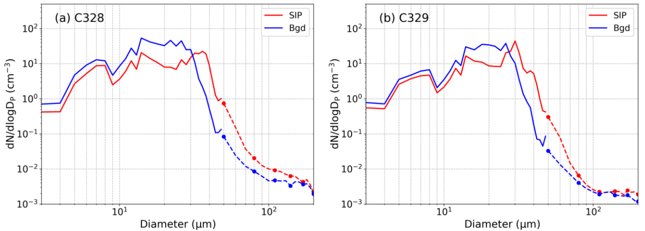
Figure 12: Mean cloud droplet size distributions measured with the CDP ( D_p < 50 \mu\text{m} ) for all SIP (red lines) and background ice periods (blue lines) during flights (a) C328, and (b) C329. 2D-S low irregular particle size distributions (dashed lines), used as proxy for large cloud droplets ( D_p > 50 \mu\text{m} ), are also provided.
