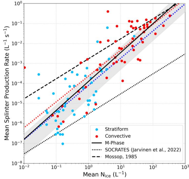
Figure 13: Mean splinter production rate ( \frac{dN_{ice}}{dt} ), calculated following Willis and Hallett (1991), as a function of mean measured ice particle concentrations for individual stratiform (blue) and convective (red) cloud segments with in-cloud temperatures within the H-M range of -3 to -8 °C. The solid black line represents the fit through the M-Phase data; the shaded region covers the area between fitting functions determined from maximum and minimum splinter production rates based on the overall relative uncertainty of \pm 86\% . The dashed and dotted black lines represent the relationships estimated by Mossop (1985) (wintertime cumulus clouds over Australia) and Järvinen et al. (2022) (summertime CAO clouds over Southern Ocean), respectively.
