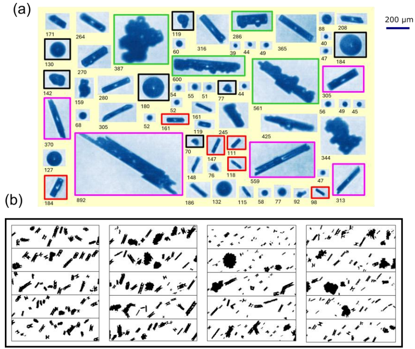
Figure C3: (a) Examples of cloud particles (ice crystals and liquid droplets) imaged with the CPI probe in SIP period 4 (between 14:11:25 and 14:13:03) during flight C329 (1 st November 2022); subsets of small columnar ice of size < 200 μm (red frames), long columns (pink frames), rimed columns (green frames), and possible frozen droplets and fragments of shattered droplets (black frames) are highlighted; numbers below images indicate the maximum dimension length ( D_p ) of each particle. (b) 2D-S images of highly irregular particles captured in SIP 4; the height of each strip corresponds to the 2D-S array width of 1280 μm.
