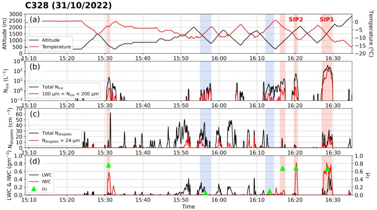
Figure 6: Time series of cloud microphysical properties (10 s averages) measured during flight C328 on 31 st October 2022 (transit leg data excluded), including (a) temperature (red line) and altitude (black line), (b) total ice crystal number concentration ( N_{\text{ice}} ; black line) and concentration of ice particles with diameter > 100 \mu\text{m} and < 200 \mu\text{m} (red line), (c) total cloud droplet concentration ( N_{\text{droplets}} ; black line) and concentration of cloud droplets with diameter > 24 \mu\text{m} (red line), and (d) liquid water content (LWC) and ice water content (IWC). SIP and background ice regions are shaded in red and blue, respectively. Mean ice mass fraction ( \mu_3 ) values for SIP and background ice periods are also marked in (d) (green triangles).
