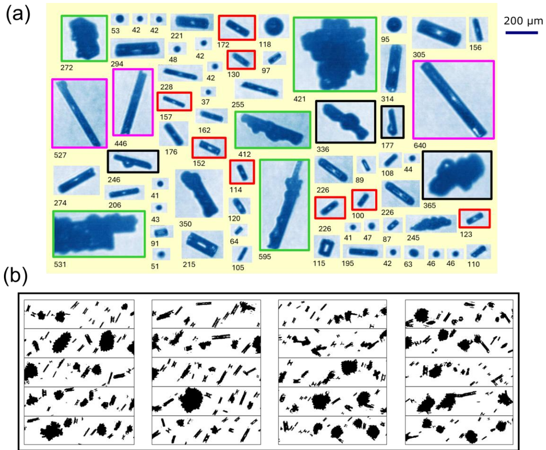
Figure 10: (a) Examples of cloud particles (ice crystals and liquid droplets) imaged with the CPI probe in SIP period 3 (between 13:26:45 and 13:29:18) during flight C329 (1 st November 2022); subsets of small columnar ice of size < 200 \mu\text{m} (red frames), long columns (pink frames), rimed columns and plates (green frames), and columns with frozen droplets attached (black frames) are highlighted; numbers below images indicate the maximum dimension length ( D_p ) of each particle. (b) 2D-S images of highly irregular particles captured in SIP 3; the height of each strip corresponds to the 2D-S array width of 1280 \mu\text{m} .
