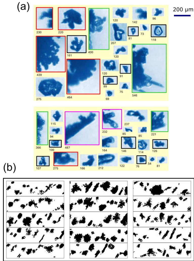
Figure 17: (a) Examples of cloud particles (ice crystals and liquid droplets) imaged with the CPI probe in two cloud segments (cloud top temperature \sim -18^\circ\text{C} ) during flight C326 (28 th October 2022); subsets of large rimed crystals with fragile branches (red frames), aggregates (green frames), large crystals with plate-like extensions (pink frames), and small, irregular ice fragments (black frames) are highlighted; numbers below images indicate the maximum dimension length ( D_p ) of each particle. (b) 2D-S images of highly irregular particles captured in both cloud segments; the height of each strip corresponds to the 2D-S array width of 1280 \mu\text{m} .
