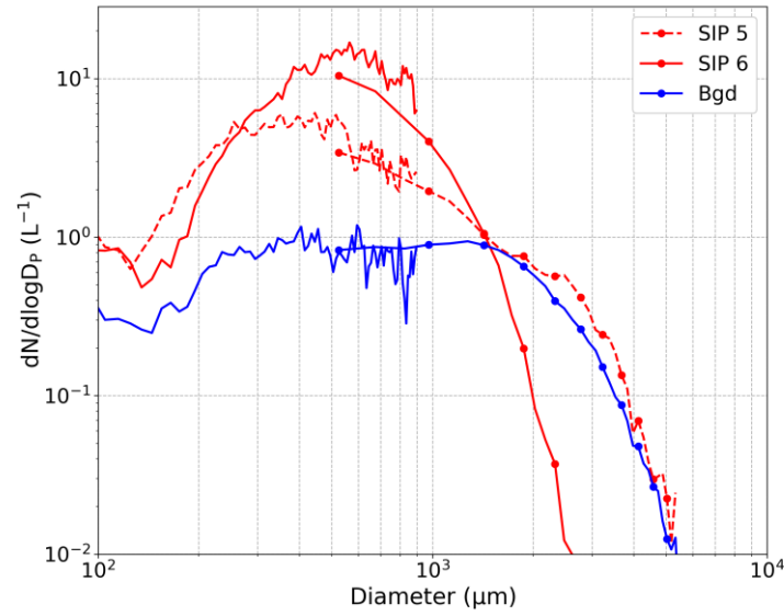
Figure 16: Mean composite (2D-S and HVPS) ice particle size distributions for SIP periods 5 (between 17:55:40 and 17:56:08) and 6 (between 19:34:40 and 19:35:10) (red lines) during flight C326 (28 th October 2022), and all background ice periods (blue line). HVPS data shown by lines with markers for particle sizes > 600 \mu\text{m} .
