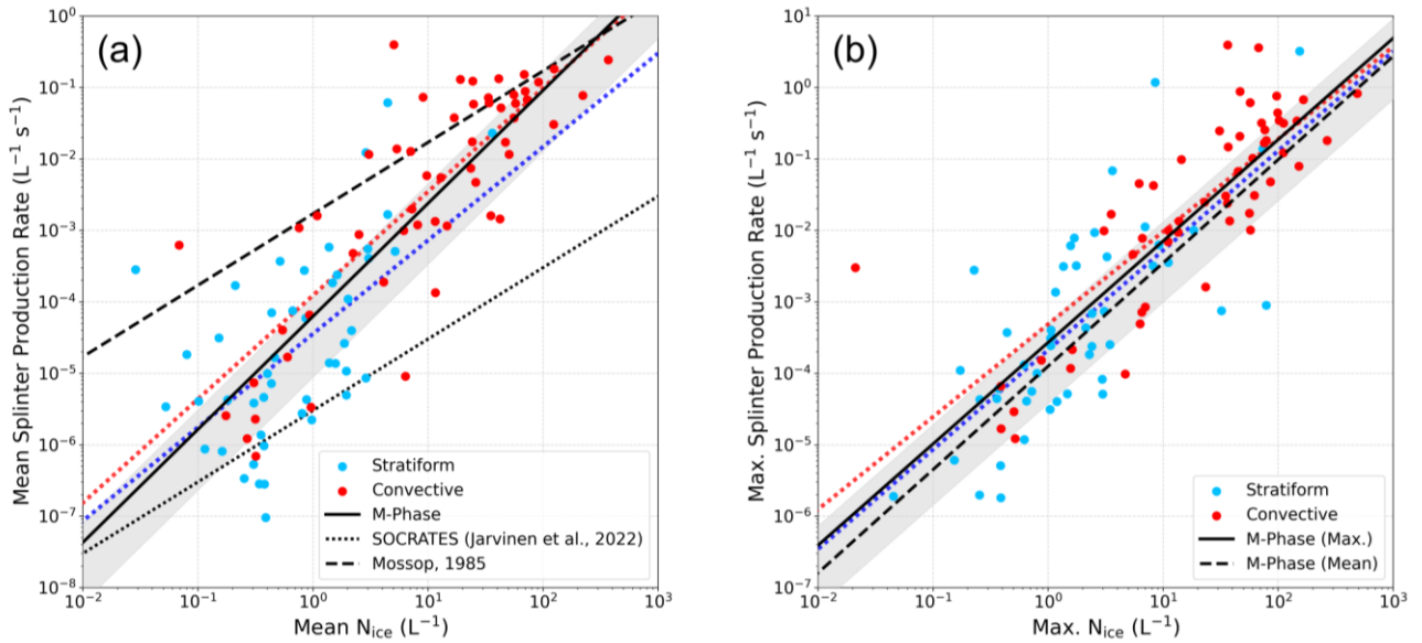
Figure D1: (a) Mean splinter production rate ( \frac{dN_{ice}}{dt} ), calculated following Willis and Hallett (1991), as a function of mean measured ice particle concentrations (including particles with D_p < 100 \mu m ) for individual stratiform (blue) and convective (red) cloud segments with in-cloud temperatures within the H-M range of -3 to -8 °C. The solid black line represents the fit through the M-Phase data; the shaded region covers the area between fitting functions determined from maximum and minimum splinter production rates based on the overall relative uncertainty of \pm 86 \% . The dashed and dotted black lines represent the relationships estimated by Mossop (1985) (wintertime cumulus clouds over Australia) and Järvinen et al. (2022) (summertime CAO clouds over Southern Ocean), respectively. (b) Maximum splinter production rate ( \frac{dN_{ice}}{dt} ) as a function of maximum measured ice particle concentrations. The solid black line represents the fit through the data shown here (maximum N_{ice} v maximum splinter production rate) for all cloud segments; the dashed black line shows the fit through the data for mean cloud segment values as shown in Fig. 13.
