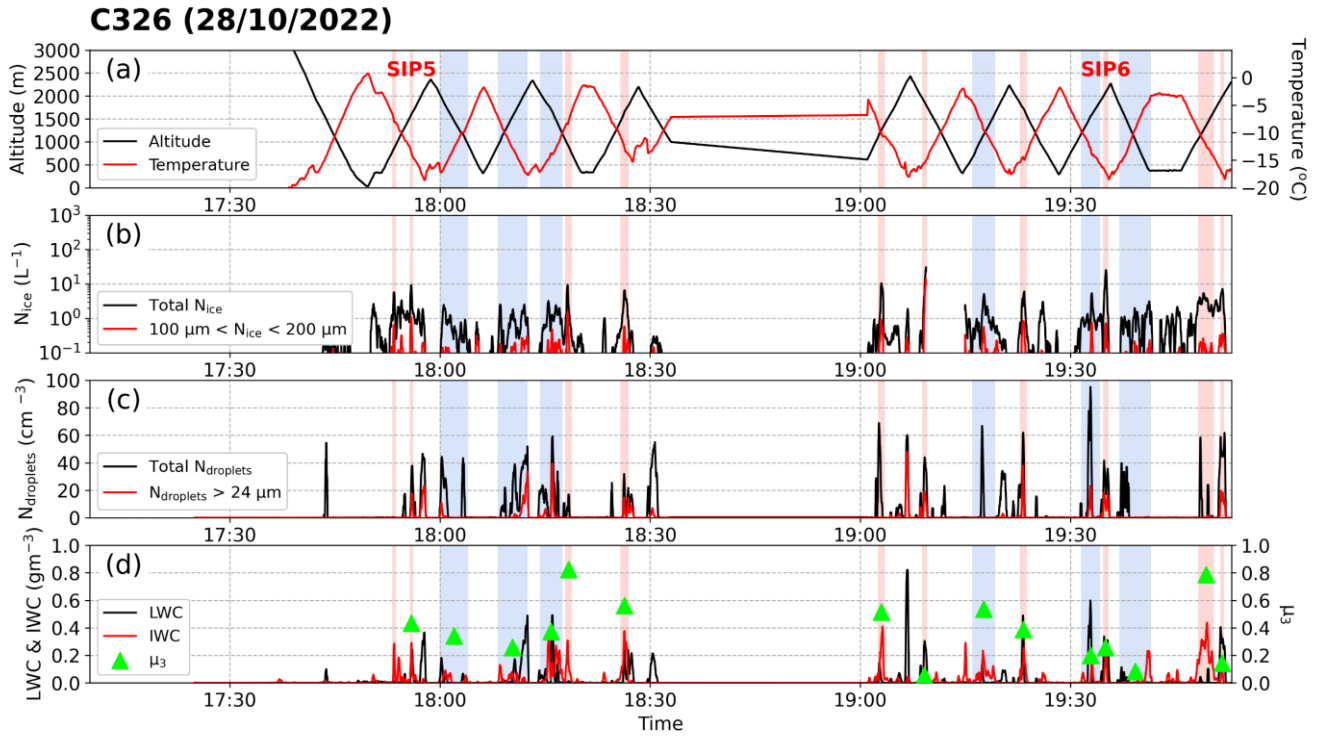
Figure 15: Time series of cloud microphysical properties (10 s averages) measured during flight C326 on 28 th October 2022 (transit leg data excluded), including (a) temperature (red line) and altitude (black line), (b) total ice crystal number concentration ( N_{ice} ; black line) and concentration of ice particles with diameter > 100 \mu\text{m} and < 200 \mu\text{m} (red line), (c) total cloud droplet concentration ( N_{droplets} ; black line) and concentration of cloud droplets with diameter > 24 \mu\text{m} (red line), and (d) liquid water content (LWC) and ice water content (IWC). SIP and background ice regions are shaded in red and blue, respectively. Mean ice mass fraction ( \mu_3 ) values for SIP and background ice periods are also marked in (d) (green triangles).
