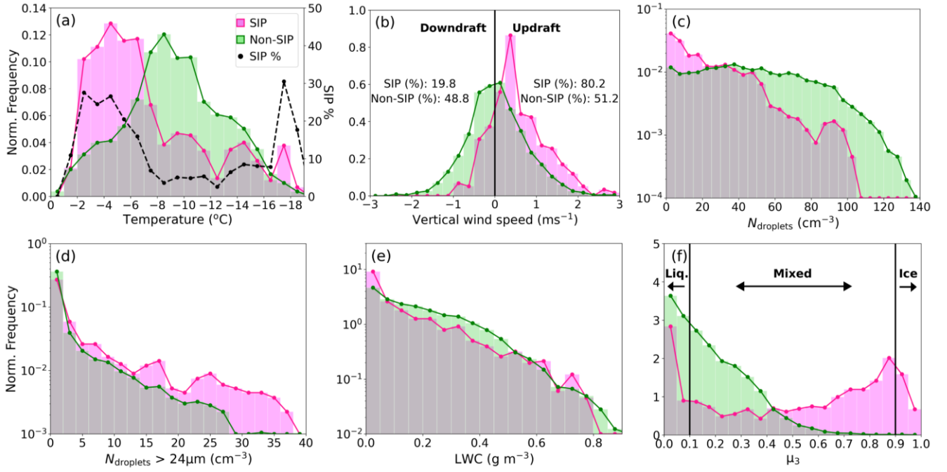
Figure 18: Relative frequency histograms of cloud microphysical properties (1 Hz data) measured within cloud regions containing strong evidence of active ice multiplication (SIP; pink), and those containing minimal evidence of active SIP processes (Non-SIP; green), including (a) local in-cloud temperature (percentage of total observations made during SIP periods within each 1°C temperature bin also marked with dashed black line), (b) vertical wind speed (straight-and-level runs only), (c) total cloud droplet concentration ( N_{\text{droplets}} ), (d) concentration of cloud droplets with diameter > 24 μm, (e) liquid water content (LWC), and (f) ice mass fraction ( \mu_3 ) with thresholds for liquid, mixed and ice phase cloud regions marked. Data normalised so that area under both SIP and Non-SIP histograms integrates to 1.
