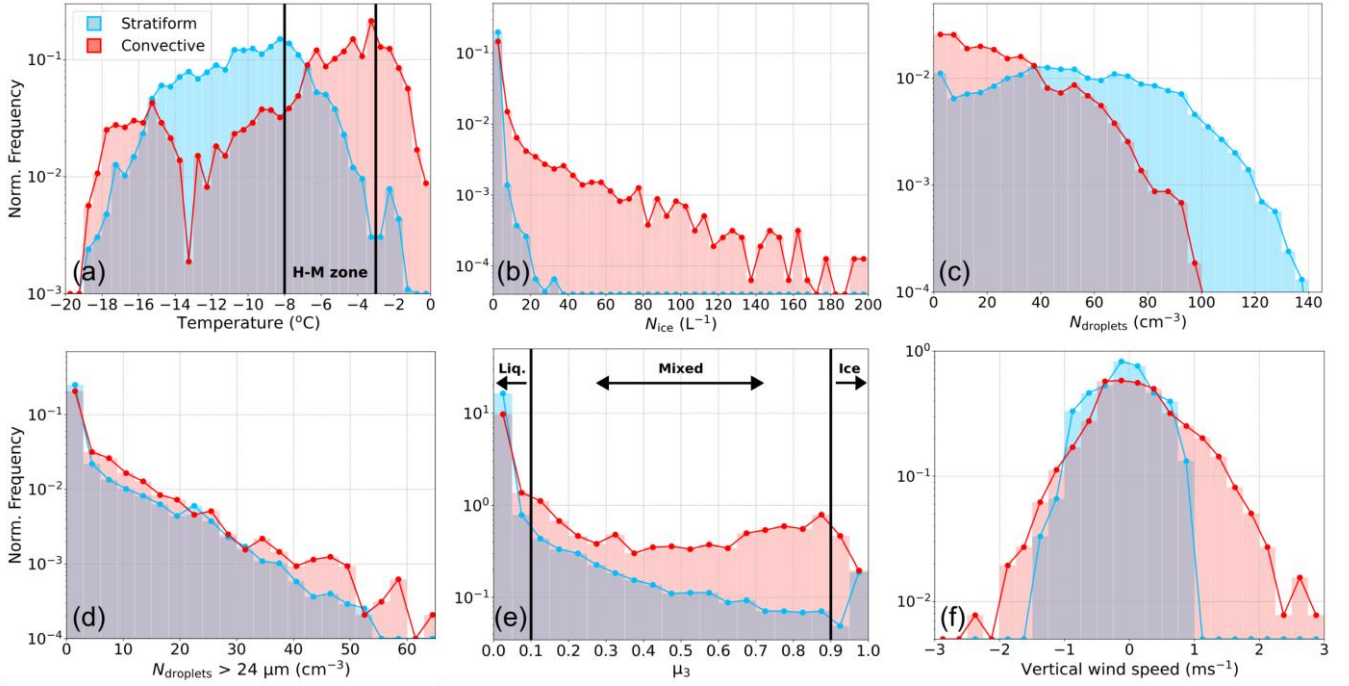
Figure 4: Relative frequency histograms of cloud microphysical properties (1 Hz data) measured within the stratiform (blue) and convective (red) regimes during all M-Phase CAO flights, including (a) local in-cloud temperature (H-M zone marked), (b) ice crystal number concentration ( N_{ice} ), (c) total cloud droplet concentration ( N_{droplets} ), (d) concentration of cloud droplets with diameter > 24 \mu m , (e) ice mass fraction ( \mu_3 ) with thresholds for liquid, mixed and ice phase cloud regions marked, and (f) vertical wind speed (straight-and-level runs only). Data is normalised so that area under both stratiform and convective histograms integrates to 1.
