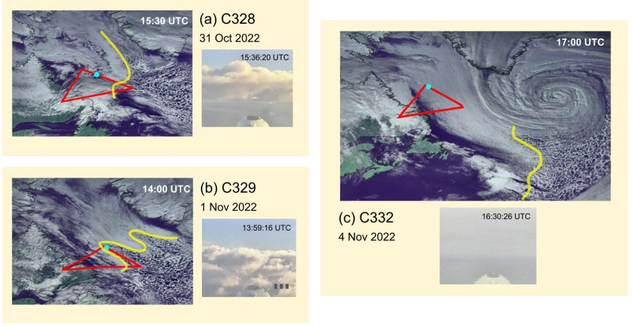
380 Figure 2: GOES-16 RGB composite satellite imagery, alongside images from the aircraft-mounted forward-facing camera, for M-Phase flights (a) C328, (b) C329, and (c) C332. Satellite overpass and camera image times are marked. Flight tracks are overlaid (red lines) and approximate locations of aircraft when camera image was captured are marked (blue circle). Yellow lines represent estimated location of stratiform-to-convective regime transition.
