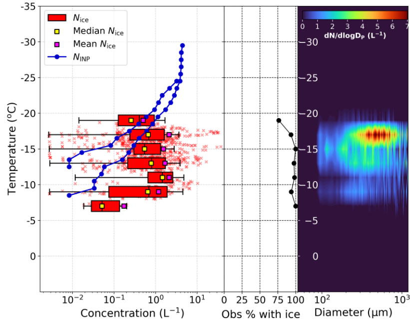
Figure 14: Measured total (2D-S + HVPS) ice crystal number concentrations ( N_{ice} ; red) as a function of local in-cloud temperature (1 Hz data) for flight C326 (28 th October 2022). Boxplots (red) for N_{ice} above the instrument detection limit in 2 °C temperature bins are composed of centre lines, edges and whiskers representing the median, interquartile range (25 th to 75 th percentile) and nearest data points within 1.5x interquartile range of the lower and upper quartiles, respectively. Median N_{ice} (yellow squares) and mean N_{ice} (pink squares) are calculated from all data points, including N_{ice} below the instrument detection limit (i.e. where we have set N_{ice} to 0 L -1 ). The percentage of ice concentration observations above 0 L -1 within each temperature bin is also provided (black line). Measured INP concentrations ( N_{INP} ) derived from filter samples collected during both flights are shown in blue. Mean ice particle size distributions as a function of local in-cloud temperature for both flights are presented in the right panel of (a) and (b).
