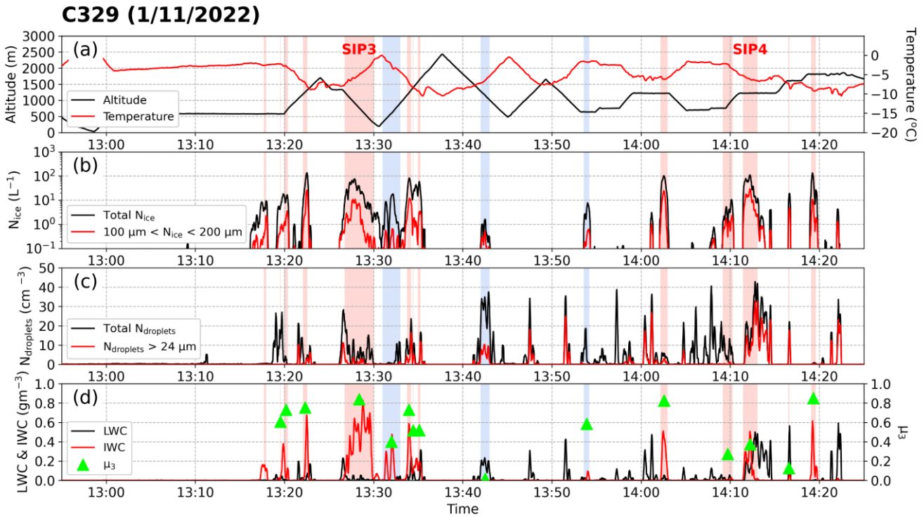
Figure 9: Time series of cloud microphysical properties (10 s averages) measured during flight C329 on 1 st November 2022 (transit leg data excluded), including (a) local temperature (red line) and altitude (black line), (b) total ice crystal number concentration ( N_{\text{ice}} ; black line) and concentration of ice particles with diameter > 100 \text{ }\mu\text{m} and < 200 \text{ }\mu\text{m} (red line), (c) total cloud droplet concentration ( N_{\text{droplets}} ; black line) and concentration of cloud droplets with diameter > 24 \text{ }\mu\text{m} (red line), and (d) liquid water content (LWC) and ice water content (IWC). SIP and background ice regions are shaded in red and blue, respectively. Mean ice mass fraction ( \mu_3 ) values for SIP and background ice periods are also marked in (d) (green triangles).
