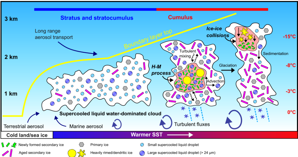
1040 Figure 19: A schematic diagram summarising the evolution of cloud morphology and microphysical properties within CAOs, moving downwind from the stratiform to the convective regime, over the Labrador Sea during the M-Phase campaign. Red regions within cumulus cloud segments contain representations of the dominant SIP mechanisms, inferred from in-situ airborne observations.
