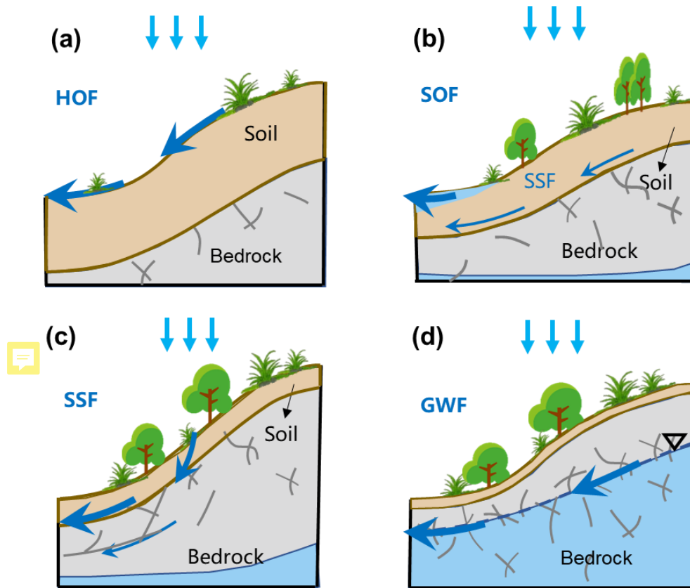
Figure A1. Conceptual schematic of runoff generation mechanism classes used in this review. HOF denotes infiltration-excess surface runoff; SOF denotes runoff from saturated or near-saturated source areas; SSF denotes event-scale lateral subsurface stormflow through soil, regolith, preferential pathways, or restrictive interfaces; and GWF denotes event-scale shallow groundwater response within weathered bedrock or fractured regolith contributing to stormflow. The schematic is intended to clarify classification terminology and does not imply that all catchments contain all pathways or that these mechanisms are mutually exclusive.
