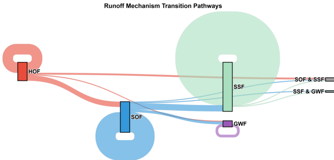
Figure 6. Sankey diagram illustrating reported runoff-mechanism transition pathways under-with increasing catchment wetness. The diagram includes only catchments for which studies with explicitly reported wetness-dependent mechanism shifts or persistence. Rectangular node height is proportional to the number of catchments with each initial mechanism. Directed band width is proportional to the number of catchments reporting each transition. Colored self-loop bands around a node indicate cases where the reported dominant mechanism remained unchanged under wetter conditions .
