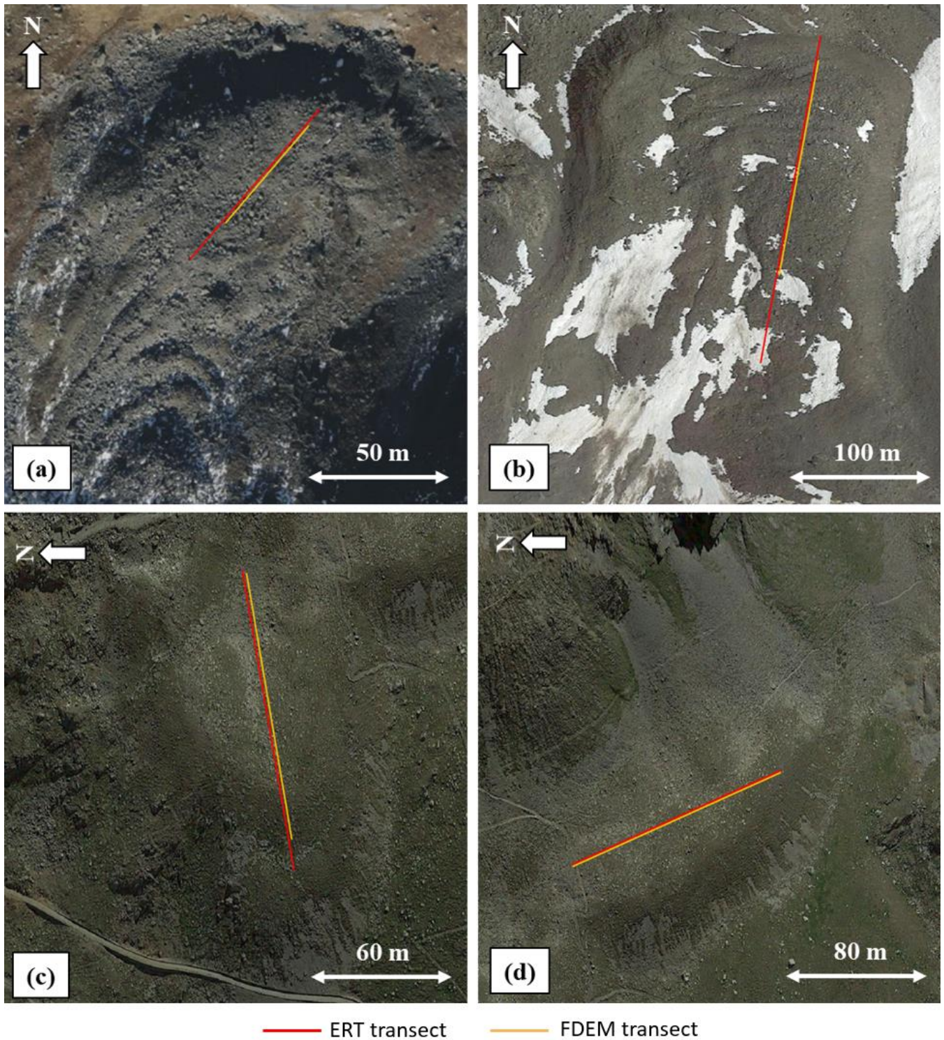
159 Figure 1. Satellite images of the study sites (Background imagery from Google Satellite; accessed via QuickMapServices in QGIS; 160 Imagery © Google; map data © Google) showing the ERT (red lines) and FDEM (orange lines) survey profiles. (a) Active rock 161 glacier at Flüela Pass (Switzerland; 46.746° N, 9.951° E). (b) Active rock glacier at Stelvio Pass (Italy; 46.527° N, 10.441° E). (c) Le 162 Rese di Scorluzzo inactive rock glacier at Stelvio Pass (Italy; 46.531° N, 10.420° E). (d) Le Rese di Scorluzzo inactive protalus rampart 163 at Stelvio Pass (Italy; 46.530° N, 10.421° E).
