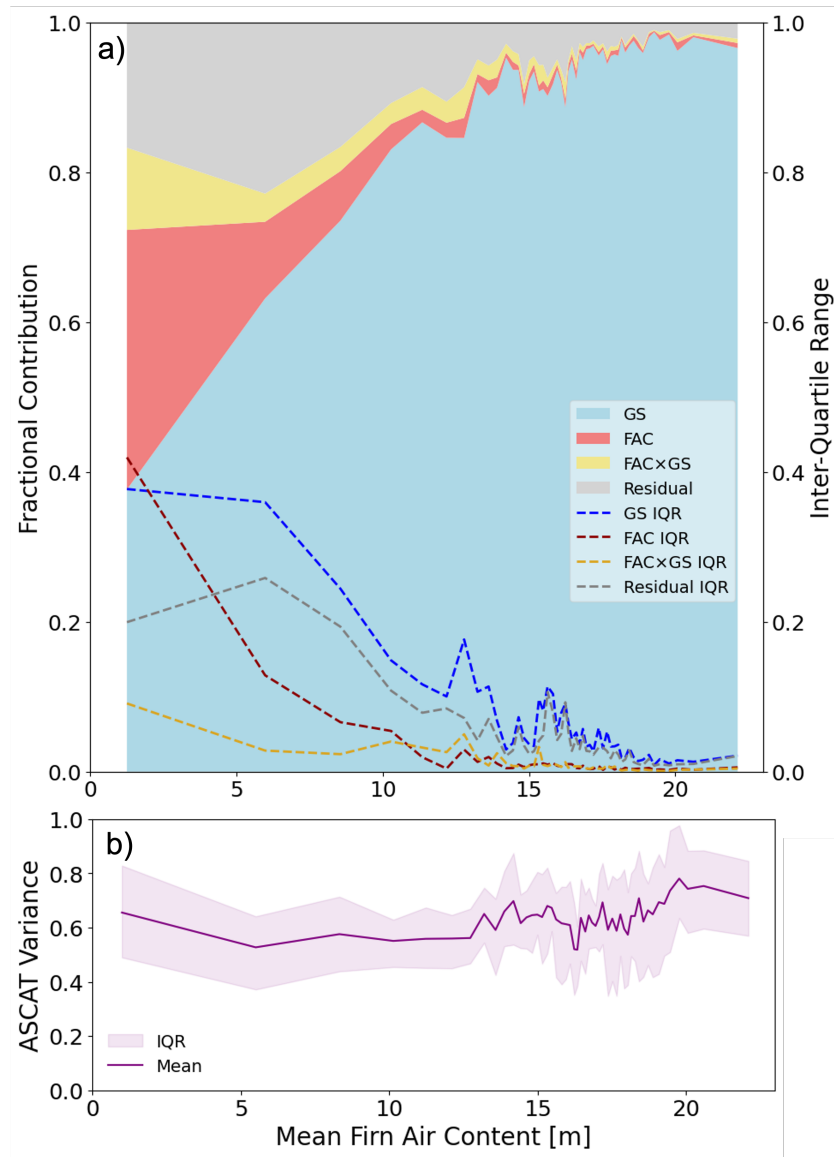
Figure 5. a) Fractional variance contributions to interannual ASCAT backscatter within the adopted framework, associated with grain size, FAC, their interaction (FACxGS), and the residual component, with uncertainty represented by the IQR. b) Mean ASCAT variance in dB as a function of mean FAC.
