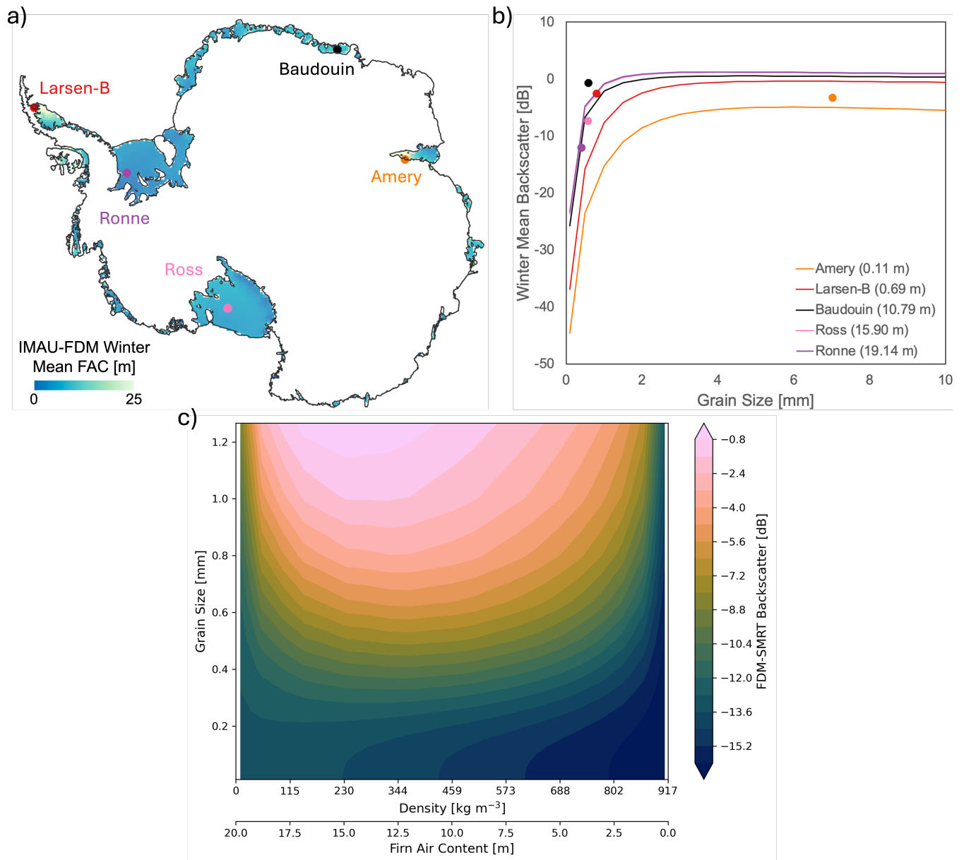
Figure 2. (a) 2007 – 2021 IMAU-FDM winter mean FAC at the Antarctic-ice-shelf-wide scale. Five representative 27 km grid cells are shown using site-specific colors. (b) FDM-SMRT-simulated winter-mean backscatter as a function of prescribed effective grain size for the five sites. Colored circles show the observed ASCAT backscatter plotted at the corresponding IMAU-FDM grain size. Site colors are consistent between panels (a) and (b). In the legend, the winter mean FAC values from IMAU-FDM are noted in brackets for the respective locations. (c) 2-D sensitivity of FDM-SMRT simulated backscatter in color to grain size and density/FAC.
