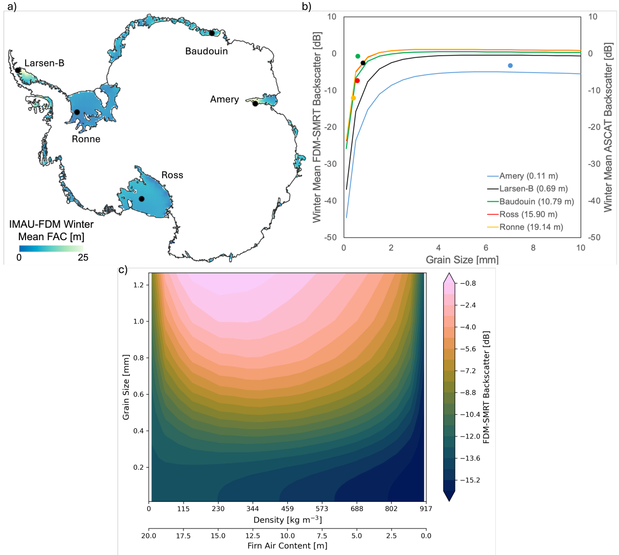
Figure 2. (a) 2007 – 2021 IMAU-FDM winter mean FAC at the Antarctic-ice-shelf-wide scale. Five samples are represented by black dots from Ross, Amery, Baudouin, Ronne, and Larsen-B ice shelves. (b) Sensitivity of FDM-SMRT simulated backscatter to grain size for five samples, as shown by coloured lines. The coloured dots represent the observed winter mean ASCAT backscatter and IMAU-FDM grain size for the corresponding sample. In the legend, the winter mean FAC values from IMAU-FDM are noted in brackets for the respective locations. (c) 2-D sensitivity of FDM-SMRT simulated backscatter in color to grain size and density/FAC.
