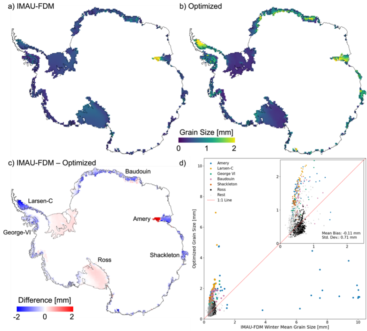
Figure 3. a) IMAU-FDM winter mean, b) Optimized, c) Difference (IMAU FDM - Optimized) grain size map, and d) Comparison between IMAU-FDM winter mean and Optimized grain size at AIS-wide Antarctic-ice-shelf-wide scale. Inset zooms the [2.5, 2.5] mm range where most of the points fall. The data points of all other ice shelves are categorized in “Rest” class, indicated by grey colour.
