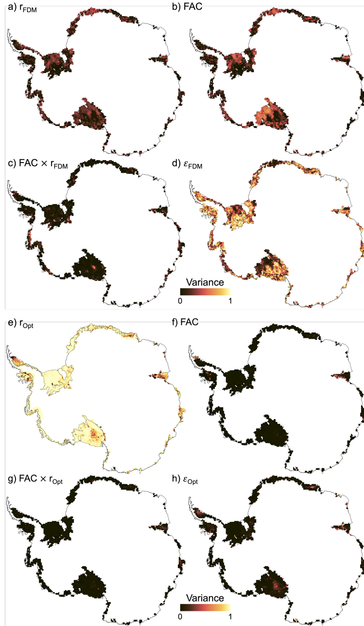
Figure B1. Spatial maps distribution of the fraction of fractional variance contributions to interannual ASCAT backscatter variance explained by within the adopted framework, associated with FAC, grain size ( r ) and their interaction, before and after grain-size optimization. Panels (a–d) show ANOVA using IMAU-FDM model grain size ( r_{\text{FDM}} ): (a) contribution of r_{\text{FDM}} , (b) of FAC, (c) their shared \text{FAC} \times r_{\text{FDM}} term, and (d) unexplained residual variance contribution ( \epsilon_{\text{FDM}} ). Panels (e–h) show the same decomposition after replacing r_{\text{FDM}} with our ASCAT-optimized grain size ( r_{\text{Opt}} ): (e) r_{\text{Opt}} , (f) FAC, (g) \text{FAC} \times r_{\text{Opt}} , and (h) unexplained residual variance contribution ( \epsilon_{\text{Opt}} ).
