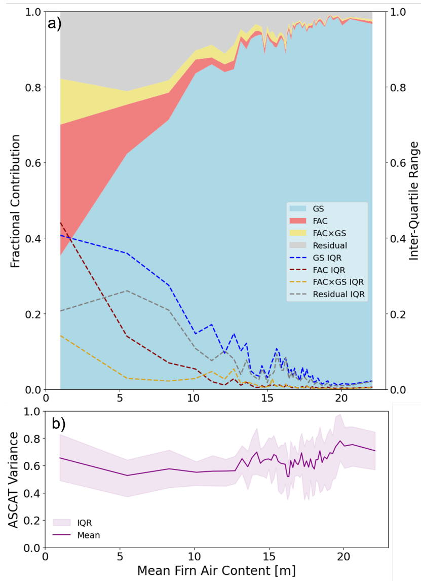
Figure 5. a) Fractional contribution of variance contributions to interannual ASCAT backscatter within the adopted framework , associated with grain size, FAC, their interaction (FAC x GS), and the unexplained-residual component, with uncertainty represented by the IQR. b) Mean ASCAT variance in dB as a function of mean FAC.
