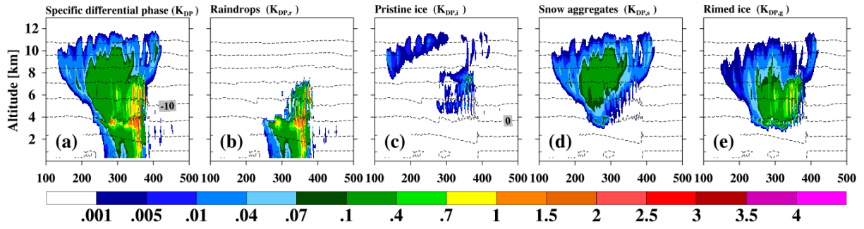
Fig. 11 Same as Fig. 9, but showing the specific differential phase at C band ( ^{\circ} \text{km}^{-1} ).
