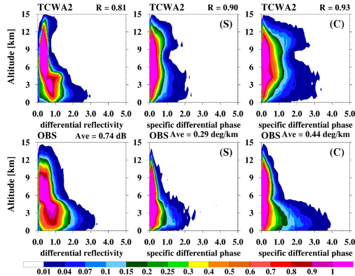
Fig. 16 Joint probability density distribution from the TCWA2 simulation (top row) and the corresponding observations (bottom row). The radar variables shown from left to right are differential reflectivity (dB), specific differential phase at S band ( ^{\circ} \text{ km}^{-1} ), and specific differential phase at C band ( ^{\circ} \text{ km}^{-1} ). The pattern correlation between simulated and observed distribution is indicated at the top of each panel, along with the observed mean values from the CWA measurements.
