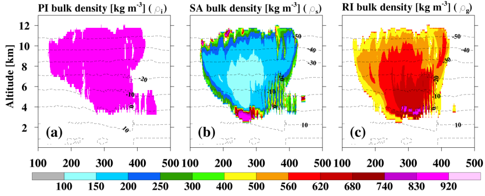
Fig. 6 Same as Fig. 3, but showing the bulk apparent density ( \text{kg m}^{-3} ) for (a) pristine ice, (b) snow aggregates, and (c) rimed ice.
