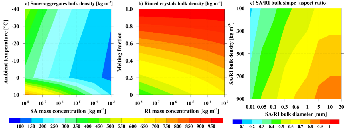
Fig. 2. Hydrometeor bulk density ( \text{kg m}^{-3} ) as a function of mass concentration ( \text{kg m}^{-3} ) for (a) snow aggregates against ambient temperature ( ^{\circ}\text{C} ), and (b) rimed ice against melting fraction. Bulk hydrometeor shape expressed as aspect ratio for snow aggregates and rimed ice, shown as a function of bulk density ( \text{kg m}^{-3} ) and bulk diameter (mm) in panel (c).
