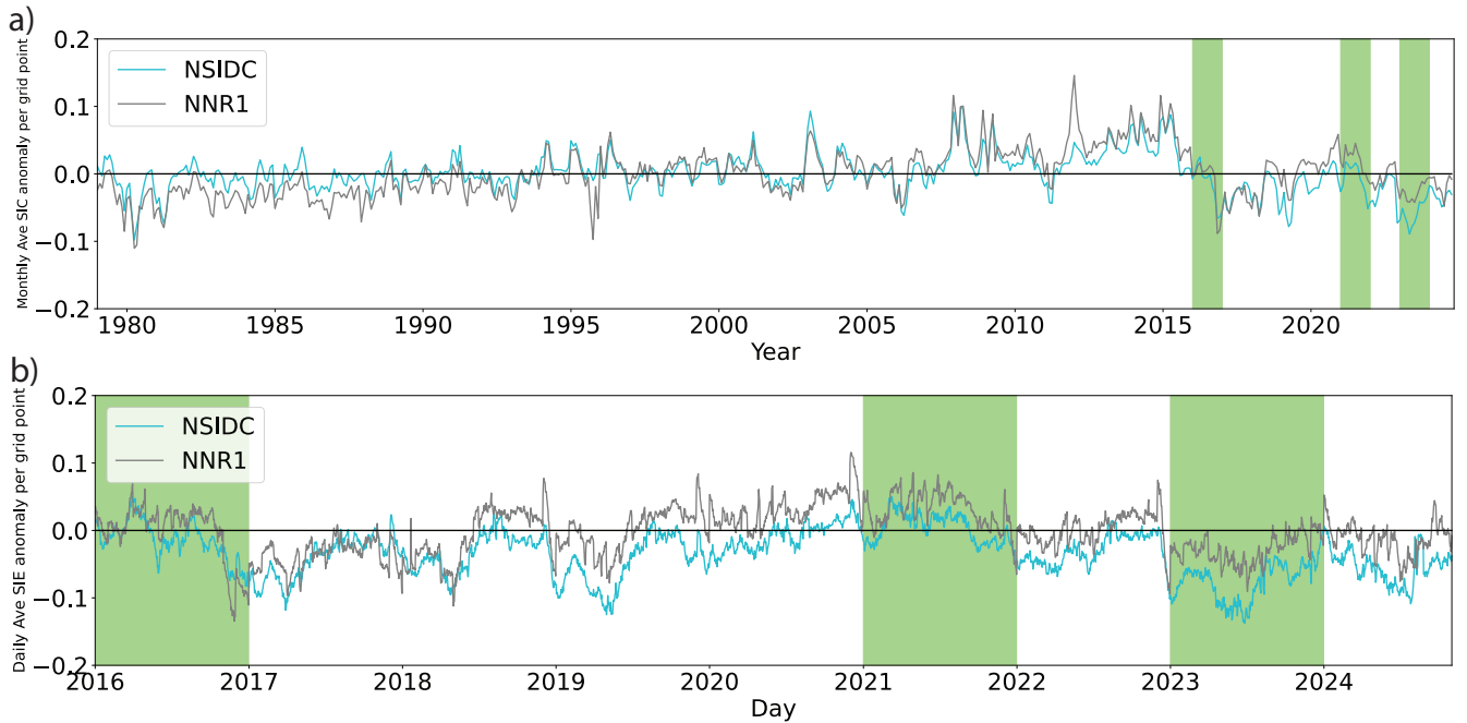
Figure 1. Panel a): A time series of monthly average anomalies in Antarctic sea ice concentration per grid point since 1979 in the Southern Hemisphere (assuming a 2.5^\circ \times 2.5^\circ resolution) for the NSIDC and NNR1 datasets. Data was converted (where appropriate) to latitude-longitude format, and then regridded to the given resolution using a linear interpolation method. Panel b): Time series of daily average anomalies in Antarctic sea ice extent per grid point over the years post January 1 st 2016 to October 31 st 2024. Shaded in green are the time periods considered for the study.
