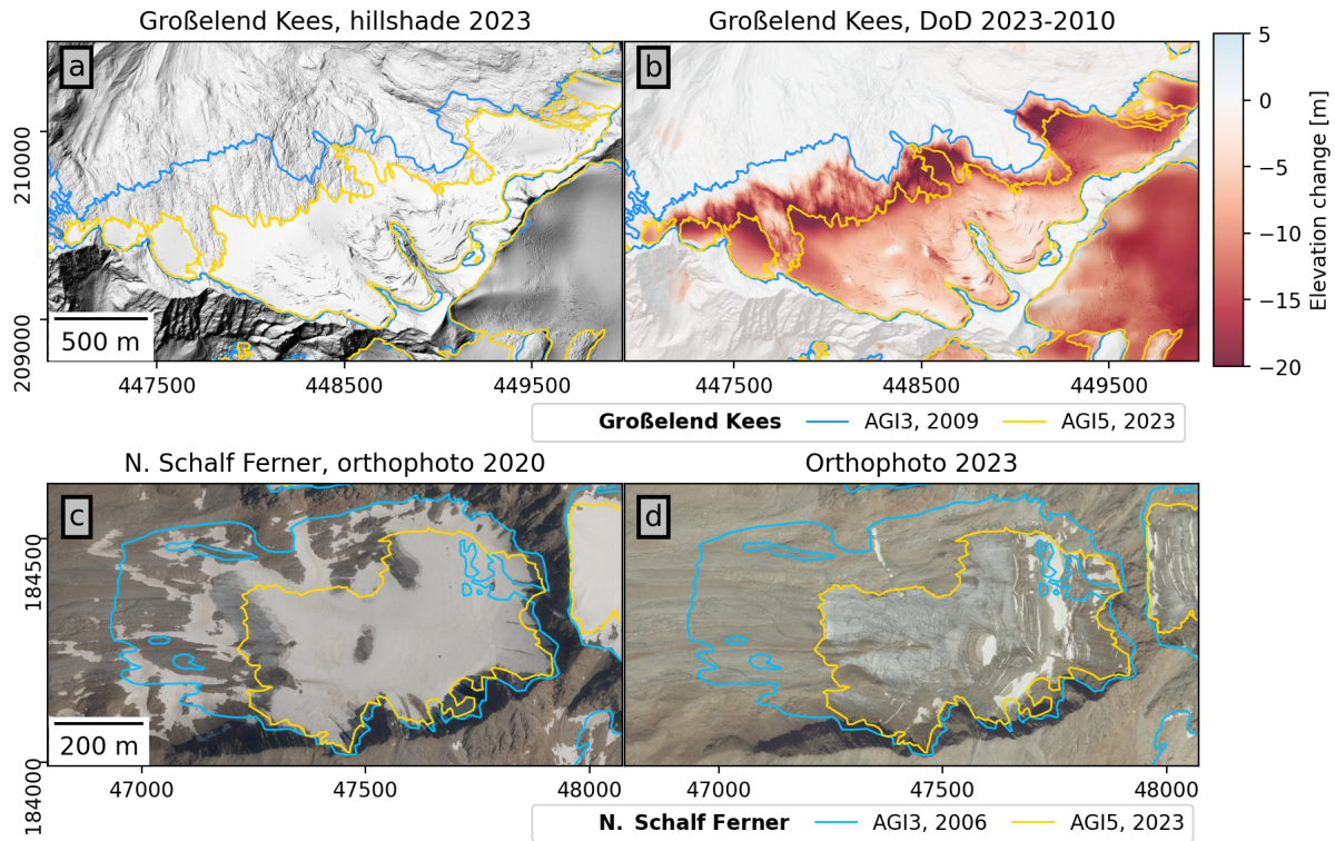
Figure 2. a: Großelend Kees (centroid coordinates: Lon. 13.315°, Lat. 47.025°; Ankogel-Hochalmspitze Group, region 2) as seen in a hillshade generated from a 2023 DEM (September 2023; Province of Carinthia, CC BY 4.0) b) Großelend Kees elevation change 2023-2010 overlaid on the hillshade (DoD: DEM of Differences). c, d: Multitemporal orthophotos of Nördlicher Schalf Ferner (centroid coordinates: Lon. 10.956°, Lat. 46.796°; Ötztal Alps, region 11; orthophotos: 28. July 2020, 19. August 2023; Province of Tyrol; CC BY 4.0 AT). a, b: EPSG: 31258; c, d: EPSG: 31287. Grid in meters. For additional information on data sources see Table S1 in the supplement.
