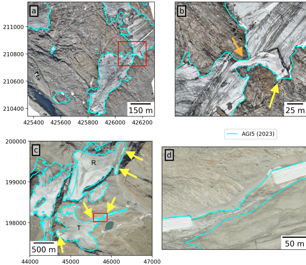
Figure 3. a: Wurtenkees Wurten Kees in the Goldberg Group with the Mölltaler Gletscher ski resort (Carinthia). The red box marks the subset shown in b. b: Zoomed in view of Wurtenkees Wurten Kees ; reflective coverings ( yellow arrow ) are applied to reduce ice melt in this sector in the vicinity of resort infrastructure. The orange arrow indicates a narrow connection between two sections of the glacier which is maintained by the resort operator through snow management measures. c: The ski resort of Sölden (Tyrol) maintains operates infrastructure and ski runs on glacierized terrain in the central Ötztal Alps, mainly on Tiefenbach Ferner (T) and Rettenbach Ferner (R). Yellow arrows indicate coverings near the glacier margins. The red box marks the subset shown in d. d: Reflective Close-up view of reflective coverings on the terminus of Tiefenbach Ferner and a narrow band of connecting ice between the two coverings. Blue lines indicate AGI5 outlines in all panels. Background image a, b: 2023 UAV orthophoto, courtesy of Geosphere Austria. c, d: 2023 orthophoto mosaic, Province of Tyrol (CC BY 4.0 AT).
