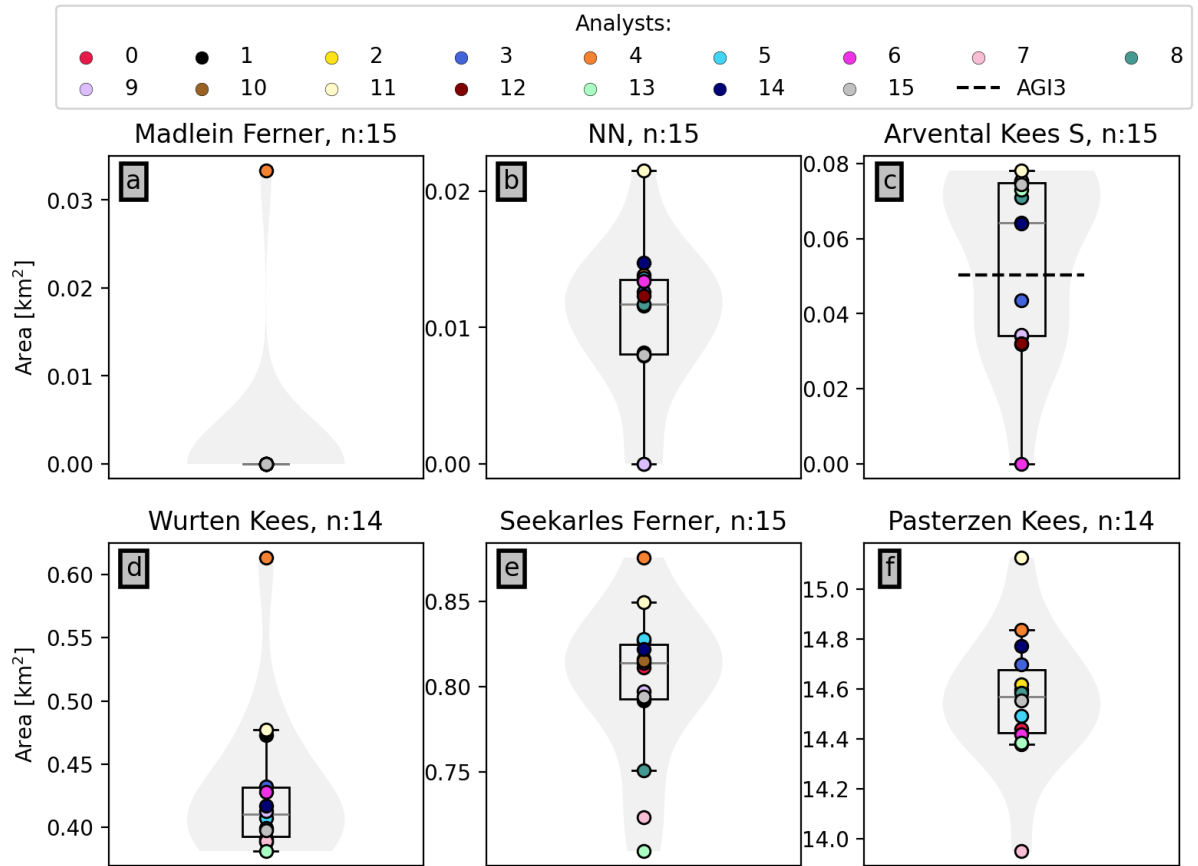
Figure 8. Glacier area derived from the outlines digitized by the analysts ( n =number of analysts) for the six test cases in the RR experiment. Grey-The boxplots indicate the first and third quartiles (black boxes) and the median (grey line); grey shading denotes the corresponding violin plots. In panel c, the AGI3 area (dashed black line) is included for comparison because the AGI5 outlines were mapped beyond the extent of the AGI3 outlines in this case. The AGI3 area was larger than all RR results for the other examples shown.
