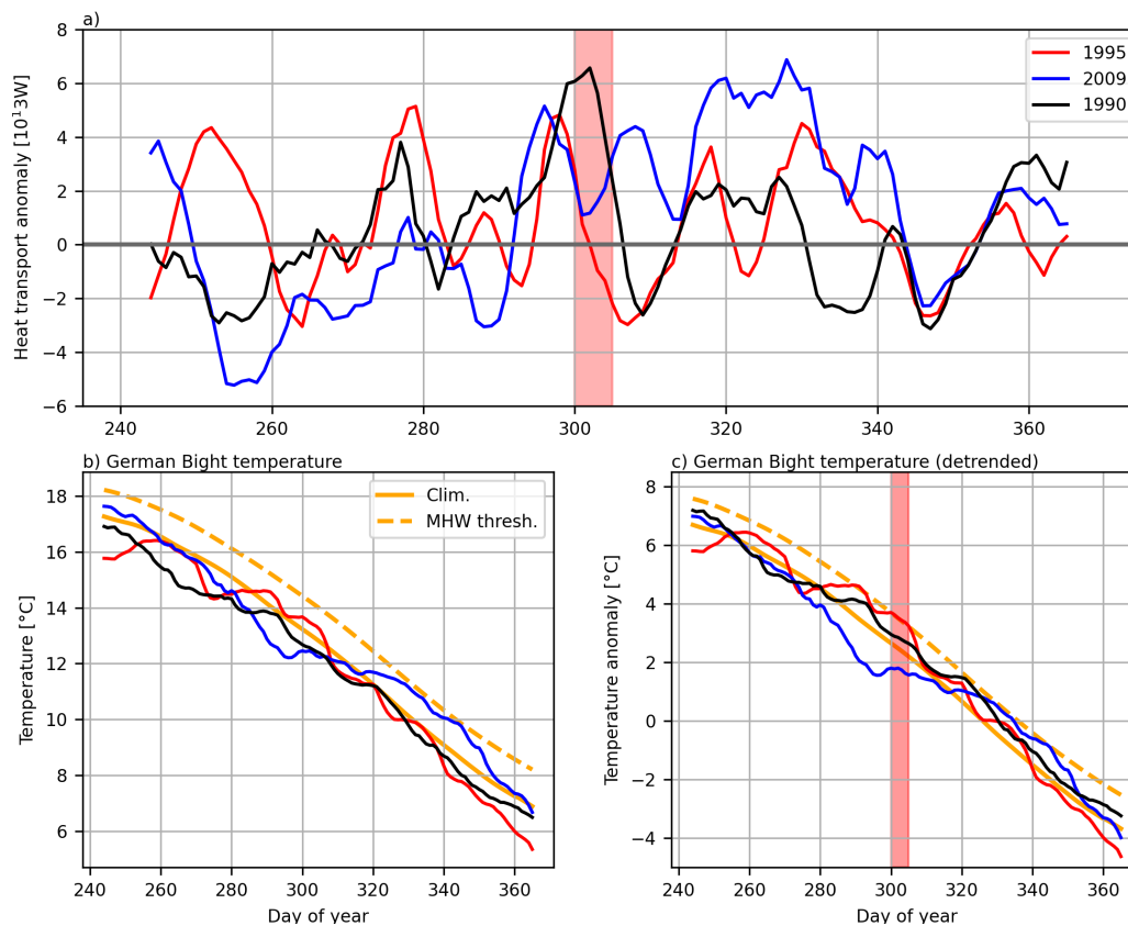
Figure A4. Heat transport anomaly trough through the English Channel (Dover Strait) in autumn of three selected years (a). Red shading indicates MHW days in the German Bight in 1995 (in 2009 and 1990 no MHW days have occurred; detrended baseline). The temperature (b) and detrended temperature (c) for the same years are shown along with the respective climatologies and MHW thresholds for the fixed and detrended baselines.
