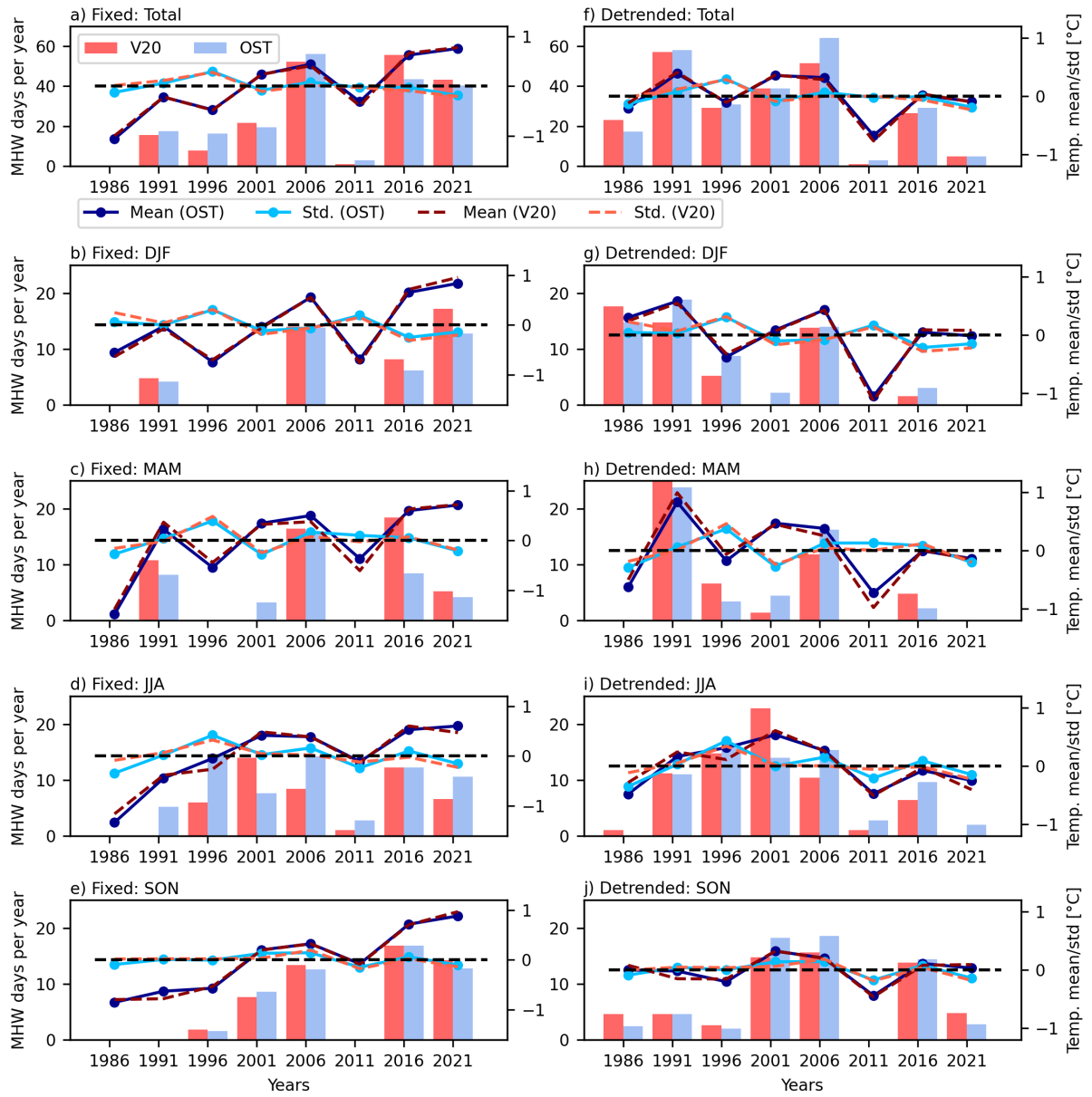
Figure 3. Average number of marine heatwave days per year (bars) in 5-year windows from VIKING20X and OSTIA (fixed baseline: a-e; detrended baseline f-j) in the German Bight . Labels on the x-axis indicate the center of the window. The mean temperature and standard deviation anomalies in the same 5-year windows are shown as lines. Panels a and f consider all days within the window, while b-f and g-j only those from the indicated months.
