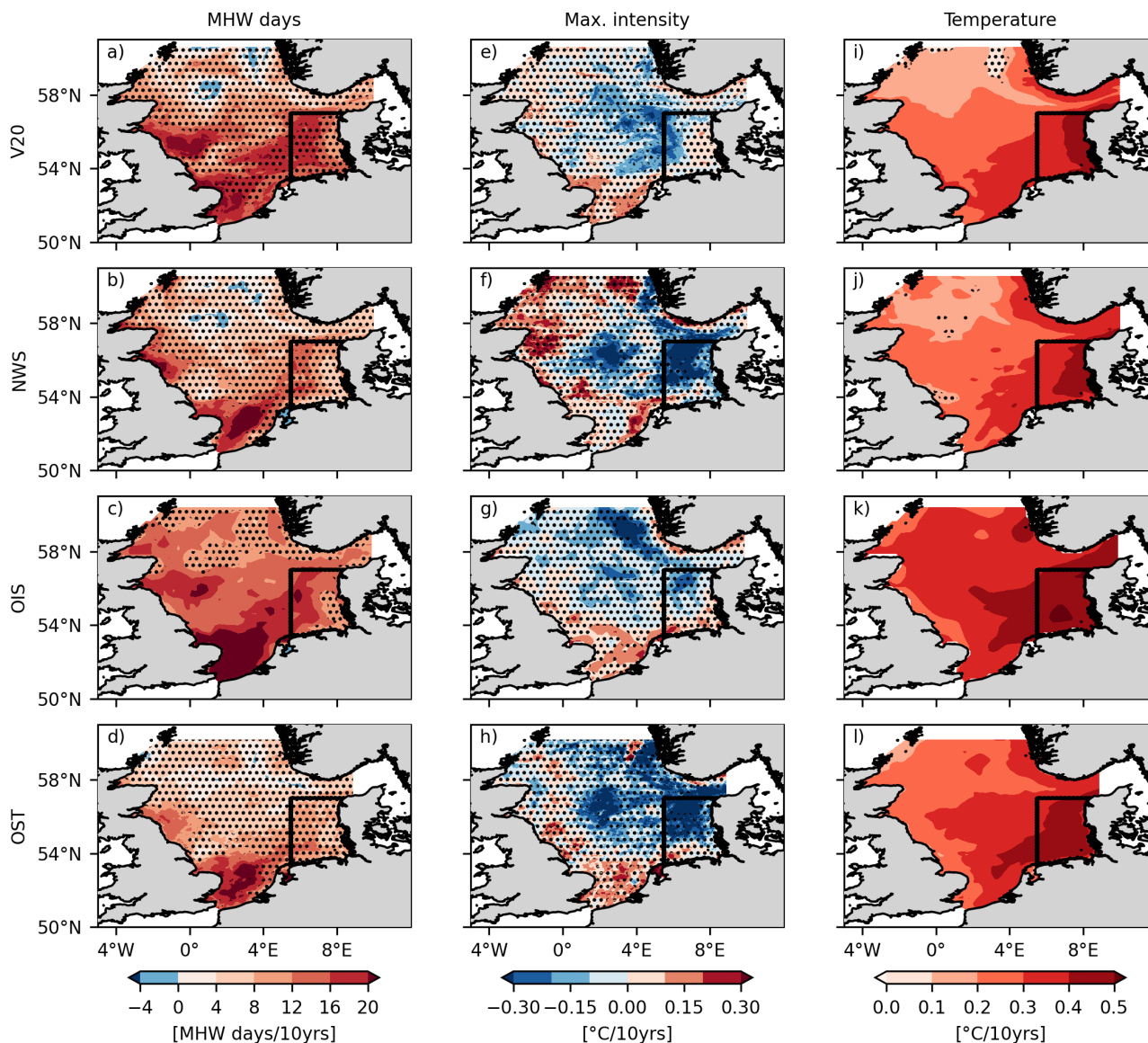
Figure 2. Linear trends (1993-2023) in MHW days per year (a-d), maximum intensity (e-h) and temperature (i-l) in VIKING20X, the European Northwest Shelf reanalysis, OISST and OSTIA. Slopes that are statistically different from zero (Non-significant slopes) based on a significance level of 5% are indicated by dots.
