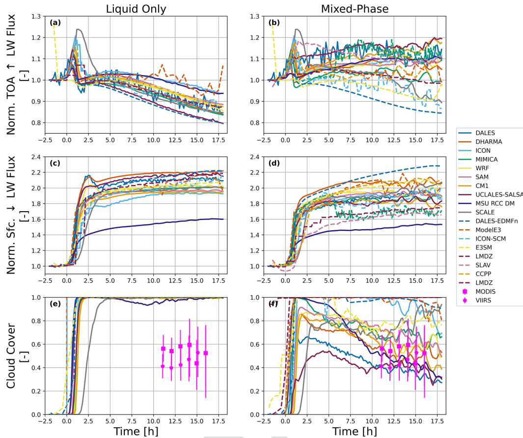
Figure 11. As in Fig. 10, except showing only model results that are normalized by the pre-cloud ( t = -1 h) values. In the bottom-most row, we also show the modeled cloud cover together with observational targets, inferred from satellites carrying the MODIS and VIIRS instruments. Identical to LES, cloud cover is computed as the portion of pixels with a cloud optical depth greater than 2.0.
