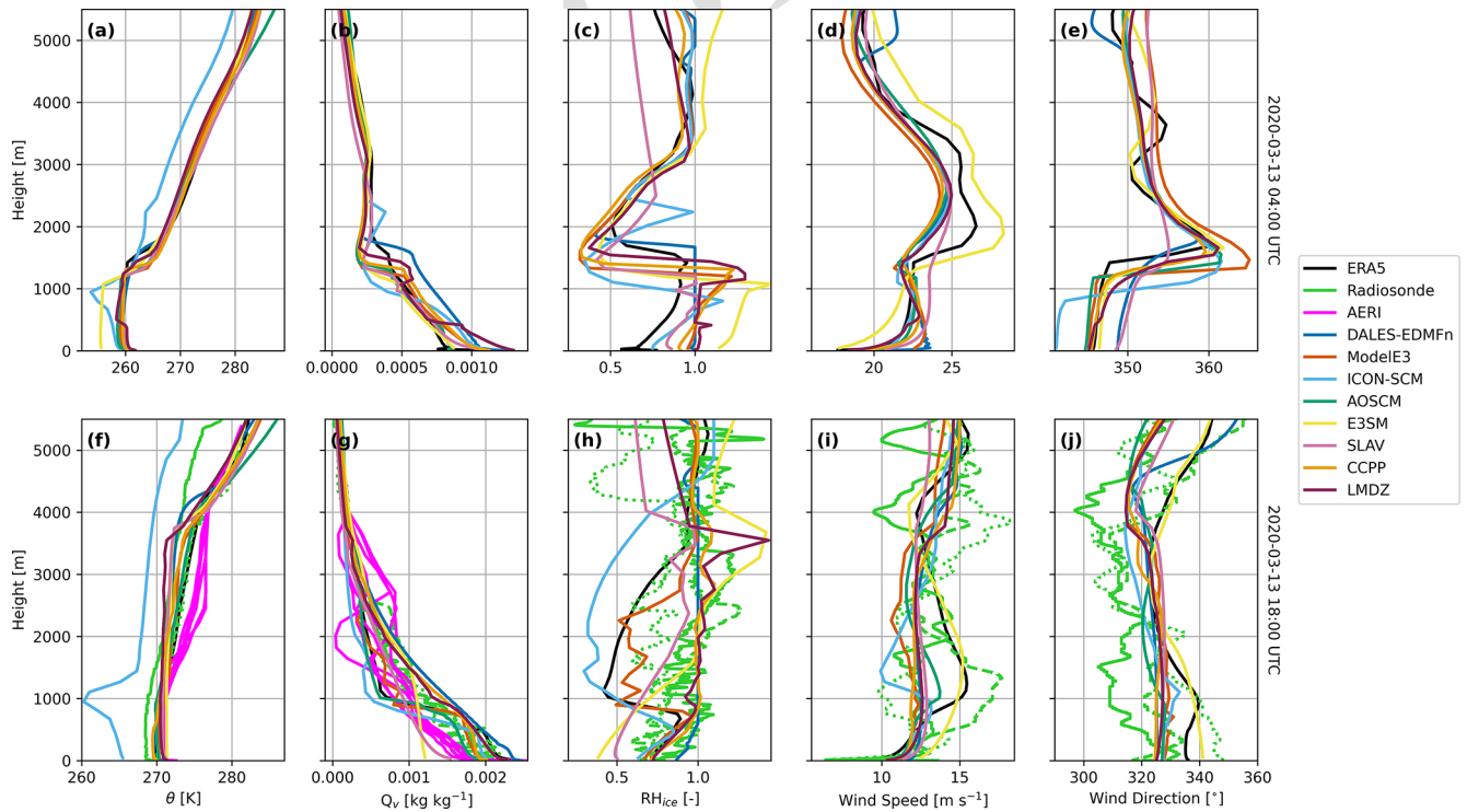
Figure 5. As in Fig. 4, except for the SCMs.
