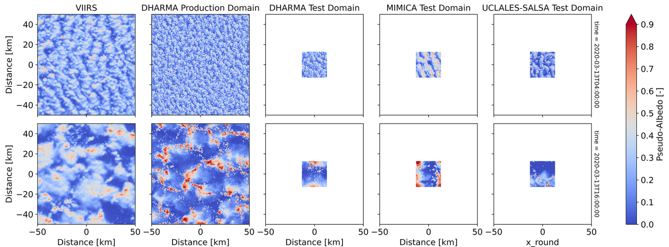
Figure 7. Pseudo-albedo comparison between VIIRS and DHARMA, MIMICA, and UCLALES-SALSA LES models at (top) 04:00 (rolls) and (bottom) 16:00 UTC (cells).
