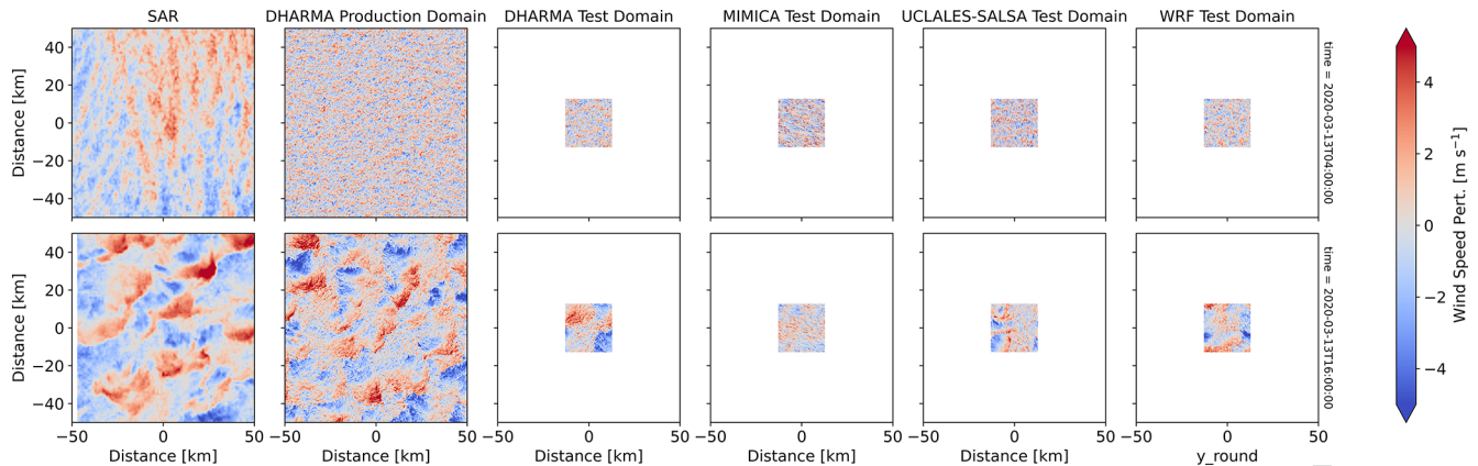
Figure 8. 10 m wind speed perturbation comparison between SAR and DHARMA, MIMICA, UCLALES-SALSA, and WRF LES models at (top) 04:00 (rolls) and (bottom) 16:00 UTC (cells). The 10 m wind speed perturbation field is computed by subtracting the domain-averaged value from each grid cell.
