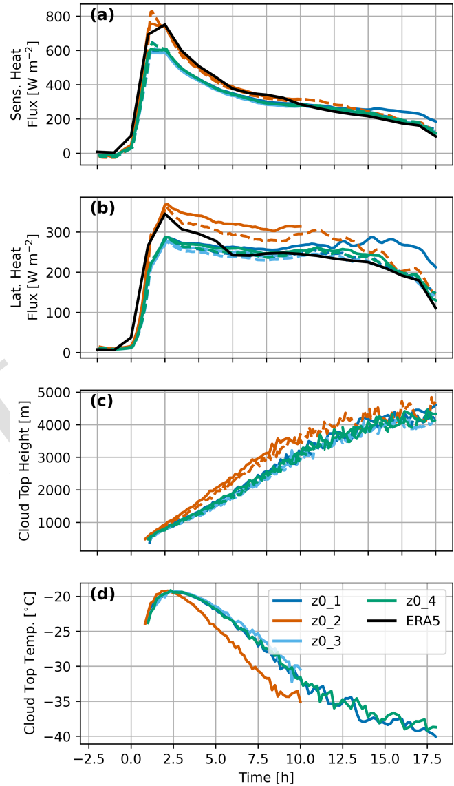
Figure B1. DHARMA LES output using various physics options. TSS
