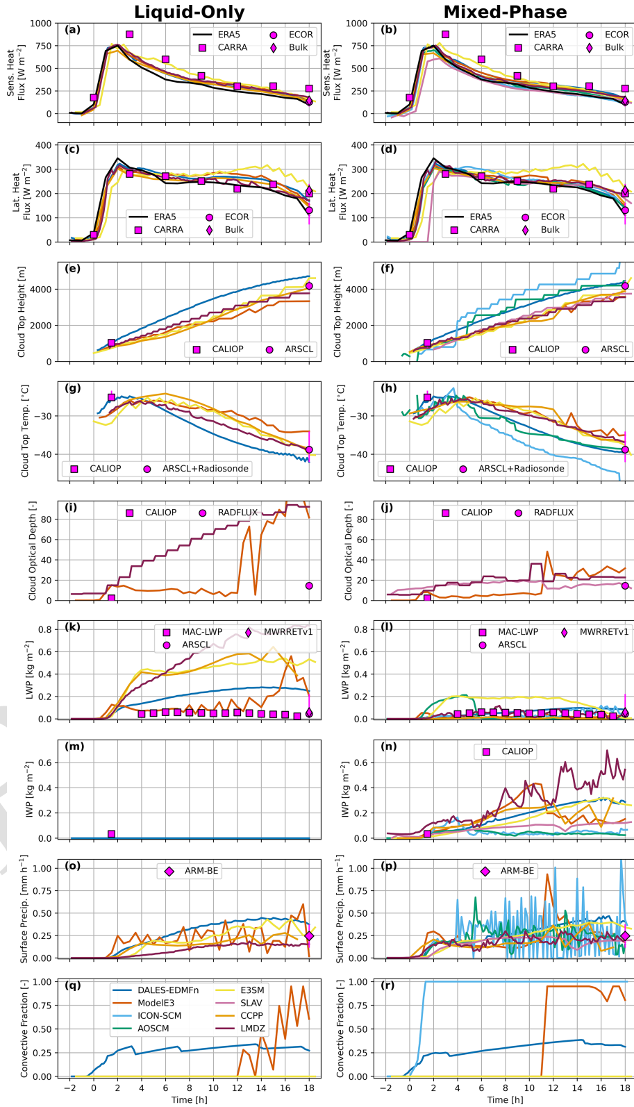
Figure 3. As in Fig. 2, except for the SCMs and the addition of of convective fraction.
