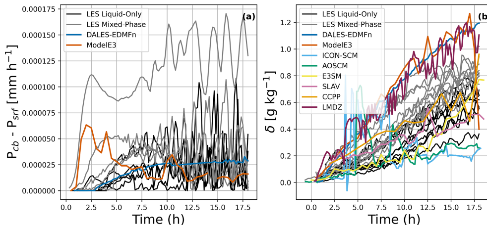
Figure 6. Cloud-base minus surface precipitation rate (left) and water vapor mixing ratio difference between the bottom and top of the MBL (i.e., 25 % and 75 % of cloud-top height, respectively) (right) over time. LES Liquid Only and LES Mixed-Phase simulations are shown in the black and gray lines respectively, with each line representing results from a single model, while the mixed-phase SCMs are colored according to the legend, noting that not all models reported precipitation flux profiles.
