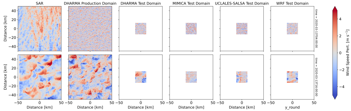
Figure 8. 10 m wind speed perturbation comparison between SAR and DHARMA, MIMICA , UCLALES-SALSA, and WRF LES models at (top) 0400 UTC (rolls) and (bottom) 1600 UTC (cells). The 10 m wind speed perturbation field is computed by subtracting the domain-averaged value from each grid cell.
