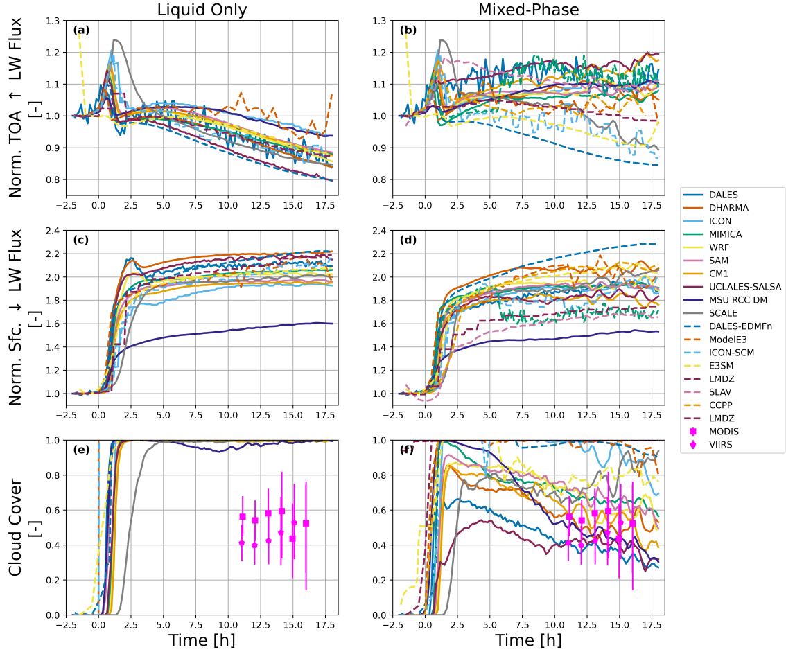
Figure 11. As in Fig. 109, except showing only model results that are normalized by the pre-cloud ( t=-1 h) values. In the bottom-most row, we also show the modeled cloud cover together with observational targets, inferred from satellites carrying the MODIS and VIIRS instruments . Identical to LES, cloud cover is computed as the portion of pixels with a cloud optical depth greater than 2.0.
