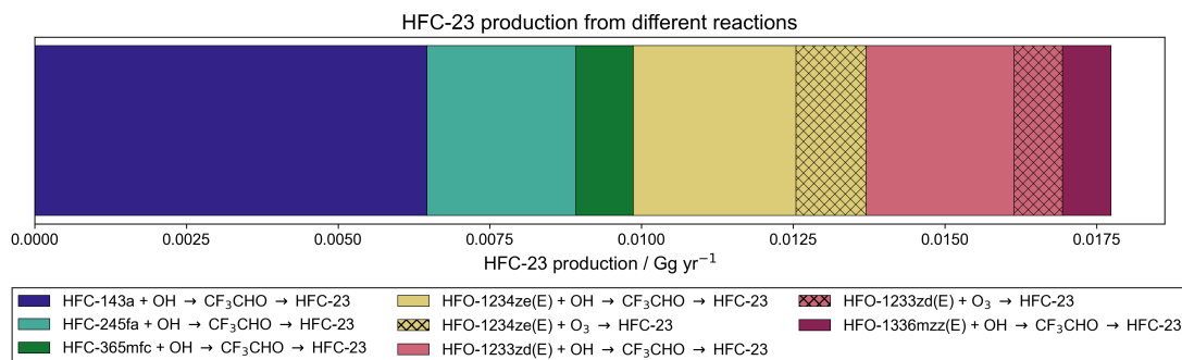
Figure 3. Plot of the contribution of each HFO reaction to in-atmosphere HFC-23 production in ‘base’ scenario. The \text{CF}_3\text{CHO} photolysis pathway reactions are shown as solid bars, while the contribution from ozonolysis is shown as hatched bars. The reaction of HFC-236fa with OH and that of HFO-1336mzz(Z) with ozone are not shown, as their contributions to total HFC-23 emissions are <0.1\% of the total.
