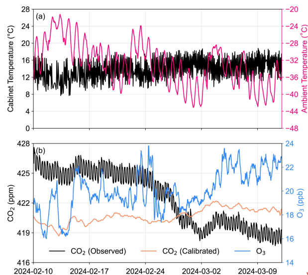
Fig. 4 Compares synchronous in-cabinet temperature (black, left axis) and outdoor ambient temperature (pink, right axis), (a), hourly average concentration of observed CO 2 , hourly average concentration of calibrated CO 2 and O 3 concentration transmitted from the unattended automated observation system at Taishan Station (b).
