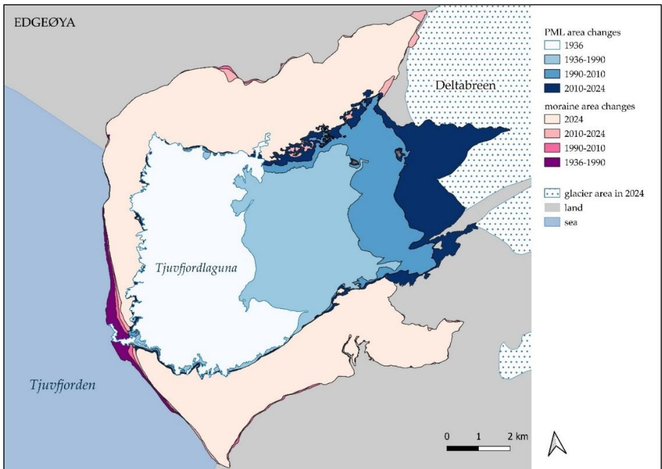
175 Figure 2: The map shows changes in the surface area of the Tjuvfjordlaguna and moraines over the years.
