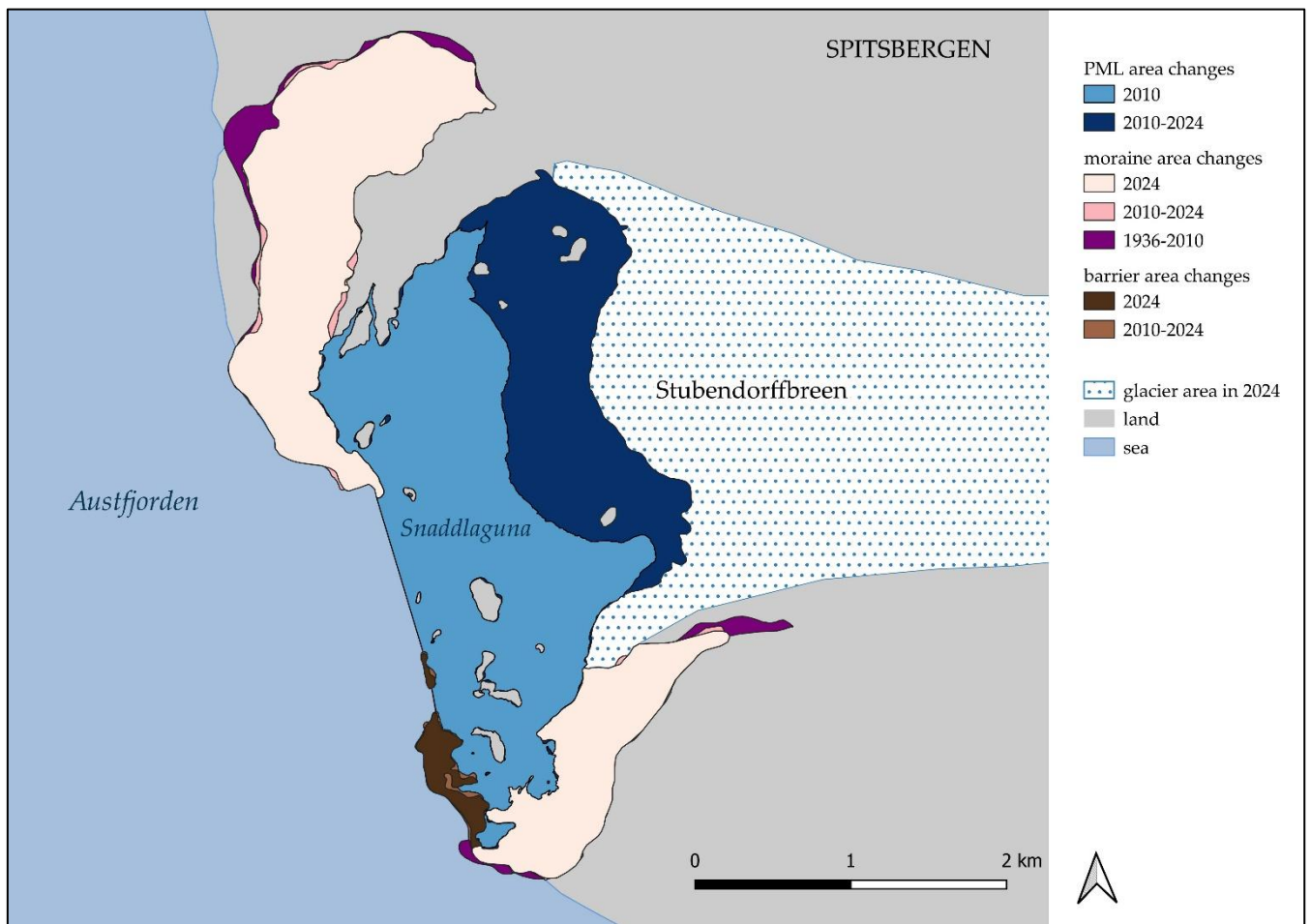
185 Figure 3: The map shows changes in the surface area of the Snaddlaguna, barriers, and moraines over the years.
