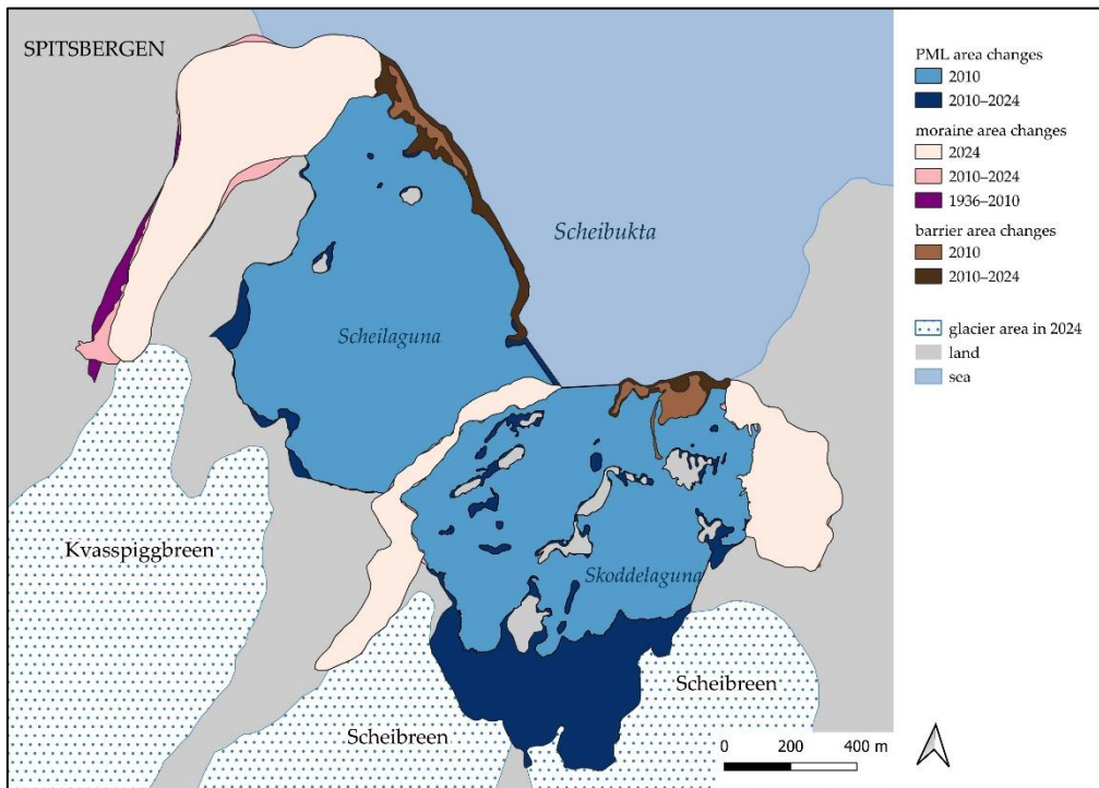
295 Figure 9: The map shows changes in the surface area of the two PLMs – Scheilaguna and Skoddelaguna – barriers and moraines over the years.
