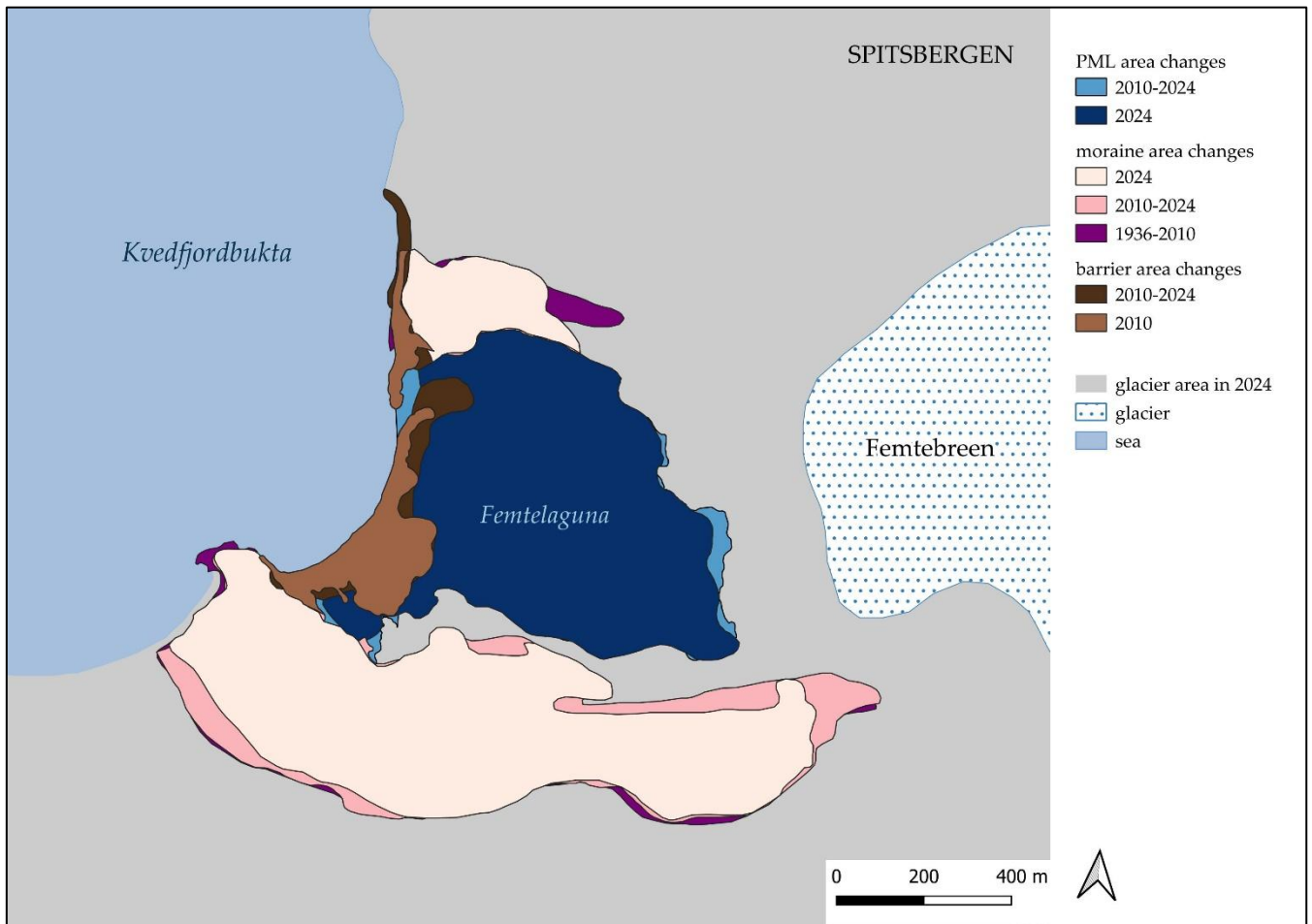
Figure 6: The map shows changes in the surface area of the Femtelaguna, barriers, and moraines over the years.
