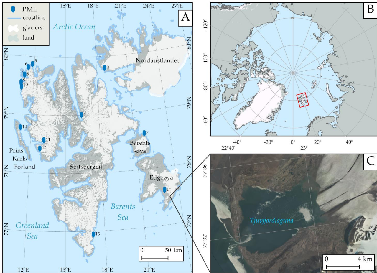
105 Figure 1: (A) PMLs' location on Svalbard. 1 – Tjuvfjordlaguna, 2 – Kapplaguna, 3 – Gimlelaguna, 4 – Snaddlaguna, 5 – Makarovlaguna, 6 – Rissalaguna, 7 – Schielaguna, 8 – Skodelaguna, 9 – Sjulaguna, 10 – Femtelaguna, 11 – Charleslaguna, 12 – Eidemlaguna, 13 – Tromsølaguna, 14 – Murraylaguna. (B) Svalbard (marked with a red rectangle) on an Arctic map. (C) The most representative paraglacial moraine lagoon in Svalbard – Tjuvfjordlaguna. Base map: 2010 orthophotomap from the Norwegian Polar Institute. 110
