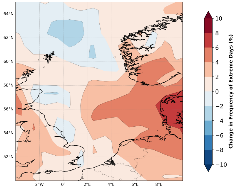
Figure 10. Change (%) in the frequency of wind speeds exceeding the control 90 th 90 th percentile over the North Sea (days 7–60, all selected years)
