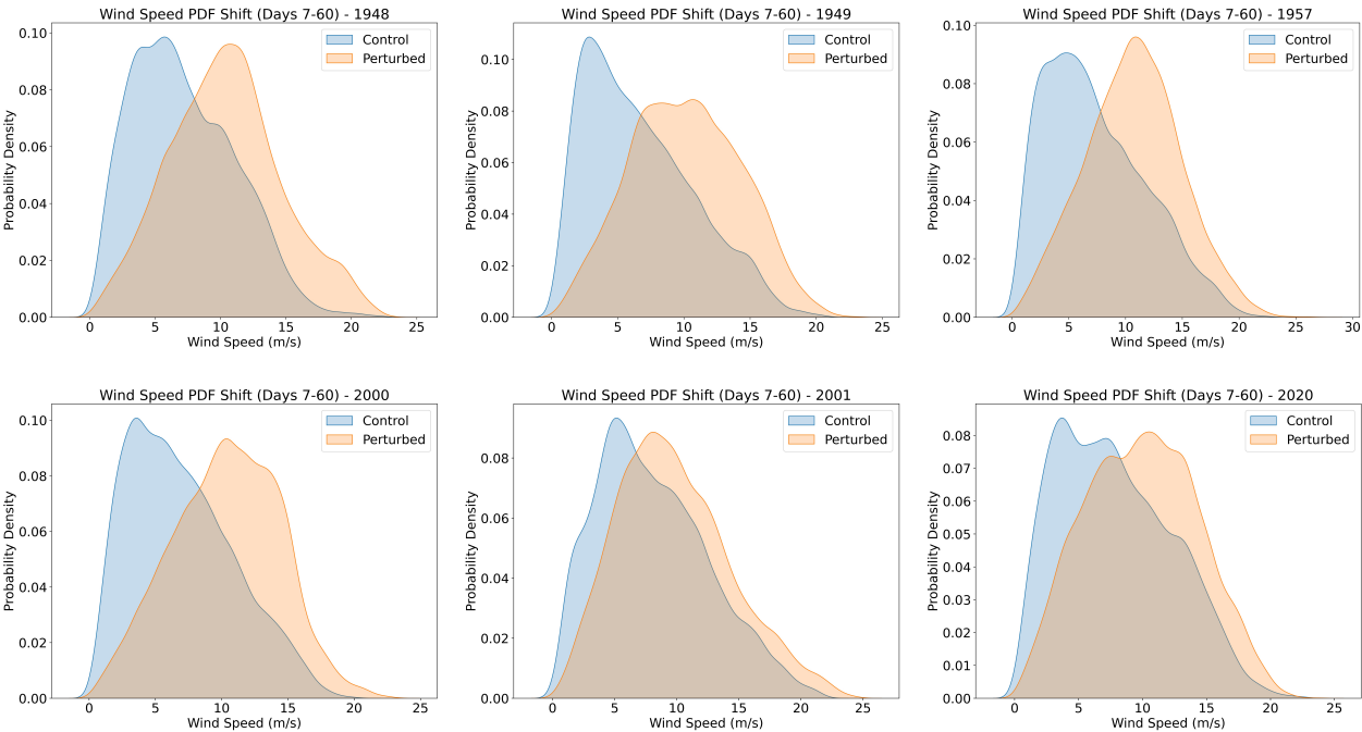
Figure 9. PDFs of daily wind speed over the North Sea (days 7–60) for control and perturbed simulations, aggregated across multiple grid cells (Longitude: 4°W to 10°E, Latitude: 51°N to 61°N). The perturbed experiment consistently shows a rightward shift and a more populated upper tail. The figure also includes quantifications of the difference at the 90 th percentile of the PDF distributions as a percentage.
