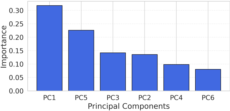
Figure 13. Importance of Principal Components Used as Predictors in the Random Forest Model
