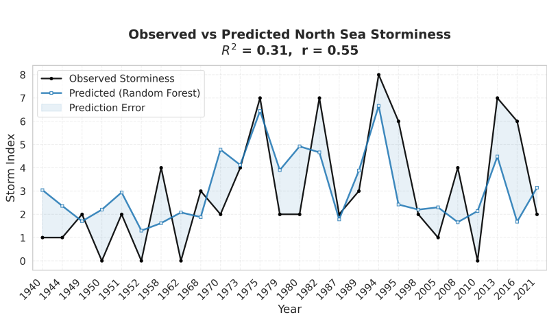
Figure 11. Comparison between observed and Random Forest predicted North Sea storminess (1940–2024). Time series of observed (black-test set) and predicted (blue) storm indices.
