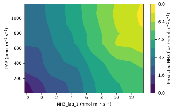
Figure 6. Partial dependence surface of predicted NH_3 flux as a function of NH_3 lag-1 and PAR under daytime conditions ( PAR > 0 ). Colors indicate predicted NH_3 flux ( nmol\ m^{-2}\ s^{-1} ) using the full value range of the model-predicted values for the daytime subset.
