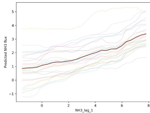
Figure 5. Individual Conditional Expectation (ICE) curves for NH_3\_lag\_1 under daytime conditions ( PAR > 0 ). Thin lines represent individual conditional responses, while the thick line shows the mean partial dependence.
