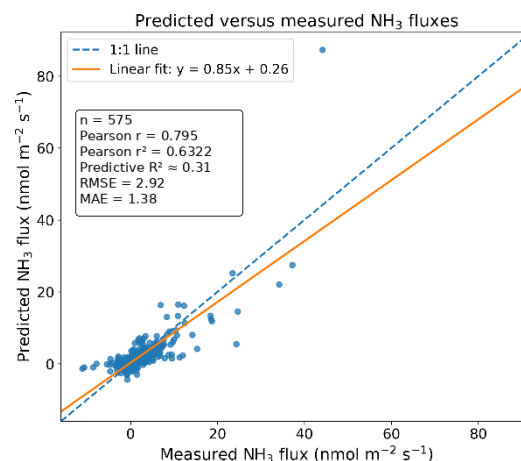
Figure 4. Comparison between measured and model-predicted \text{NH}_3 fluxes. The dashed line indicates the 1:1 relationship, and the solid line shows the linear regression fit.
