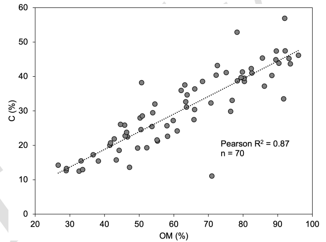
Figure 3. Relationship between organic matter content (%OM) and carbon content (%C) in Costa Rican peat.
