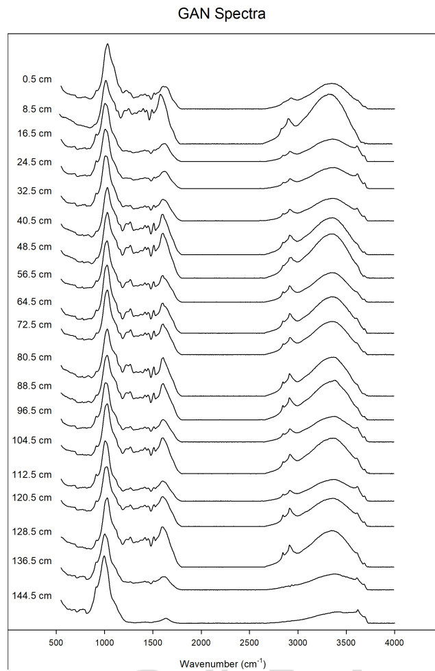
Figure A1. Stacked overlay of the FTIR spectra, Gandoca (GAN) core.
