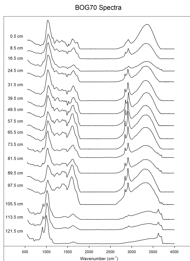
Figure A4. Stacked overlay of the FTIR spectra, BOG70 core.
