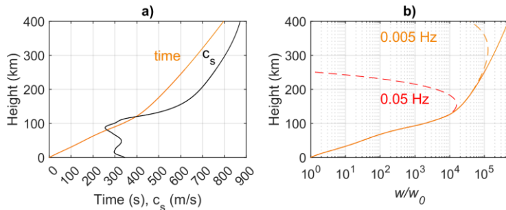
Fig. 5 a) Simulated infrasound propagation time (orange) and sound speed (black) as a function of height. b) Simulated vertical air particle oscillation velocities w normalized to the initial value w_0 above the ground surface for frequencies 0.05 Hz (red) and 0.005 Hz (orange). The solid orange line represents an idealized case of lossless propagation of a plane wave.
