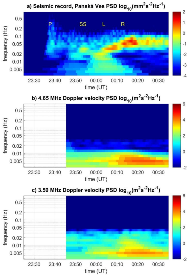
275 Fig. 3 Dynamic spectra (power spectral densities) of vertical velocity v_z of the ground surface motion on the night of July 29 to 30, 2025 (a), and of the Doppler shifts measured at f=4.65 MHz (b) and 3.59 MHz (c). The dynamic spectra correspond to signals presented in Figure 2.
