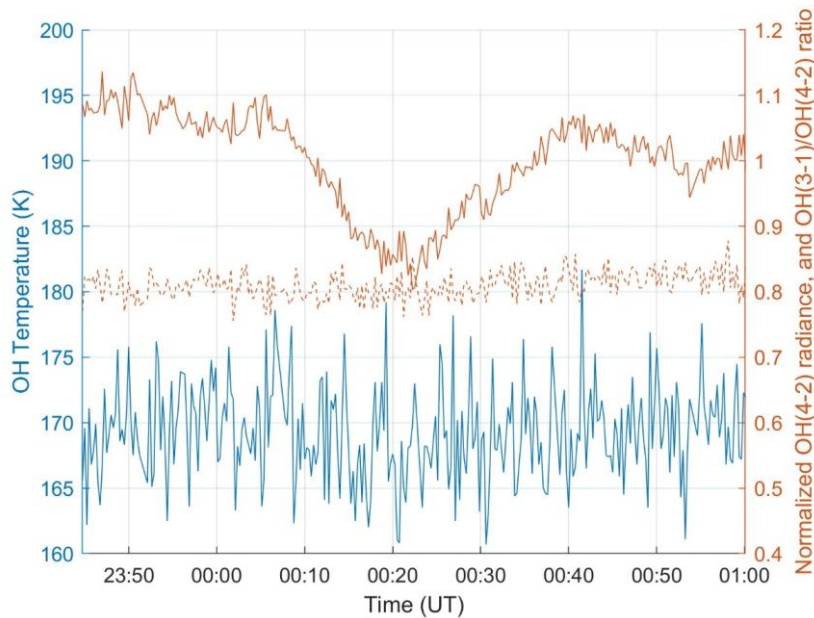
Fig. 7 OH temperature (blue) and OH(4-2) radiance (solid red) on the night of July 29 to 30, 2025. The nearly constant ratio (dashed red) between OH(3-1)- and OH(4-2)-emissions indicates a structure with large vertical wavelengths/scales being associated with the drop in intensity. See text for further details.
