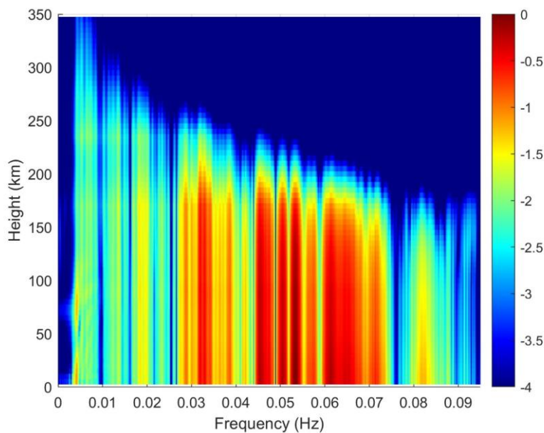
340 | Fig. 6 Expected power spectral densities (colour coded common logarithm) at different altitudes, normalized to the ground level.
