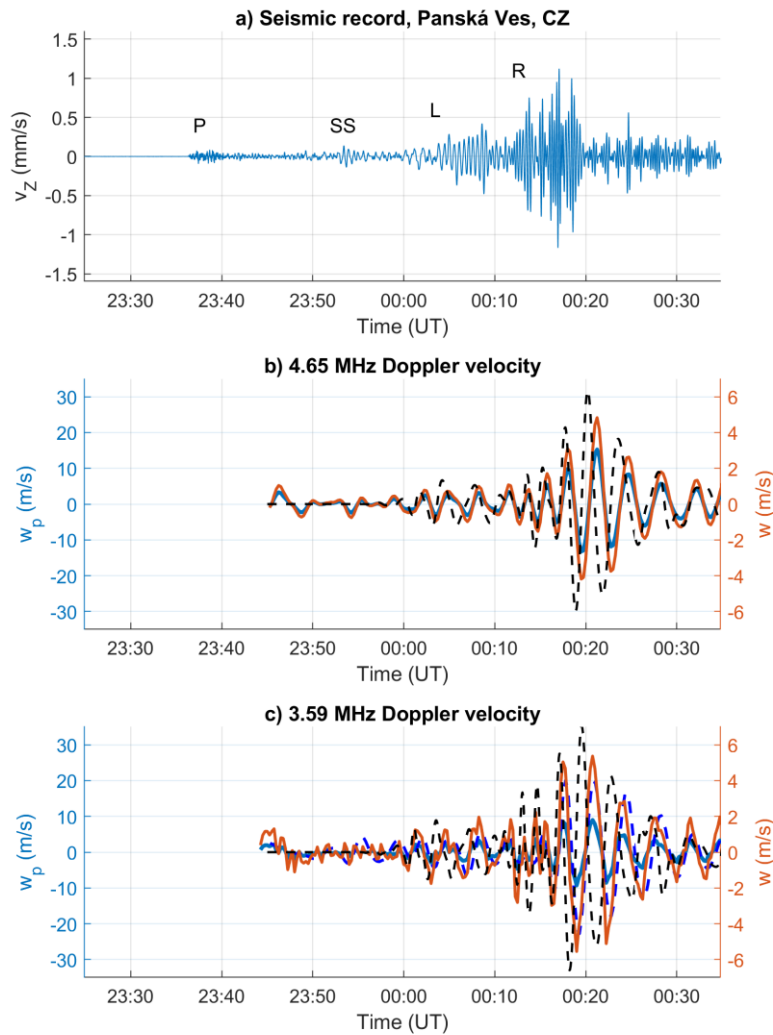
265 Fig. 2 a) Vertical velocity v_z of the ground surface motion in Panská Ves on the night of July 29 to 30, 2025 b) and c) Vertical velocity of plasma motion w_p (blue solid) directly obtained from the observed Doppler shift by equation (1) (blue) and the calculated vertical velocity of air particle oscillation w (red) obtained using equation (3) for measurements at f=4.65 and 3.59 MHz, respectively. Black dashed lines show the simulated vertical air particle oscillation
