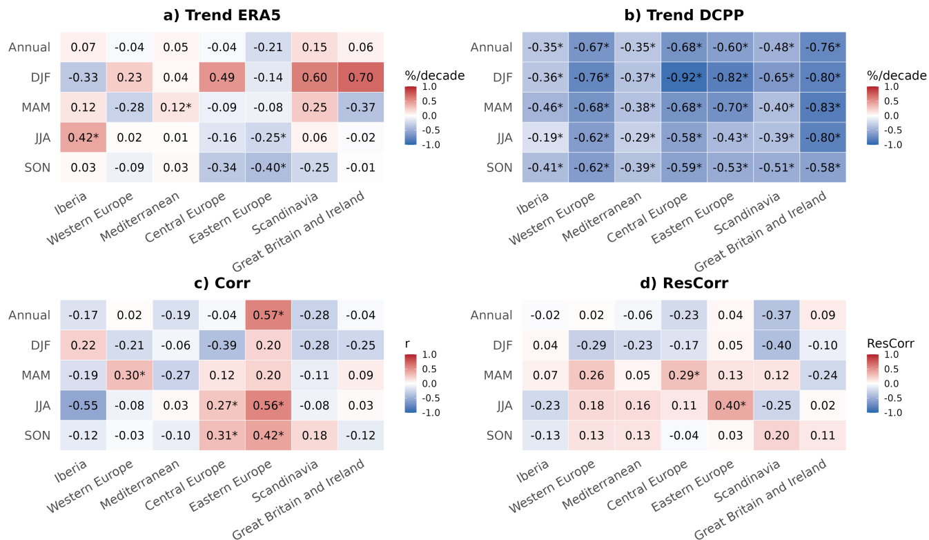
Figure 4. WCF trends derived from ERA5 for years 1961–2019 with 1961–2019 using a three years three-year rolling mean (a) and from the DCPP for the start dates 1960–2016 for 1960–2016 over forecast years 1–3 (b), the correlation between ERA5 and DCPP (c), and the ResCorr between DCPP and ERA5 respect relative to HIST (d), shown for the annual mean and for each season across the seven european European sub-regions (Figure S4). Statistically significant trends and , correlations and ResCorr values at the 95% confidence level are marked with an asterisk.
