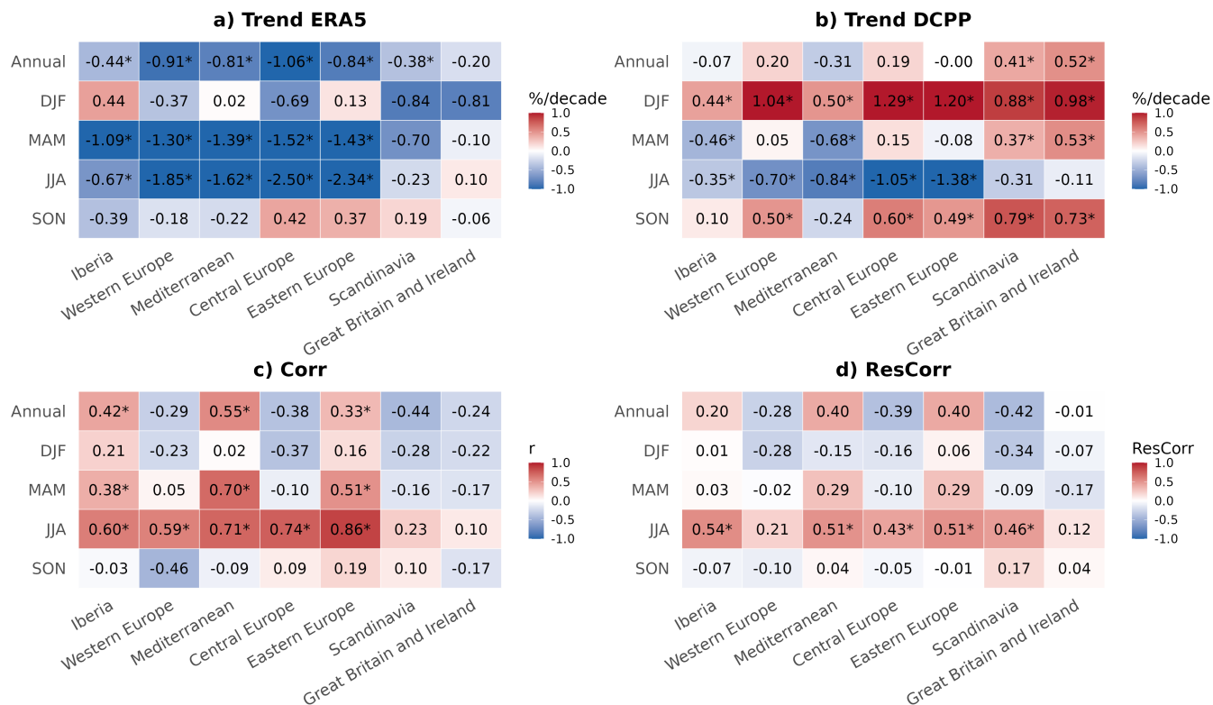
Figure 6. NED trends derived from ERA5 for years 1961–2019 with 1961–2019 using a three years three-year rolling mean (a) and from the DCPP for the start dates 1960–2016 for 1960–2016 over forecast years 1–3 (b), the correlation between ERA5 and DCPP (c), and the ResCorr between DCPP and ERA5 respect relative to HIST (d), shown for the annual mean and for each season across the seven european European sub-regions (Figure S4). Statistically significant trends and , correlations and ResCorr values at the 95% confidence level are marked with an asterisk.
