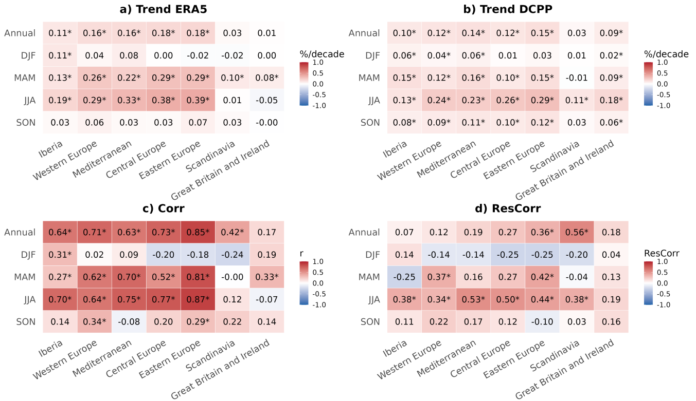
Figure 2. PVpot trends derived from ERA5 for years 1961–2019 with 1961–2019 using a three-years three-year rolling mean (a) and from the DCPP for the start dates 1960–2016 for 1960–2016 over forecast years 1–3 (b), the correlation between ERA5 and DCPP (c), and the ResCorr between DCPP and ERA5 respect relative to HIST (d), shown for the annual mean and for each season across the seven european European sub-regions (Figure S4). Statistically significant trends and , correlations and ResCorr values at the 95% confidence level are marked with an asterisk.
